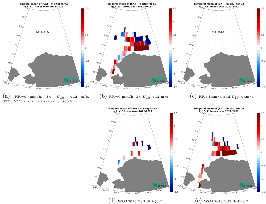
Figure 14: Temporal mean gridded over spatial boxes of size 1^\circ \times 1^\circ of \Delta SSS (SMAP SSS L3 v5.0 - Monthly (JPL) - SASSIE) for 5 different subdatasets corresponding to:RR=0 mm/h, 3 < U_{10} < 12 m/s, SST>5°C, distance to coast > 800 km (a), RR=0 mm/h, 3 < U_{10} < 12 m/s (b), RR>1mm/h and U_{10} < 4 m/s (c), WOA2013 SSS Std<0.2 (d), WOA2013 SSS Std>0.2 (e).
