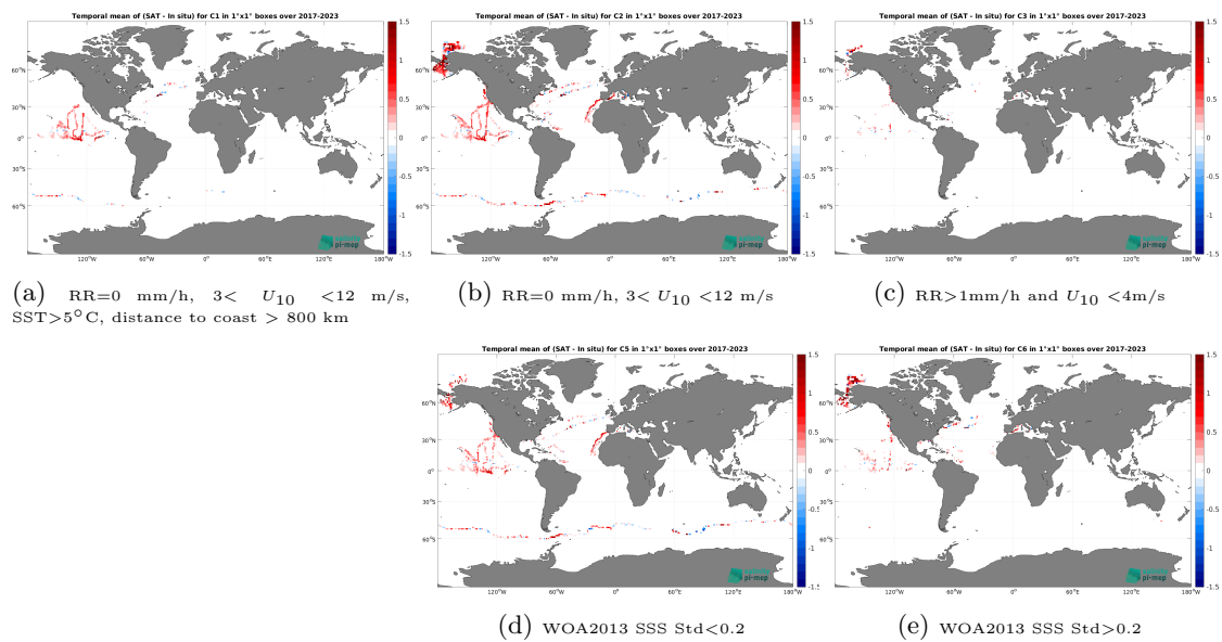
Figure 14: Temporal mean gridded over spatial boxes of size 1^\circ \times 1^\circ of \Delta SSS (SMAP SSS L3 v5.0 - Monthly (JPL) - Saifdrone) for 5 different subdatasets corresponding to:RR=0 mm/h, 3 < U_{10} < 12 m/s, SST > 5^\circ\text{C} , distance to coast > 800 km (a), RR=0 mm/h, 3 < U_{10} < 12 m/s (b), RR > 1 mm/h and U_{10} < 4 m/s (c), WOA2013 SSS Std < 0.2 (d), WOA2013 SSS Std > 0.2 (e).
