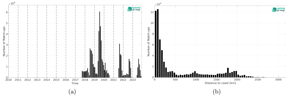
Figure 2: Number of match-ups between Sairdrone and SMAP SSS L3 v5.0 - Monthly (JPL) SSS as a function of time (a) and as function of the distance to coast (b) over the Global Ocean Pi-MEP region and for the full satellite product period.
