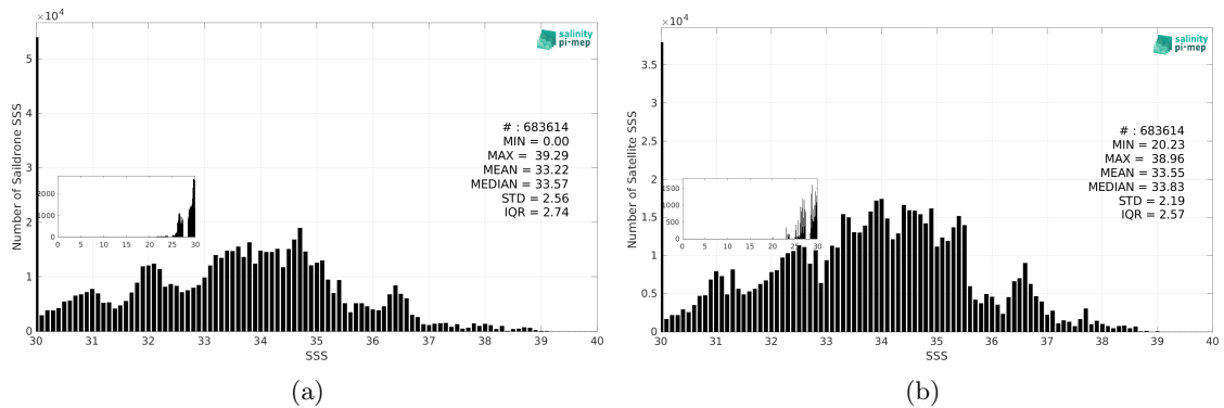
Figure 3: Histograms of SSS from Sairdrone (a) and SMAP SSS L3 v5.0 - Monthly (JPL) (b) considering all match-up pairs per bins of 0.1 over the Global Ocean Pi-MEP region and for the full satellite product period.
