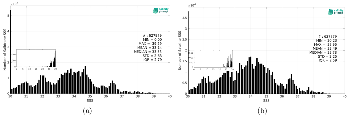
Figure 3: Histograms of SSS from Saildrone (a) and SMAP SSS L3 v5.0 - Monthly (JPL) (b) considering all match-up pairs per bins of 0.1 over the Global Ocean Pi-MEP region and for the full satellite product period.
