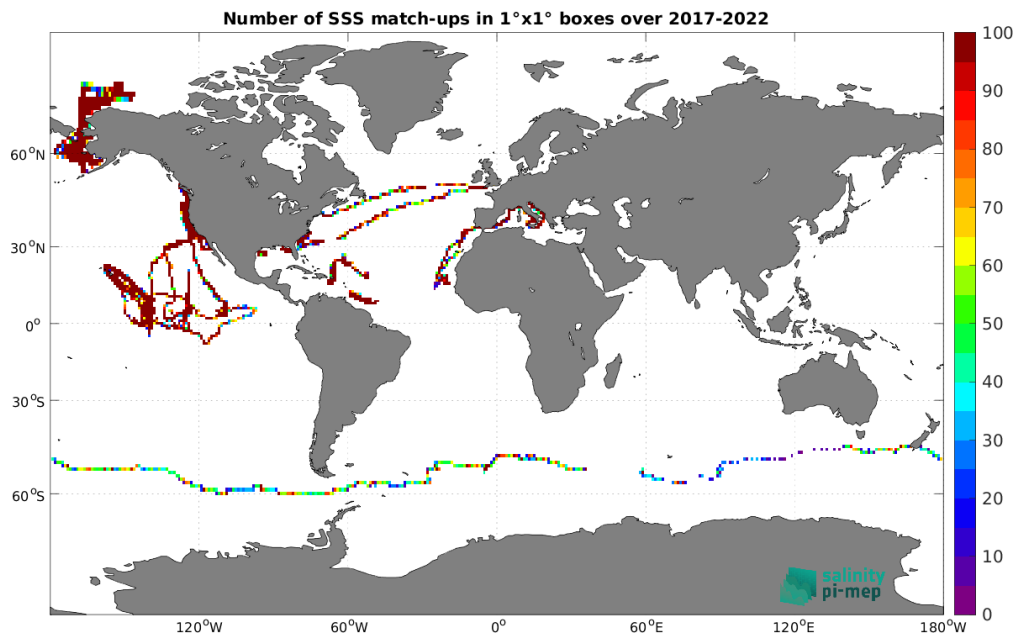
Figure 5: Number of SSS match-ups between Saildrone SSS and the SMAP SSS L3 v5.0 - Monthly (JPL) SSS product for the Global Ocean Pi-MEP region over 1^\circ \times 1^\circ boxes and for the full satellite product period.
