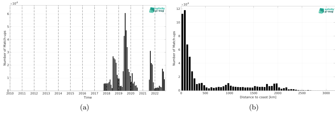
Figure 2: Number of match-ups between Saildrone and SMAP SSS L3 v5.0 - Monthly (JPL) SSS as a function of time (a) and as function of the distance to coast (b) over the Global Ocean Pi-MEP region and for the full satellite product period.
