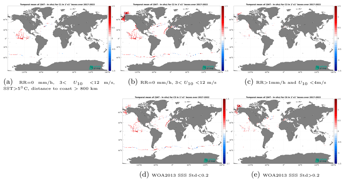
Figure 14: Temporal mean gridded over spatial boxes of size 1^\circ \times 1^\circ of \Delta SSS (SMAP SSS L3 v5.0 - Monthly (JPL) - Saikrone) for 5 different subdatasets corresponding to:RR=0 mm/h, 3 < U_{10} < 12 m/s, SST > 5^\circ\text{C} , distance to coast > 800 km (a), RR=0 mm/h, 3 < U_{10} < 12 m/s (b), RR > 1 mm/h and U_{10} < 4 m/s (c), WOA2013 SSS Std < 0.2 (d), WOA2013 SSS Std > 0.2 (e).
