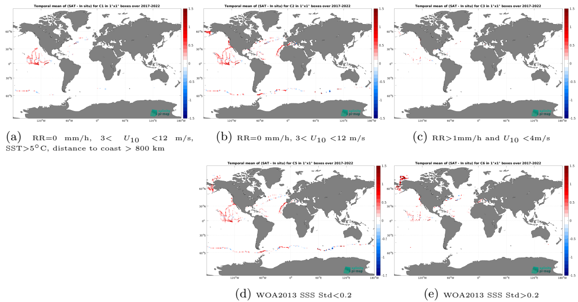
Figure 12: Temporal mean gridded over spatial boxes of size 1^\circ \times 1^\circ of \Delta SSS (SMAP SSS L3 v5.0 - Monthly (JPL) - Saifdrone) for 5 different subdatasets corresponding to:RR=0 mm/h, 3 < U_{10} < 12 m/s, SST > 5^\circ\text{C} , distance to coast > 800 km (a), RR=0 mm/h, 3 < U_{10} < 12 m/s (b), RR > 1 mm/h and U_{10} < 4 m/s (c), WOA2013 SSS Std < 0.2 (d), WOA2013 SSS Std > 0.2 (e).
