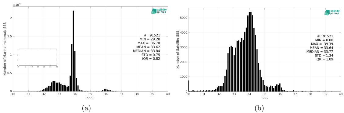
Figure 2: Histograms of SSS from Marine mammals (a) and SMAP SSS L3 v5.0 - Monthly (JPL) (b) considering all match-up pairs per bins of 0.1 over the Global Ocean Pi-MEP region and for the full satellite product period.
