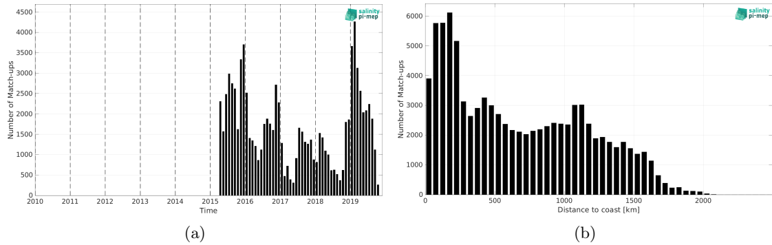
Figure 1: Number of match-ups between Marine mammals and SMAP SSS L3 v5.0 - Monthly (JPL) SSS as a function of time (a) and as function of the distance to coast (b) over the Global Ocean Pi-MEP region and for the full satellite product period.
