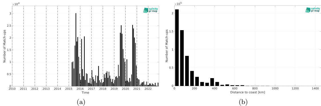
Figure 1: Number of match-ups between ICES and SMAP SSS L3 v5.0 - Monthly (JPL) SSS as a function of time (a) and as function of the distance to coast (b) over the Global Ocean Pi-MEP region and for the full satellite product period.
