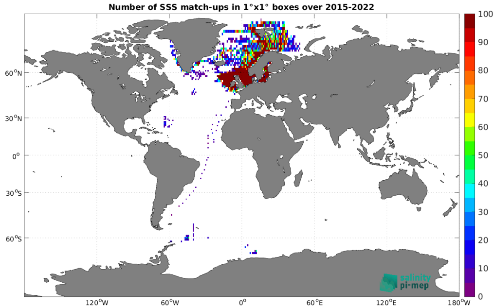
Figure 4: Number of SSS match-ups between ICES SSS and the SMAP SSS L3 v5.0 - Monthly (JPL) SSS product for the Global Ocean Pi-MEP region over 1^\circ \times 1^\circ boxes and for the full satellite product period.
