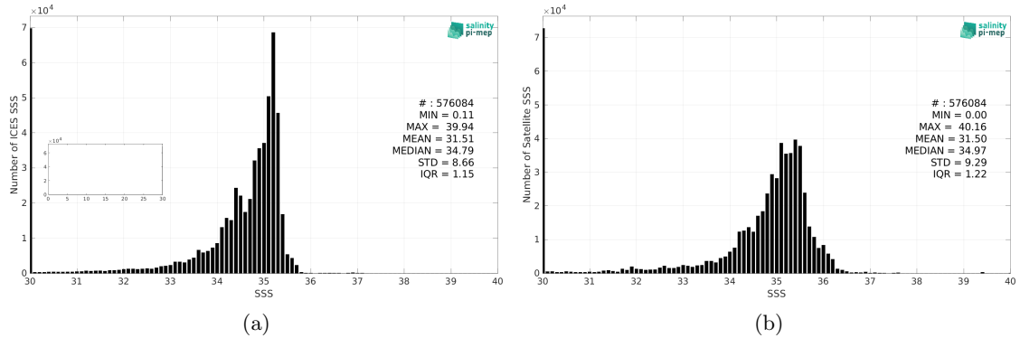
Figure 2: Histograms of SSS from ICES (a) and SMAP SSS L3 v5.0 - Monthly (JPL) (b) considering all match-up pairs per bins of 0.1 over the Global Ocean Pi-MEP region and for the full satellite product period.
