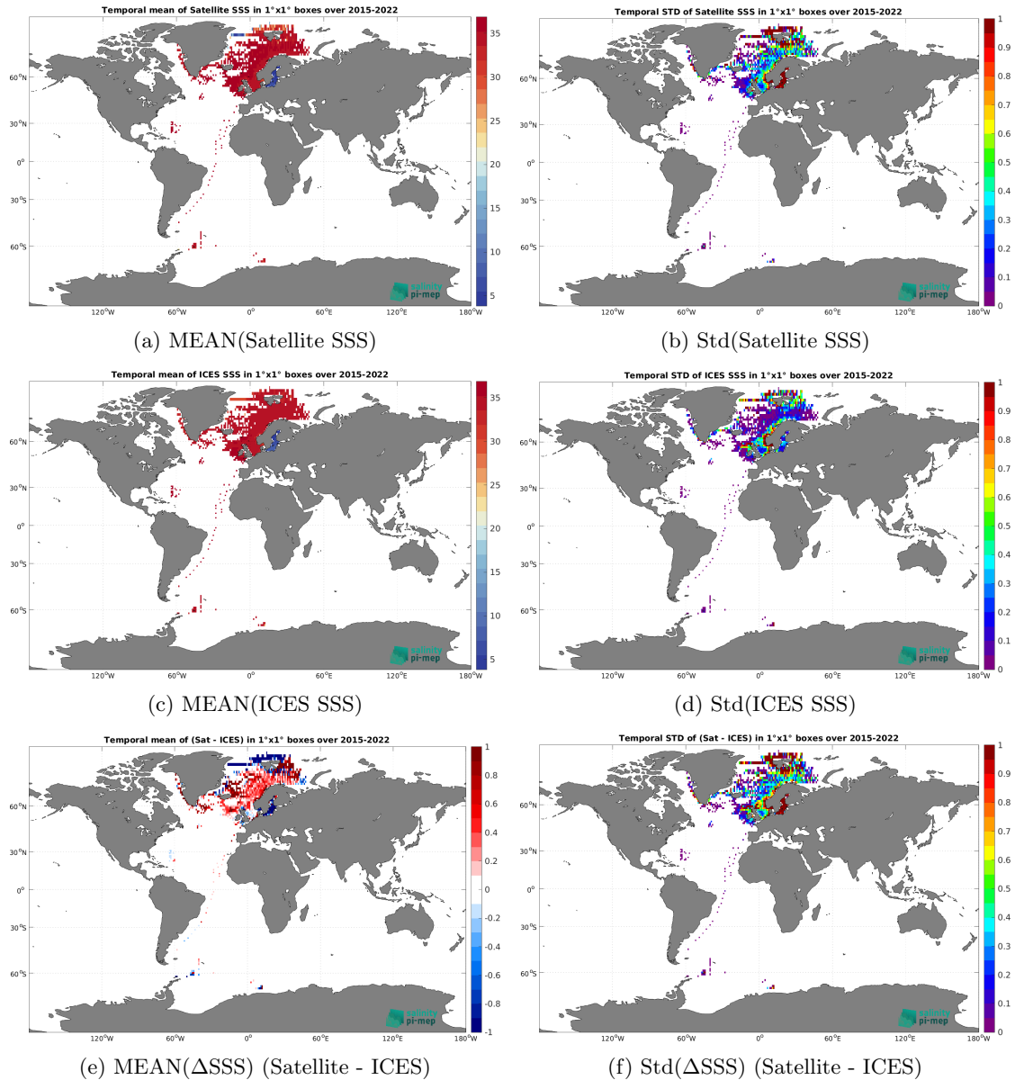
Figure 6: Temporal mean (left) and Std (right) of SSS from SMAP SSS L3 v5.0 - Monthly (JPL) (top), ICES (middle), and of \Delta SSS (Satellite - ICES). Only match-up pairs are used to generate these maps.
