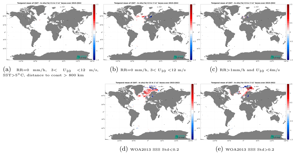
Figure 12: Temporal mean gridded over spatial boxes of size 1^\circ \times 1^\circ of \Delta\text{SSS} (SMAP SSS L3 v5.0 - Monthly (JPL) - ICES) for 5 different subdatasets corresponding to:RR=0 mm/h, 3 < U_{10} < 12 m/s, SST > 5^\circ\text{C} , distance to coast > 800 km (a), RR=0 mm/h, 3 < U_{10} < 12 m/s (b), RR > 1\text{mm/h} and U_{10} < 4\text{m/s} (c), WOA2013 SSS Std < 0.2 (d), WOA2013 SSS Std > 0.2 (e).
