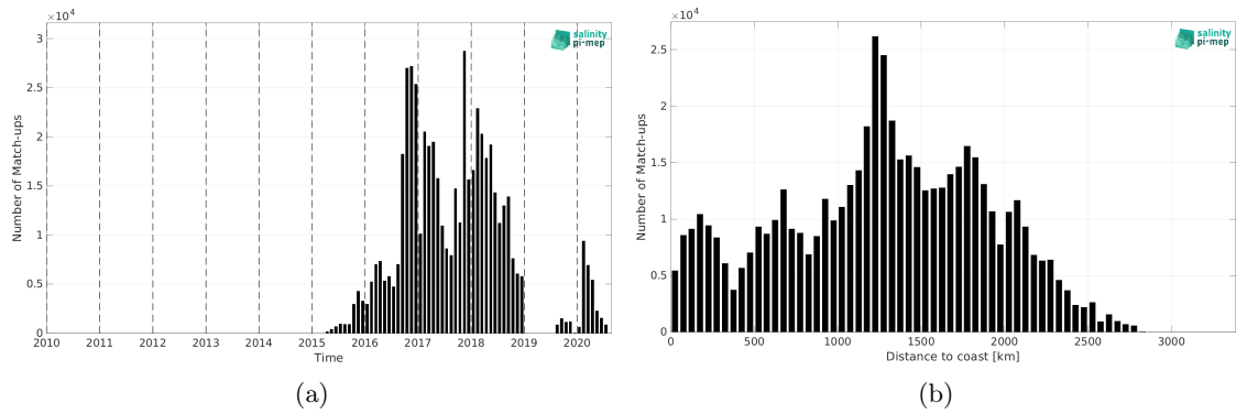
Figure 2: Number of match-ups between Surface drifters and SMAP SSS L3 v5.0 - Monthly (JPL) SSS as a function of time (a) and as function of the distance to coast (b) over the Global Ocean Pi-MEP region and for the full satellite product period.
