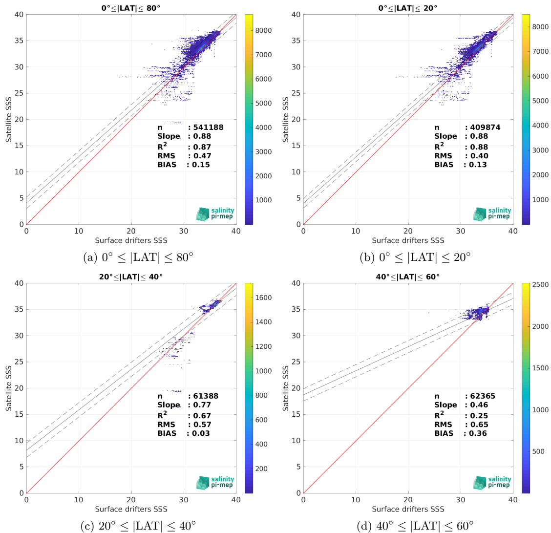
Figure 9: Contour maps of the concentration of SMAP SSS L3 v5.0 - Monthly (JPL) SSS (y-axis) versus Surface drifters SSS (x-axis) at match-up pairs for different latitude bands. For each plot, the red line shows x=y . The black thin and dashed lines indicate a linear fit through the data cloud and the \pm 95\% confidence levels, respectively. The number match-up pairs n , the slope and R^2 coefficient of the linear fit, the root mean square (RMS) and the mean bias between satellite and in situ data are indicated for each latitude band in each plots.
