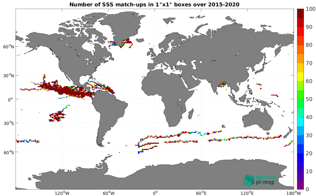
Figure 4: Number of SSS match-ups between Surface drifters SSS and the SMAP SSS L3 v5.0 - Monthly (JPL) SSS product for the Global Ocean Pi-MEP region over 1^\circ \times 1^\circ boxes and for the full satellite product period.
