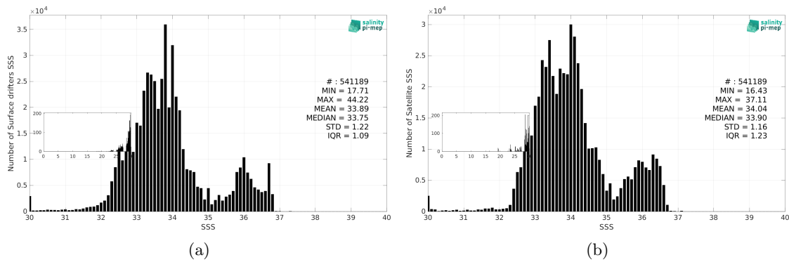
Figure 3: Histograms of SSS from Surface drifters (a) and SMAP SSS L3 v5.0 - Monthly (JPL) (b) considering all match-up pairs per bins of 0.1 over the Global Ocean Pi-MEP region and for the full satellite product period.
