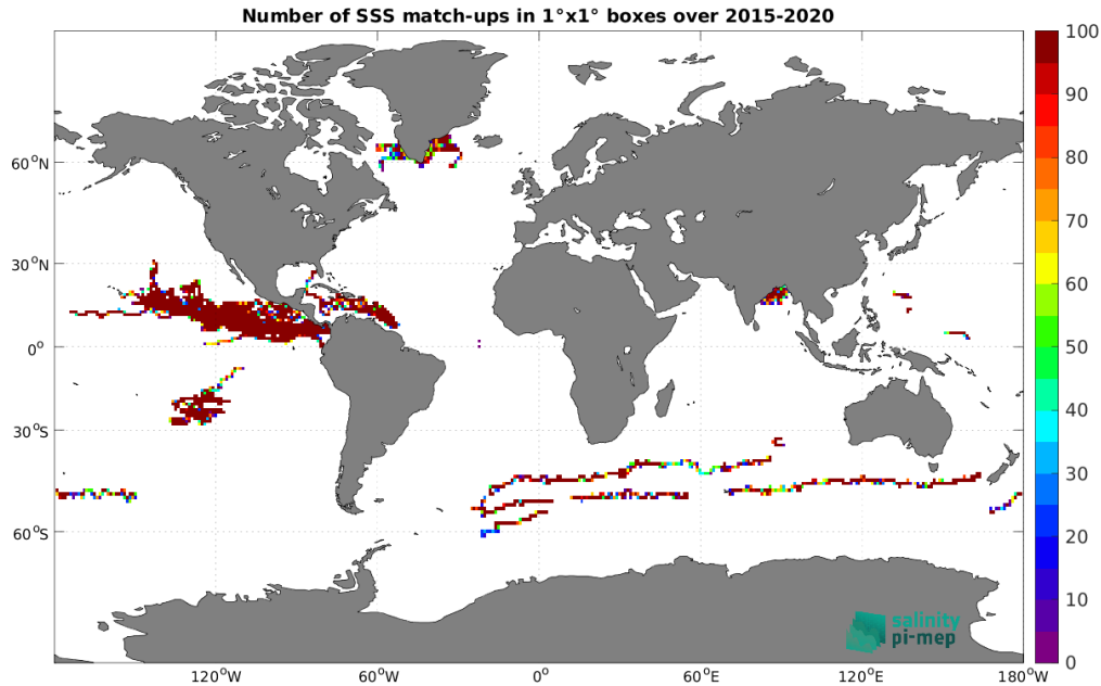
Figure 3: Number of SSS match-ups between Surface drifters SSS and the SMAP SSS L3 v5.0 - Monthly (JPL) SSS product for the Global Ocean Pi-MEP region over 1^\circ \times 1^\circ boxes and for the full satellite product period.
