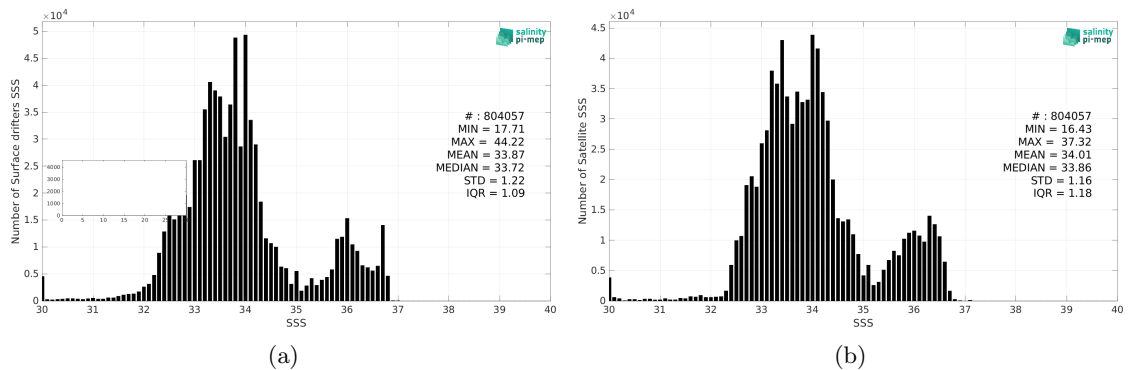
Figure 2: Histograms of SSS from Surface drifters (a) and SMAP SSS L3 v5.0 - Monthly (JPL) (b) considering all match-up pairs per bins of 0.1 over the Global Ocean Pi-MEP region and for the full satellite product period.
