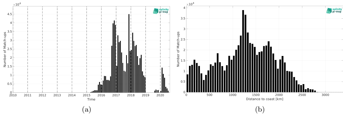
Figure 1: Number of match-ups between Surface drifters and SMAP SSS L3 v5.0 - Monthly (JPL) SSS as a function of time (a) and as function of the distance to coast (b) over the Global Ocean Pi-MEP region and for the full satellite product period.
