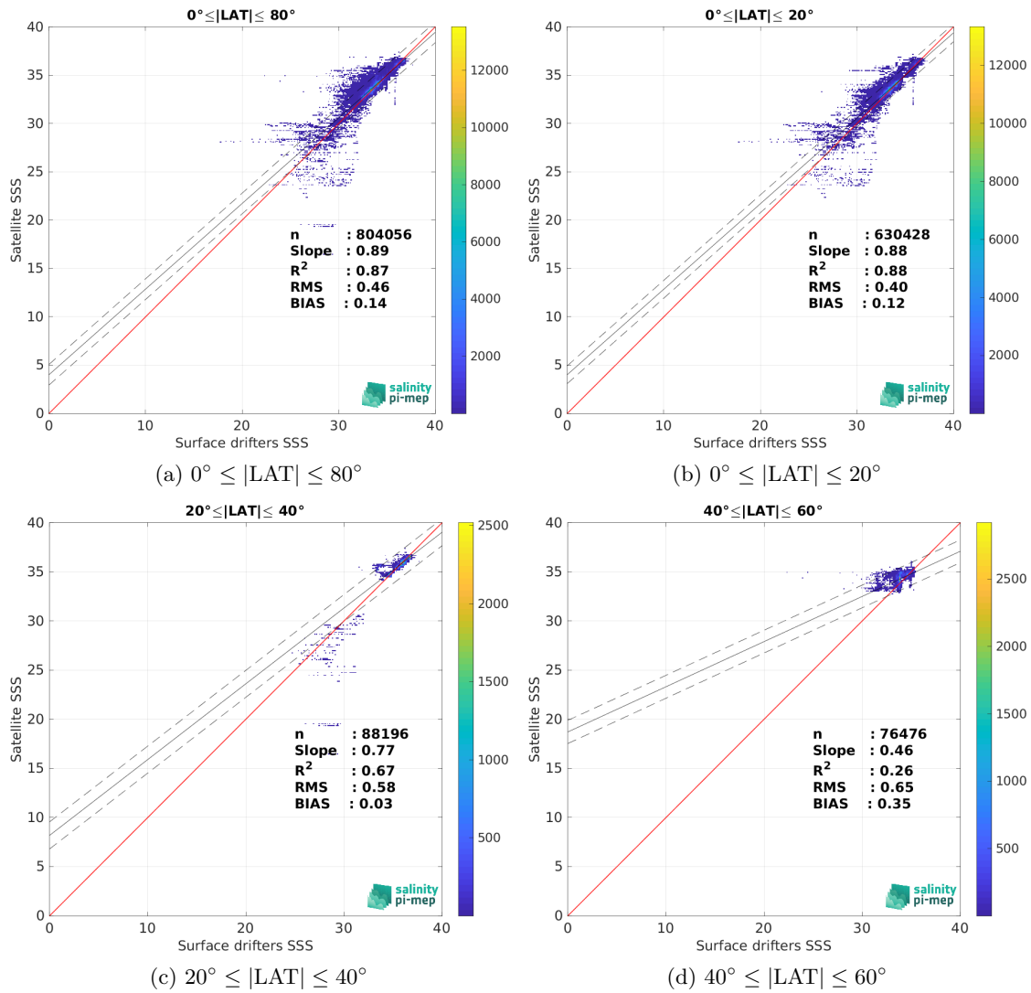
Figure 8: Contour maps of the concentration of SMAP SSS L3 v5.0 - Monthly (JPL) SSS (y-axis) versus Surface drifters SSS (x-axis) at match-up pairs for different latitude bands. For each plot, the red line shows x=y . The black thin and dashed lines indicate a linear fit through the data cloud and the \pm 95\% confidence levels, respectively. The number match-up pairs n , the slope and R^2 coefficient of the linear fit, the root mean square (RMS) and the mean bias between satellite and in situ data are indicated for each latitude band in each plots.
