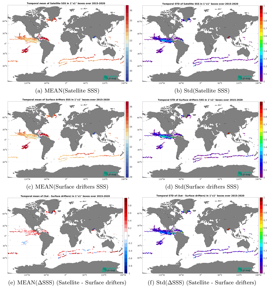
Figure 5: Temporal mean (left) and Std (right) of SSS from SMAP SSS L3 v5.0 - Monthly (JPL) (top), Surface drifters (middle), and of \Delta SSS (Satellite - Surface drifters). Only match-up pairs are used to generate these maps.
