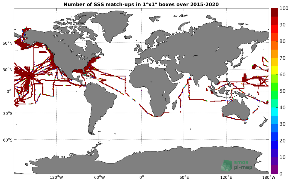
Figure 4: Number of SSS match-ups between TSG-SAMOS SSS and the SMAP-L3-JPL-V4.3-8DAY-RUNNING-60KM SSS product for the Global Ocean Pi-MEP region over 1^\circ \times 1^\circ boxes and for the full satellite product period.
