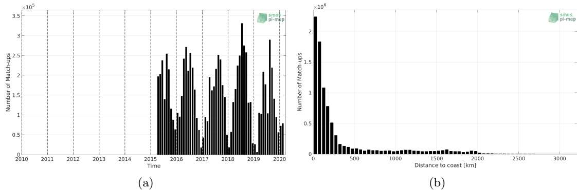
Figure 1: Number of match-ups between TSG-SAMOS and SMAP-L3-JPL-V4.3-8DAY-RUNNING-60KM SSS as a function of time (a) and as function of the distance to coast (b) over the Global Ocean Pi-MEP region and for the full satellite product period.
