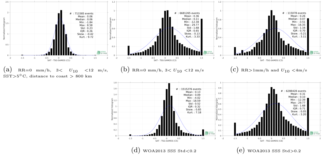
Figure 13: Normalized histogram of \Delta\text{SSS} (SMAP-L3-JPL-V4.3-8DAY-RUNNING-60KM - TSG-SAMOS) for 5 different subdatasets corresponding to: RR=0 mm/h, 3 < U_{10} < 12 m/s, SST >5^{\circ}\text{C} , distance to coast > 800 km (a), RR=0 mm/h, 3 < U_{10} < 12 m/s (b), RR >1 mm/h and U_{10} < 4 m/s (c), WOA2013 SSS Std <0.2 (d), WOA2013 SSS Std >0.2 (e).
