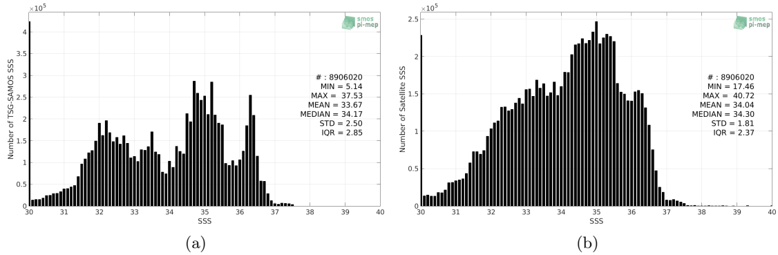
Figure 2: Histograms of SSS from TSG-SAMOS (a) and SMAP-L3-JPL-V4.3-8DAY-RUNNING-60KM (b) considering all match-up pairs per bins of 0.1 over the Global Ocean Pi-MEP region and for the full satellite product period.
