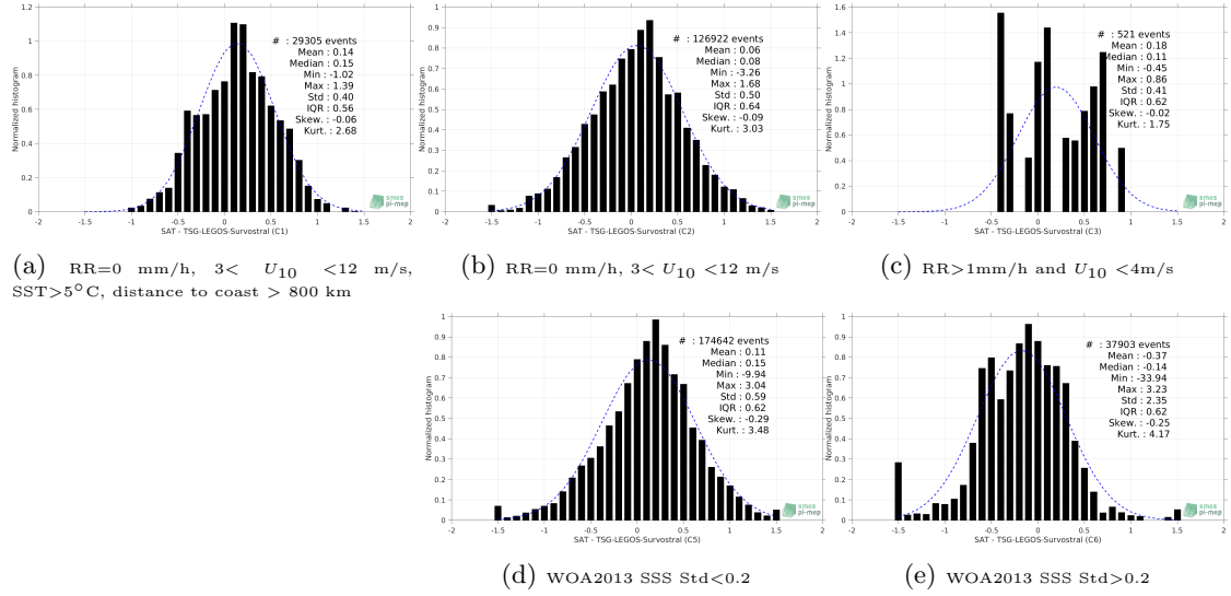
Figure 13: Normalized histogram of \Delta SSS (SMAP-L3-JPL-V4.3-8DAY-RUNNING-60KM - TSG-LEGOS-Survostral) for 5 different subdatasets corresponding to: RR=0 mm/h, 3 < U_{10} < 12 m/s, SST>5°C, distance to coast > 800 km (a), RR=0 mm/h, 3 < U_{10} < 12 m/s (b), RR>1mm/h and U_{10} < 4 m/s (c), WOA2013 SSS Std<0.2 (d), WOA2013 SSS Std>0.2 (e).
