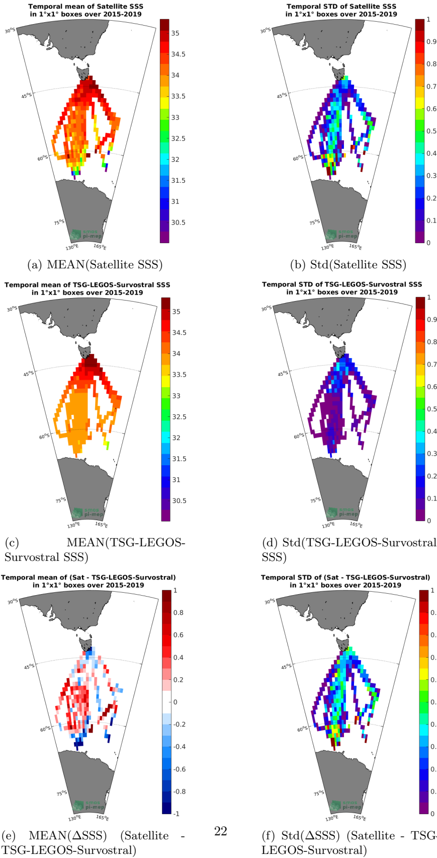
Figure 6: Temporal mean (left) and Std (right) of SSS from SMAP-L3-JPL-V4.3-8DAY-RUNNING-60KM (top), TSG-LEGOS-Survostral (middle), and of \Delta SSS (Satellite - TSG-LEGOS-Survostral). Only match-up pairs are used to generate these maps.
