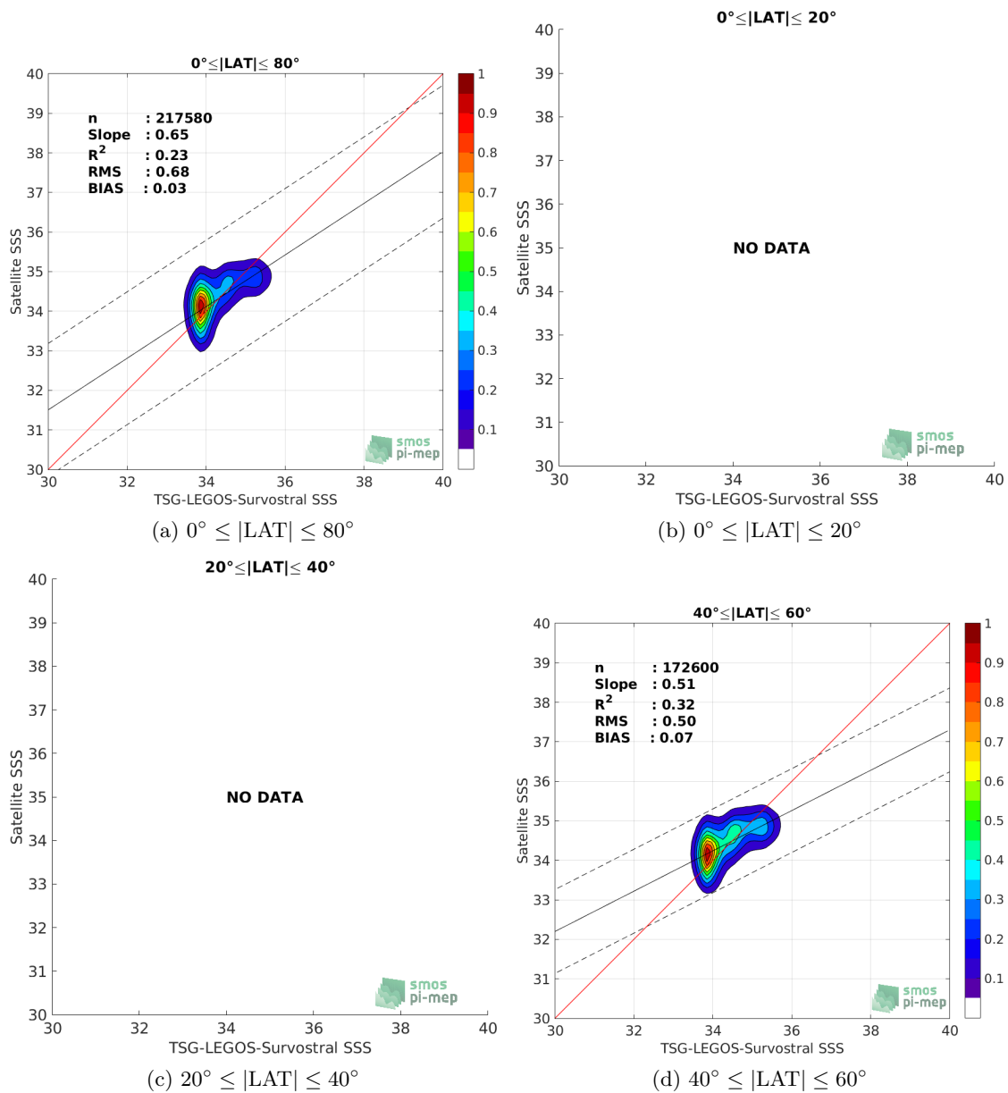
Figure 9: Contour maps of the concentration of SMAP-L3-JPL-V4.3-8DAY-RUNNING-60KM SSS (y-axis) versus TSG-LEGOS-Survostral SSS (x-axis) at match-up pairs for different latitude bands. For each plot, the red line shows x=y . The black thin and dashed lines indicate a linear fit through the data cloud and the \pm 95\% confidence levels, respectively. The number match-up pairs n , the slope and R^2 coefficient of the linear fit, the root mean square (RMS) and the mean bias between satellite and in situ data are indicated for each latitude band in each plots.
