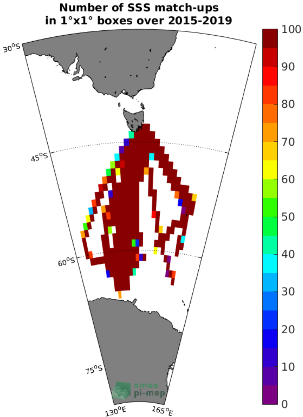
Figure 4: Number of SSS match-ups between TSG-LEGOS-Survostral SSS and the SMAP-L3-JPL-V4.3-8DAY-RUNNING-60KM SSS product for the Global Ocean Pi-MEP region over 1°x1° boxes and for the full satellite product period.
