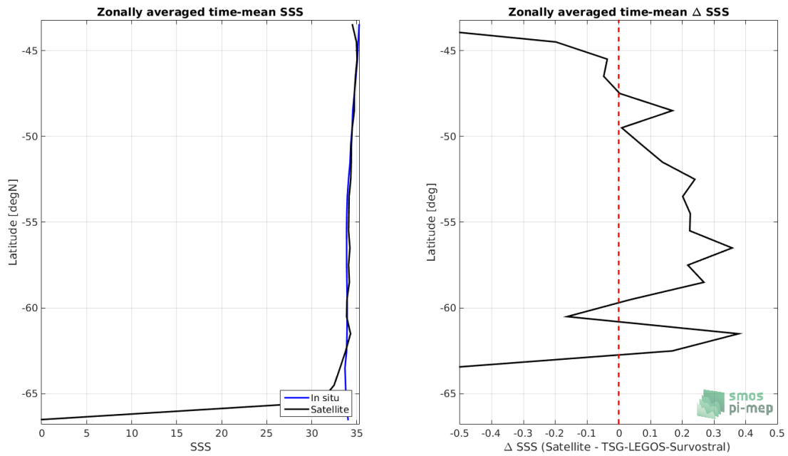
Figure 8: Left panel: Zonal mean SSS from SMAP-L3-JPL-V4.3-8DAY-RUNNING-60KM satellite product (black) and from TSG-LEGOS-Survostral (blue). Right panel: Zonal mean of \Delta SSS (Satellite - TSG-LEGOS-Survostral) for all the collected Pi-MEP match-up pairs estimated over the full satellite product period.
