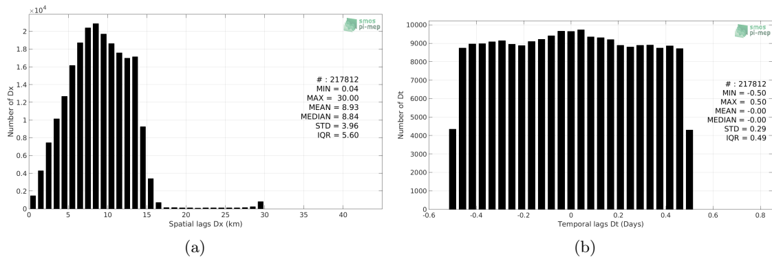
Figure 5: Histograms of the spatial (a) and temporal (b) lags between the time of the TSG-LEGOS-Survostral measurements and the date of the corresponding SMAP-L3-JPL-V4.3-8DAY-RUNNING-60KM SSS product.
