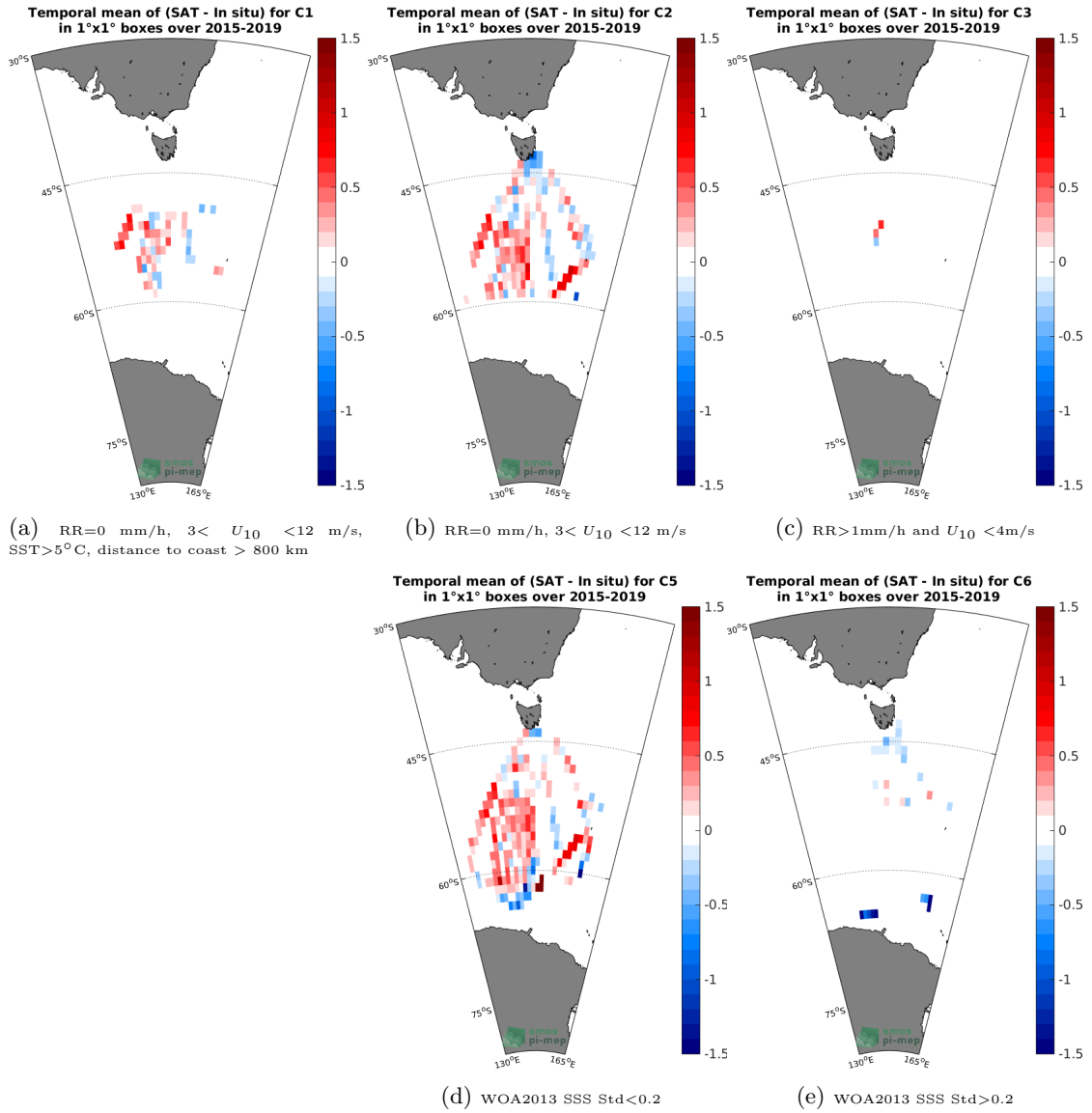
Figure 12: Temporal mean gridded over spatial boxes of size 1°x1° of \Delta SSS (SMAP-L3-JPL-V4.3-8DAY-RUNNING-60KM - TSG-LEGOS-Survostral) for 5 different subdatasets corresponding to:RR=0 mm/h, 3 < U_{10} < 12 m/s, SST>5°C, distance to coast > 800 km (a), RR=0 mm/h, 3 < U_{10} < 12 m/s (b), RR>1mm/h and U_{10} < 4 m/s (c), WOA2013 SSS Std<0.2 (d), WOA2013 SSS Std>0.2 (e).
