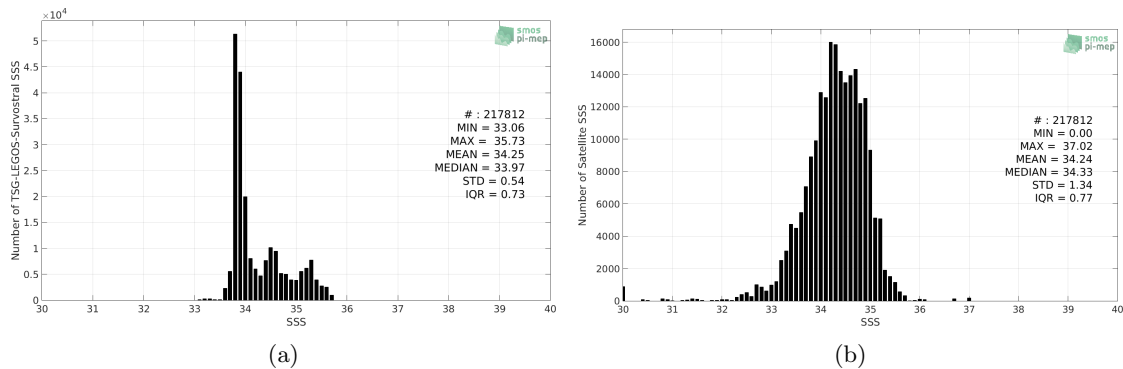
Figure 2: Histograms of SSS from TSG-LEGOS-Survostral (a) and SMAP-L3-JPL-V4.3-8DAY-RUNNING-60KM (b) considering all match-up pairs per bins of 0.1 over the Global Ocean Pi-MEP region and for the full satellite product period.
