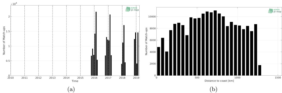
Figure 1: Number of match-ups between TSG-LEGOS-Survostral and SMAP-L3-JPL-V4.3-8DAY-RUNNING-60KM SSS as a function of time (a) and as function of the distance to coast (b) over the Global Ocean Pi-MEP region and for the full satellite product period.
