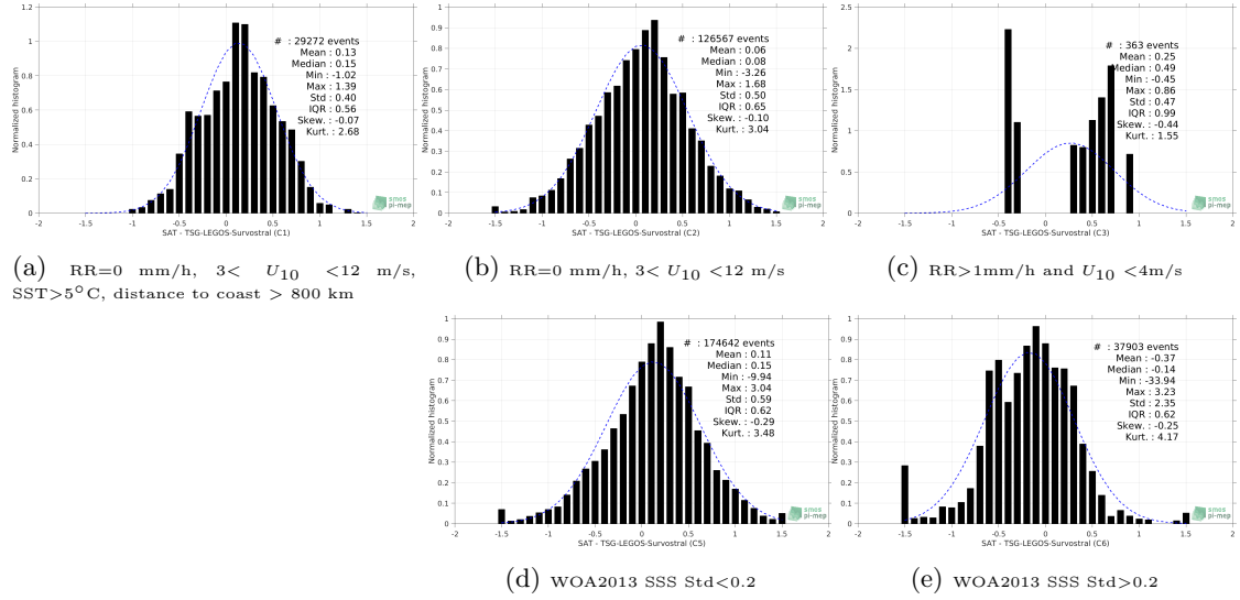
Figure 13: Normalized histogram of \Delta SSS (SMAP-L3-JPL-V4.3-8DAY-RUNNING-60KM - TSG-LEGOS-Survostral) for 5 different subdatasets corresponding to: RR=0 mm/h, 3 < U_{10} < 12 m/s, SST > 5°C, distance to coast > 800 km (a), RR=0 mm/h, 3 < U_{10} < 12 m/s (b), RR > 1mm/h and U_{10} < 4 m/s (c), WOA2013 SSS Std < 0.2 (d), WOA2013 SSS Std > 0.2 (e).
