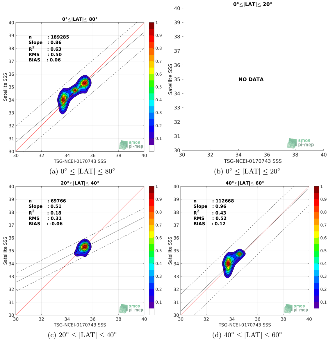
Figure 9: Contour maps of the concentration of SMAP-L3-JPL-V4.3-MONTHLY-60KM SSS (y-axis) versus TSG-NCEI-0170743 SSS (x-axis) at match-up pairs for different latitude bands. For each plot, the red line shows x=y . The black thin and dashed lines indicate a linear fit through the data cloud and the \pm 95\% confidence levels, respectively. The number match-up pairs n , the slope and R^2 coefficient of the linear fit, the root mean square (RMS) and the mean bias between satellite and in situ data are indicated for each latitude band in each plots.
