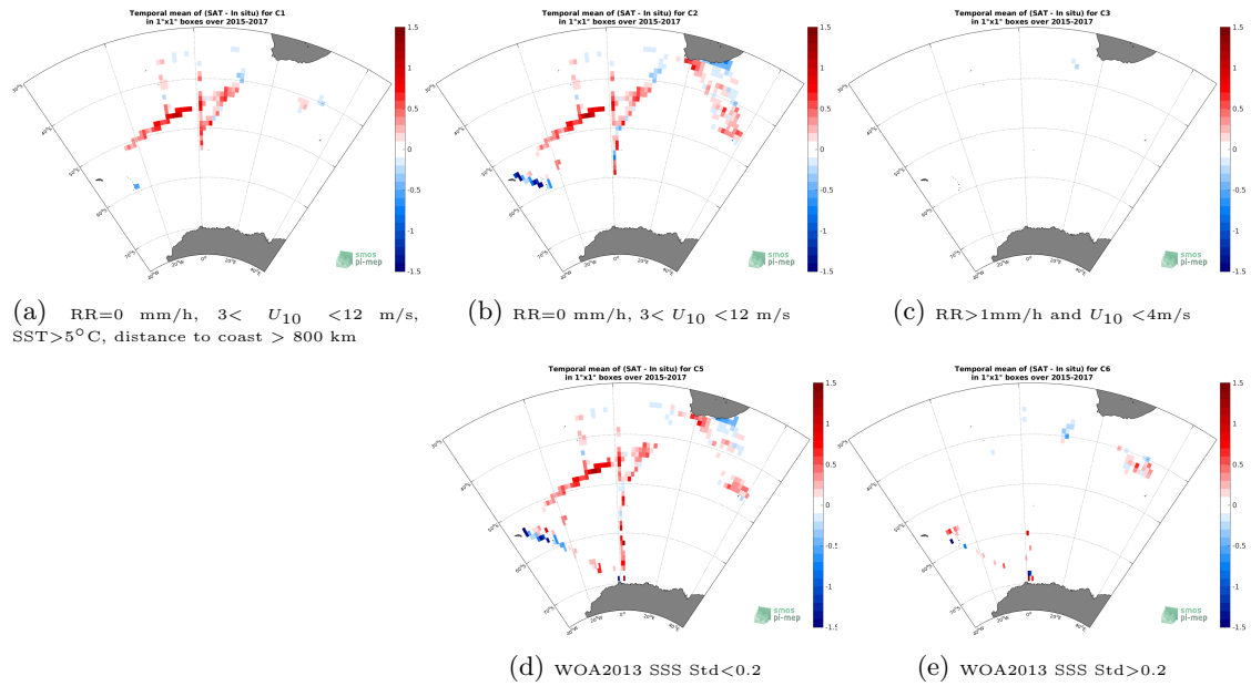
Figure 12: Temporal mean gridded over spatial boxes of size 1^\circ \times 1^\circ of \Delta SSS (SMAP-L3-JPL-V4.3-MONTHLY-60KM - TSG-NCEI-0170743) for 5 different subdatasets corresponding to:RR=0 mm/h, 3 < U_{10} < 12 m/s, SST >5^\circ C, distance to coast > 800 km (a), RR=0 mm/h, 3 < U_{10} < 12 m/s (b), RR >1 mm/h and U_{10} < 4 m/s (c), WOA2013 SSS Std <0.2 (d), WOA2013 SSS Std >0.2 (e).
