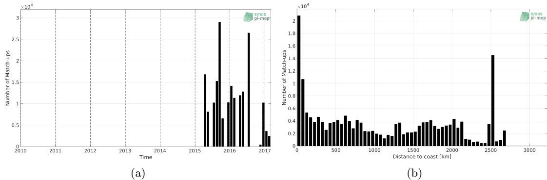
Figure 1: Number of match-ups between TSG-NCEI-0170743 and SMAP-L3-JPL-V4.3-MONTHLY-60KM SSS as a function of time (a) and as function of the distance to coast (b) over the Global Ocean Pi-MEP region and for the full satellite product period.
