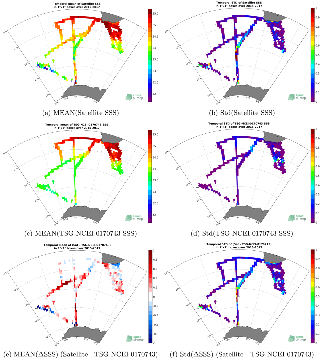
Figure 6: Temporal mean (left) and Std (right) of SSS from SMAP-L3-JPL-V4.3-MONTHLY-60KM (top), TSG-NCEI-0170743 (middle), and of \Delta SSS (Satellite - TSG-NCEI-0170743). Only match-up pairs are used to generate these maps.
