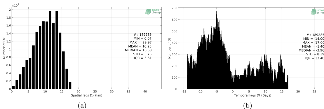
Figure 5: Histograms of the spatial (a) and temporal (b) lags between the time of the TSG-NCEI-0170743 measurements and the date of the corresponding SMAP-L3-JPL-V4.3-MONTHLY-60KM SSS product.
