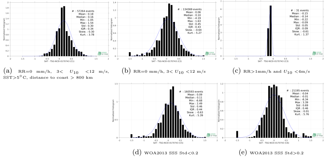
Figure 13: Normalized histogram of \Delta\text{SSS} (SMAP-L3-JPL-V4.3-MONTHLY-60KM - TSG-NCEI-0170743) for 5 different subdatasets corresponding to: RR=0 mm/h, 3 < U_{10} < 12 m/s, SST > 5^{\circ}\text{C} , distance to coast > 800 km (a), RR=0 mm/h, 3 < U_{10} < 12 m/s (b), RR > 1 mm/h and U_{10} < 4 m/s (c), WOA2013 SSS Std <0.2 (d), WOA2013 SSS Std >0.2 (e).
