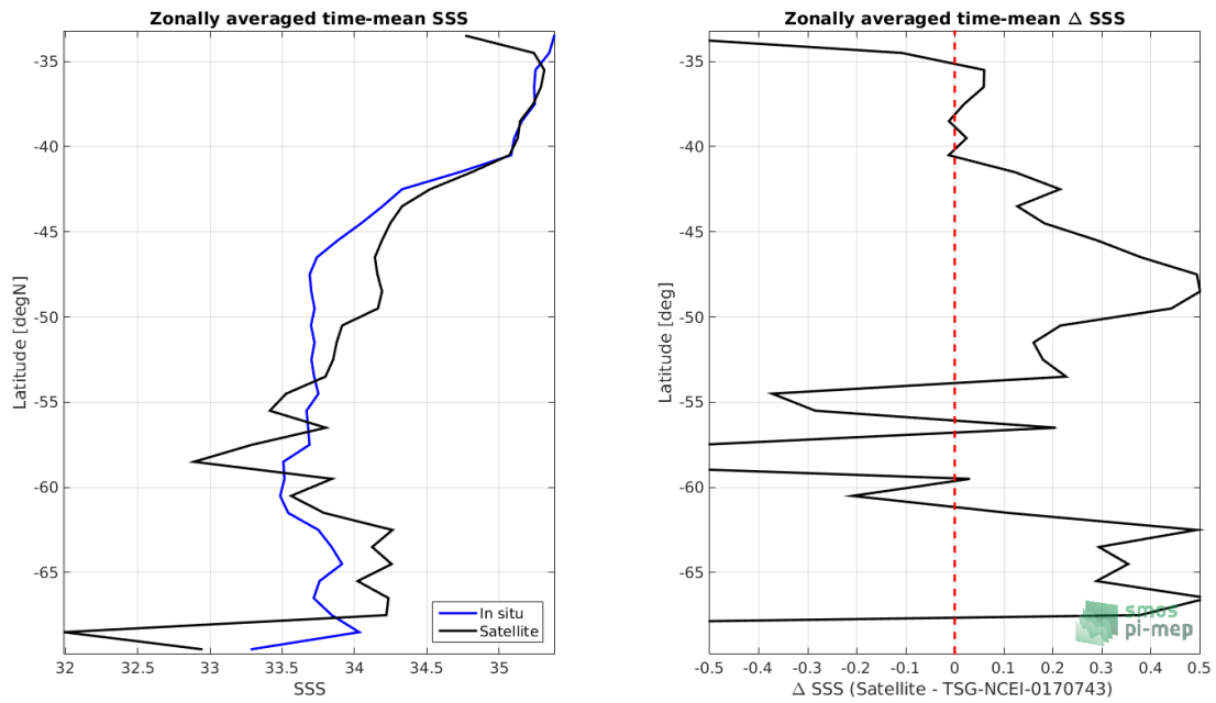
Figure 8: Left panel: Zonal mean SSS from SMAP-L3-JPL-V4.3-MONTHLY-60KM satellite product (black) and from TSG-NCEI-0170743 (blue). Right panel: Zonal mean of \Delta SSS (Satellite - TSG-NCEI-0170743) for all the collected Pi-MEP match-up pairs estimated over the full satellite product period.
