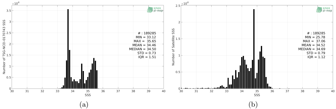
Figure 2: Histograms of SSS from TSG-NCEI-0170743 (a) and SMAP-L3-JPL-V4.3-MONTHLY-60KM (b) considering all match-up pairs per bins of 0.1 over the Global Ocean Pi-MEP region and for the full satellite product period.
