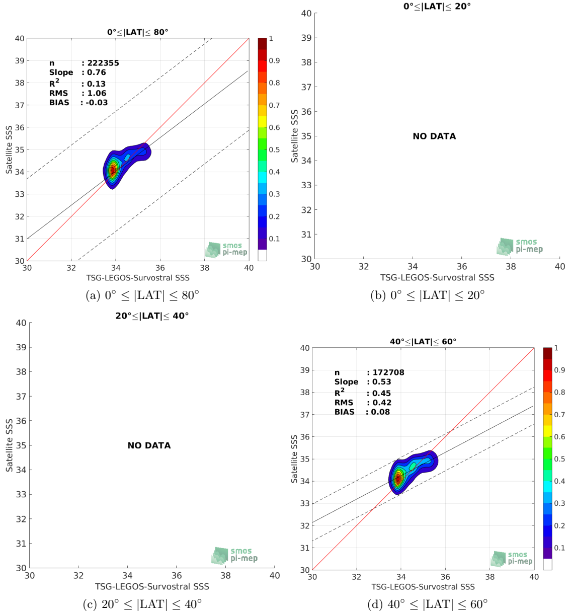
Figure 9: Contour maps of the concentration of SMAP-L3-JPL-V4.3-MONTHLY-60KM SSS (y-axis) versus TSG-LEGOS-Survostral SSS (x-axis) at match-up pairs for different latitude bands. For each plot, the red line shows x=y . The black thin and dashed lines indicate a linear fit through the data cloud and the \pm 95\% confidence levels, respectively. The number match-up pairs n , the slope and R^2 coefficient of the linear fit, the root mean square (RMS) and the mean bias between satellite and in situ data are indicated for each latitude band in each plots.
