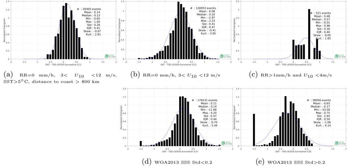
Figure 13: Normalized histogram of \Delta SSS (SMAP-L3-JPL-V4.3-MONTHLY-60KM - TSG-LEGOS-Survostral) for 5 different subdatasets corresponding to: RR=0 mm/h, 3 < U_{10} < 12 m/s, SST>5°C, distance to coast > 800 km (a), RR=0 mm/h, 3 < U_{10} < 12 m/s (b), RR>1mm/h and U_{10} < 4 m/s (c), WOA2013 SSS Std<0.2 (d), WOA2013 SSS Std>0.2 (e).
