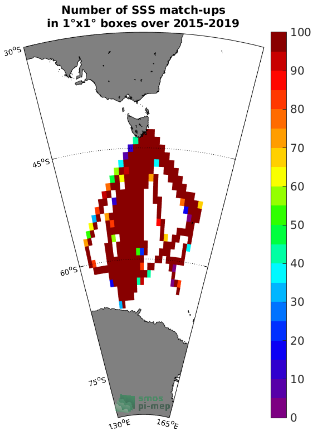
Figure 4: Number of SSS match-ups between TSG-LEGOS-Survostral SSS and the SMAP-L3-JPL-V4.3-MONTHLY-60KM SSS product for the Global Ocean Pi-MEP region over 1°x1° boxes and for the full satellite product period.
