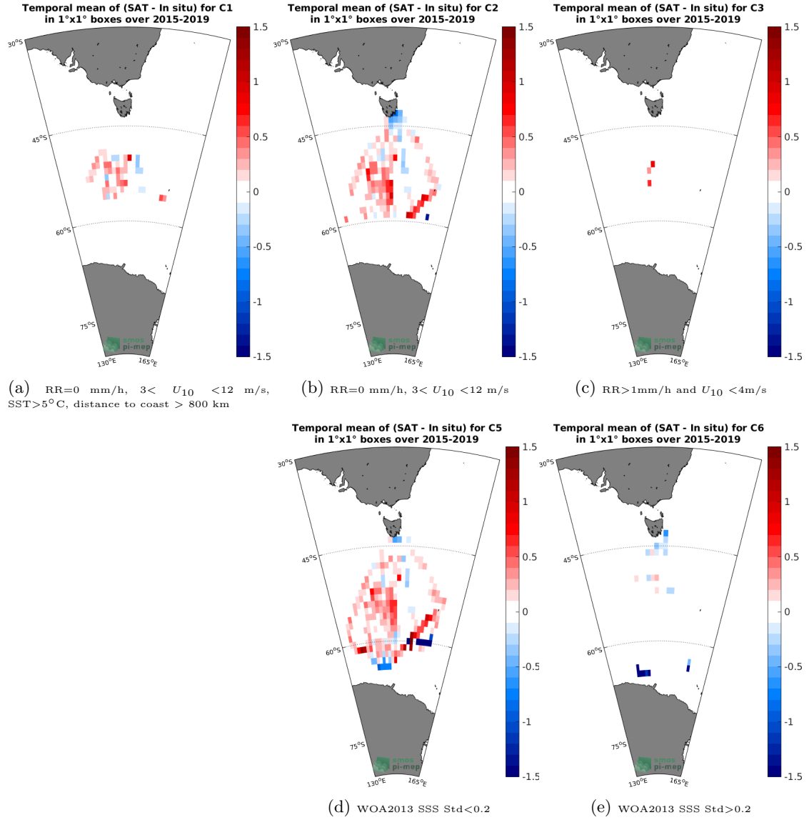
Figure 12: Temporal mean gridded over spatial boxes of size 1°x1° of \Delta\text{SSS} (SMAP-L3-JPL-V4.3-MONTHLY-60KM - TSG-LEGOS-Survostral) for 5 different subdatasets corresponding to: RR=0 mm/h, 3 < U_{10} < 12 m/s, SST > 5^{\circ}\text{C} , distance to coast > 800 km (a), RR=0 mm/h, 3 < U_{10} < 12 m/s (b), RR > 1\text{mm/h} and U_{10} < 4\text{m/s} (c), WOA2013 SSS Std < 0.2 (d), WOA2013 SSS Std > 0.2 (e).
