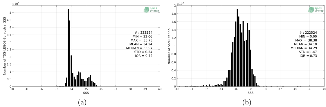
Figure 2: Histograms of SSS from TSG-LEGOS-Survostral (a) and SMAP-L3-JPL-V4.3-MONTHLY-60KM (b) considering all match-up pairs per bins of 0.1 over the Global Ocean Pi-MEP region and for the full satellite product period.
