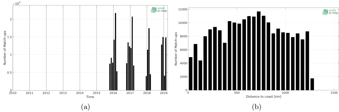
Figure 1: Number of match-ups between TSG-LEGOS-Survostral and SMAP-L3-JPL-V4.3-MONTHLY-60KM SSS as a function of time (a) and as function of the distance to coast (b) over the Global Ocean Pi-MEP region and for the full satellite product period.
