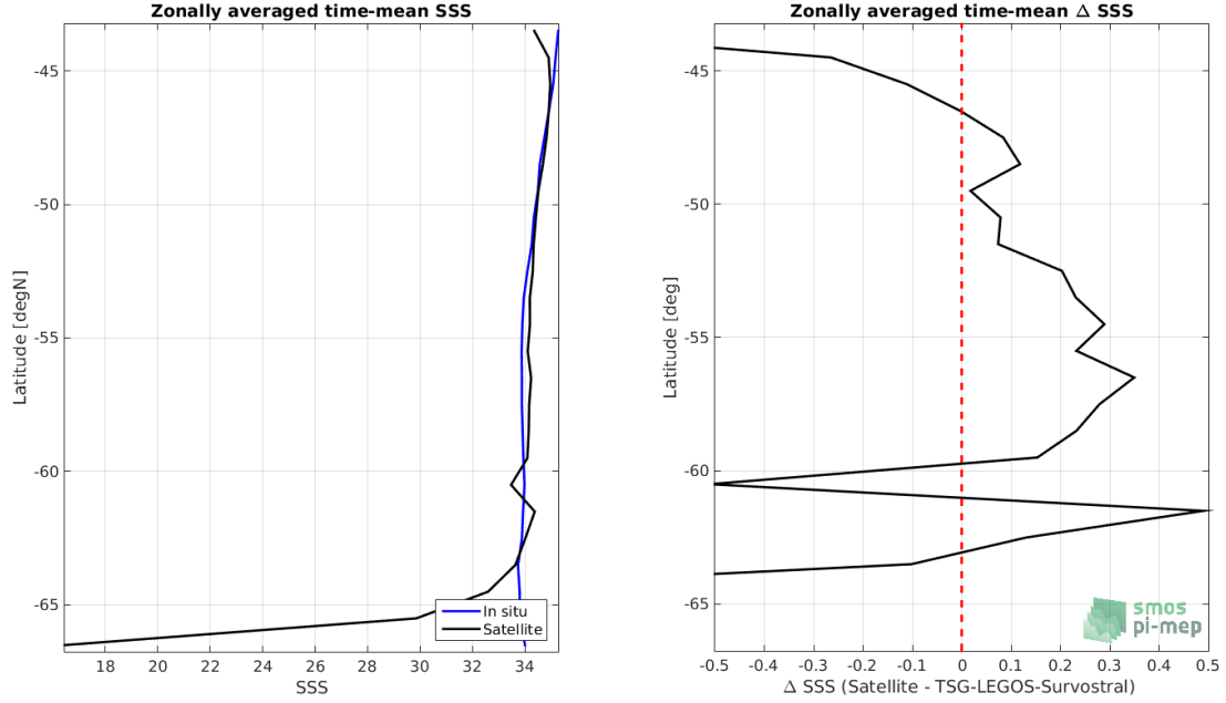
Figure 8: Left panel: Zonal mean SSS from SMAP-L3-JPL-V4.3-MONTHLY-60KM satellite product (black) and from TSG-LEGOS-Survostral (blue). Right panel: Zonal mean of \Delta SSS (Satellite - TSG-LEGOS-Survostral) for all the collected Pi-MEP match-up pairs estimated over the full satellite product period.
