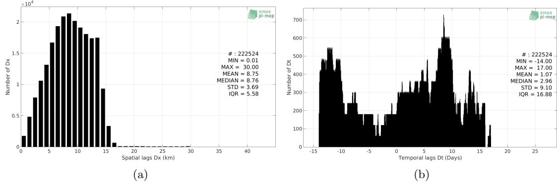
Figure 5: Histograms of the spatial (a) and temporal (b) lags between the time of the TSG-LEGOS-Survostral measurements and the date of the corresponding SMAP-L3-JPL-V4.3-MONTHLY-60KM SSS product.
