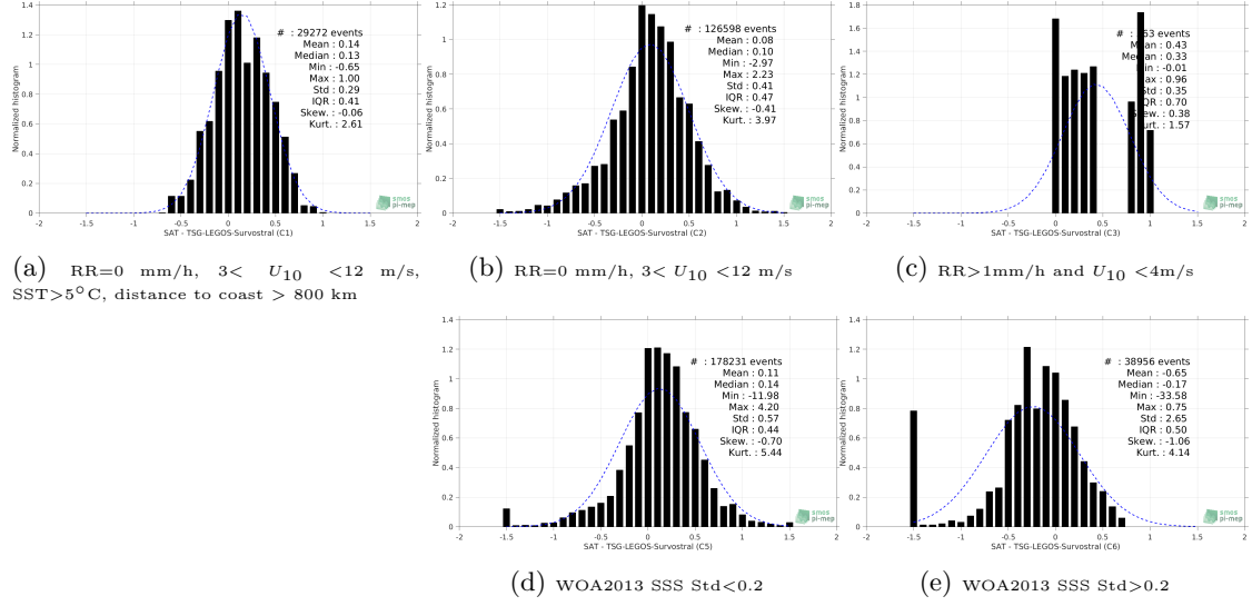
Figure 13: Normalized histogram of \Delta SSS (SMAP-L3-JPL-V4.3-MONTHLY-60KM - TSG-LEGOS-Survostral) for 5 different subdatasets corresponding to: RR=0 mm/h, 3 < U_{10} < 12 m/s, SST > 5°C, distance to coast > 800 km (a), RR=0 mm/h, 3 < U_{10} < 12 m/s (b), RR > 1 mm/h and U_{10} < 4 m/s (c), WOA2013 SSS Std < 0.2 (d), WOA2013 SSS Std > 0.2 (e).
