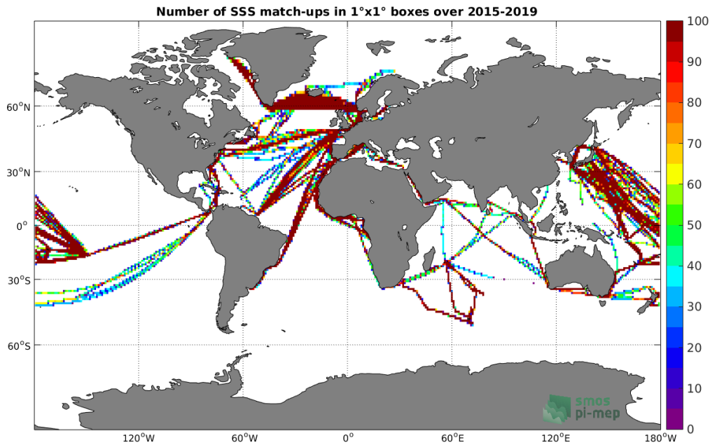
Figure 4: Number of SSS match-ups between TSG-LEGOS-DM SSS and the SMAP-L3-JPL-V4.3-MONTHLY-60KM SSS product for the Global Ocean Pi-MEP region over 1^\circ \times 1^\circ boxes and for the full satellite product period.
