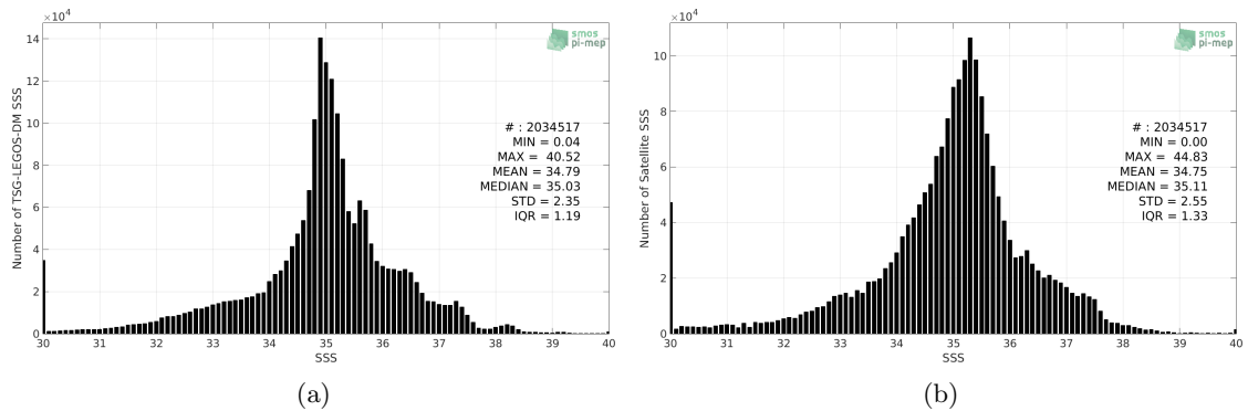
Figure 2: Histograms of SSS from TSG-LEGOS-DM (a) and SMAP-L3-JPL-V4.3-MONTHLY-60KM (b) considering all match-up pairs per bins of 0.1 over the Global Ocean Pi-MEP region and for the full satellite product period.
