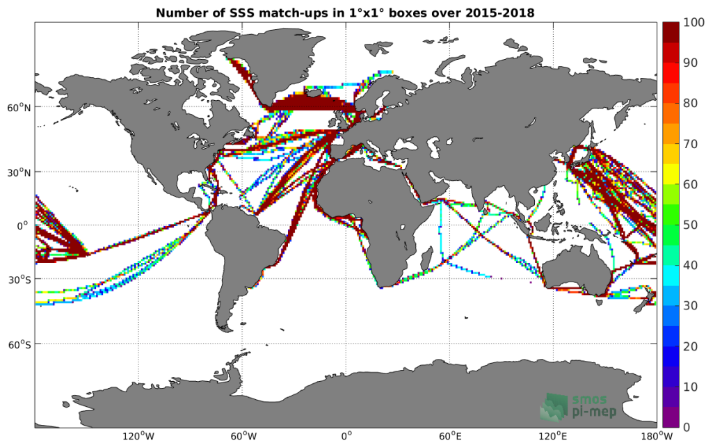
Figure 4: Number of SSS match-ups between TSG-LEGOS-DM SSS and the SMAP-L3-JPL-V4.3-MONTHLY-60KM SSS product for the Global Ocean Pi-MEP region over 1°x1° boxes and for the full satellite product period.
