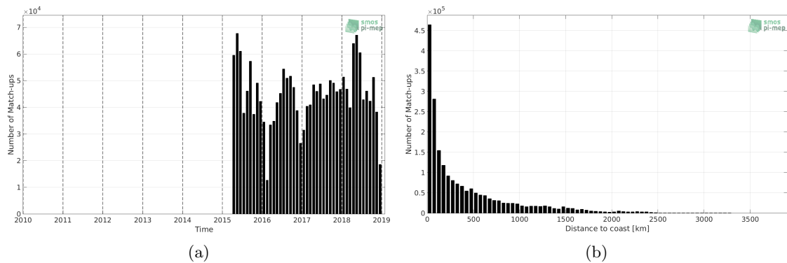
Figure 1: Number of match-ups between TSG-LEGOS-DM and SMAP-L3-JPL-V4.3-MONTHLY-60KM SSS as a function of time (a) and as function of the distance to coast (b) over the Global Ocean Pi-MEP region and for the full satellite product period.
