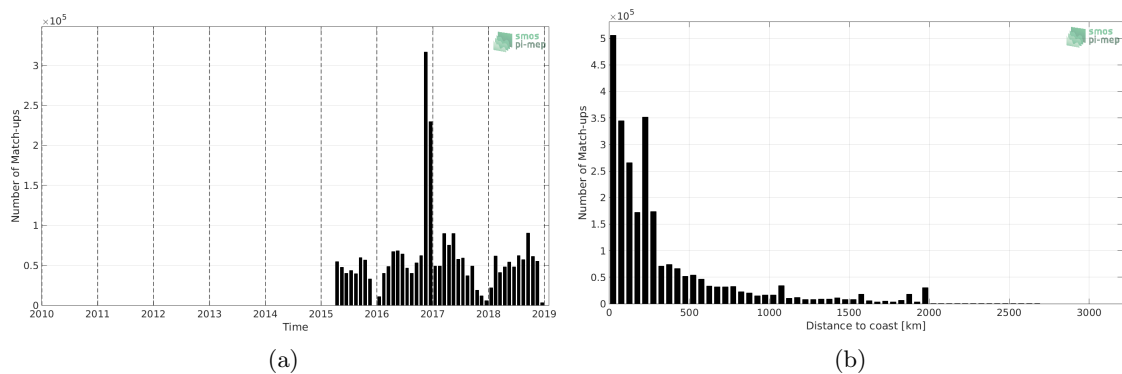
Figure 1: Number of match-ups between TSG-GOSUD-Research-vessel and SMAP-L3-JPL-V4.3-MONTHLY-60KM SSS as a function of time (a) and as function of the distance to coast (b) over the Global Ocean Pi-MEP region and for the full satellite product period.
