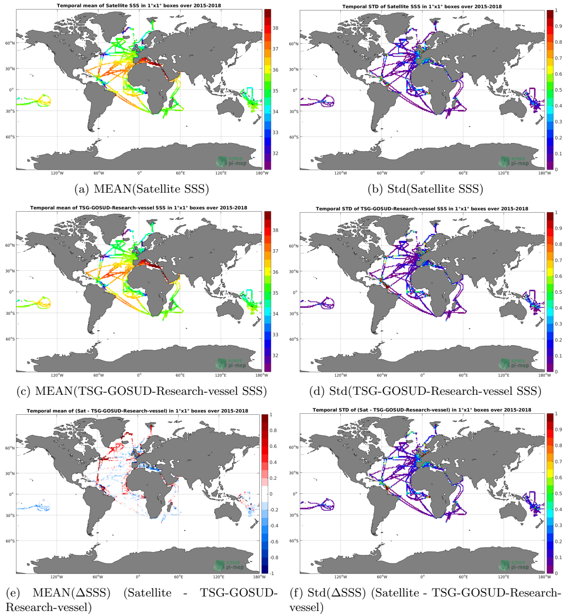
Figure 6: Temporal mean (left) and Std (right) of SSS from SMAP-L3-JPL-V4.3-MONTHLY-60KM (top), TSG-GOSUD-Research-vessel (middle), and of \Delta SSS (Satellite - TSG-GOSUD-Research-vessel). Only match-up pairs are used to generate these maps.
