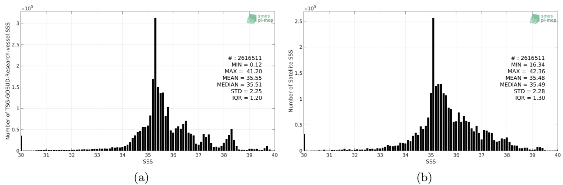
Figure 2: Histograms of SSS from TSG-GOSUD-Research-vessel (a) and SMAP-L3-JPL-V4.3-MONTHLY-60KM (b) considering all match-up pairs per bins of 0.1 over the Global Ocean Pi-MEP region and for the full satellite product period.
