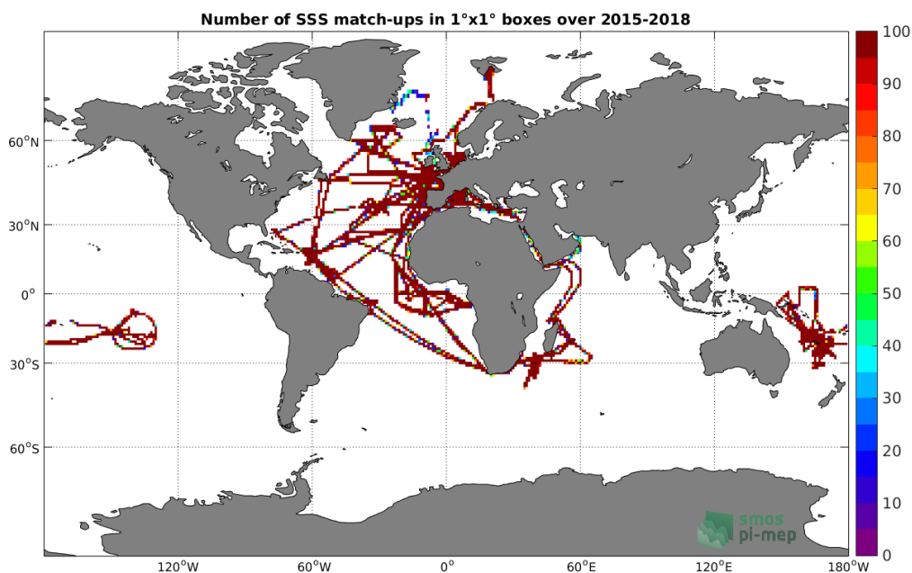
Figure 4: Number of SSS match-ups between TSG-GOSUD-Research-vessel SSS and the SMAP-L3-JPL-V4.3-MONTHLY-60KM SSS product for the Global Ocean Pi-MEP region over 1°x1° boxes and for the full satellite product period.
