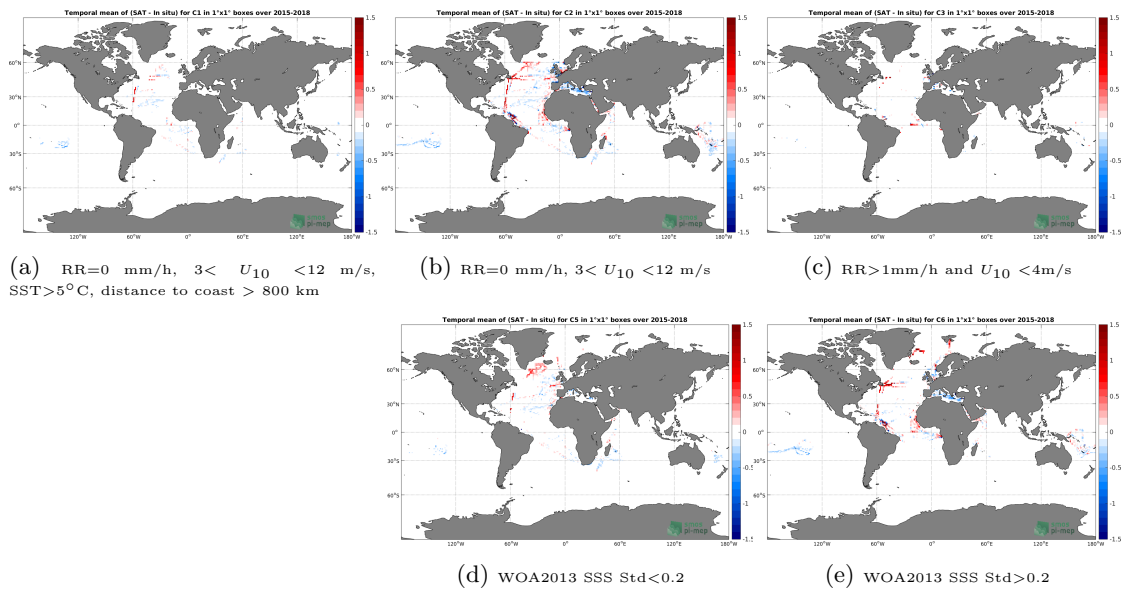
Figure 12: Temporal mean gridded over spatial boxes of size 1^\circ \times 1^\circ of \Delta SSS (SMAP-L3-JPL-V4.3-MONTHLY-60KM - TSG-GOSUD-Research-vessel) for 5 different subdatasets corresponding to: RR=0 mm/h, 3 < U_{10} < 12 m/s, SST > 5°C, distance to coast > 800 km (a), RR=0 mm/h, 3 < U_{10} < 12 m/s (b), RR > 1mm/h and U_{10} < 4 m/s (c), WOA2013 SSS Std < 0.2 (d), WOA2013 SSS Std > 0.2 (e).
