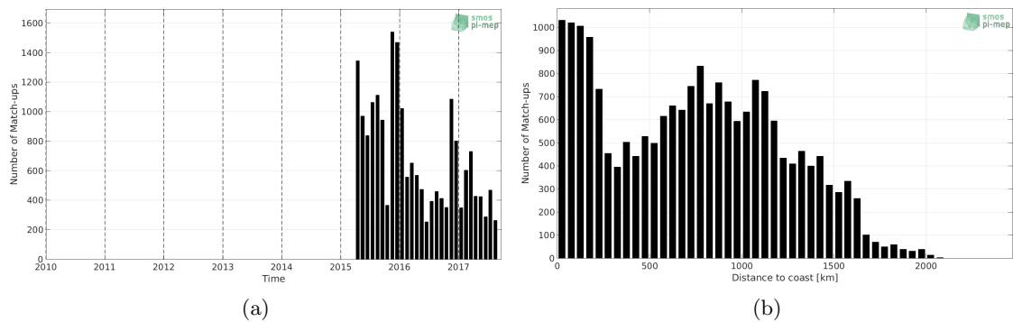
Figure 1: Number of match-ups between Sea mammals and SMAP-L3-JPL-V4.3-MONTHLY-60KM SSS as a function of time (a) and as function of the distance to coast (b) over the Global Ocean Pi-MEP region and for the full satellite product period.
