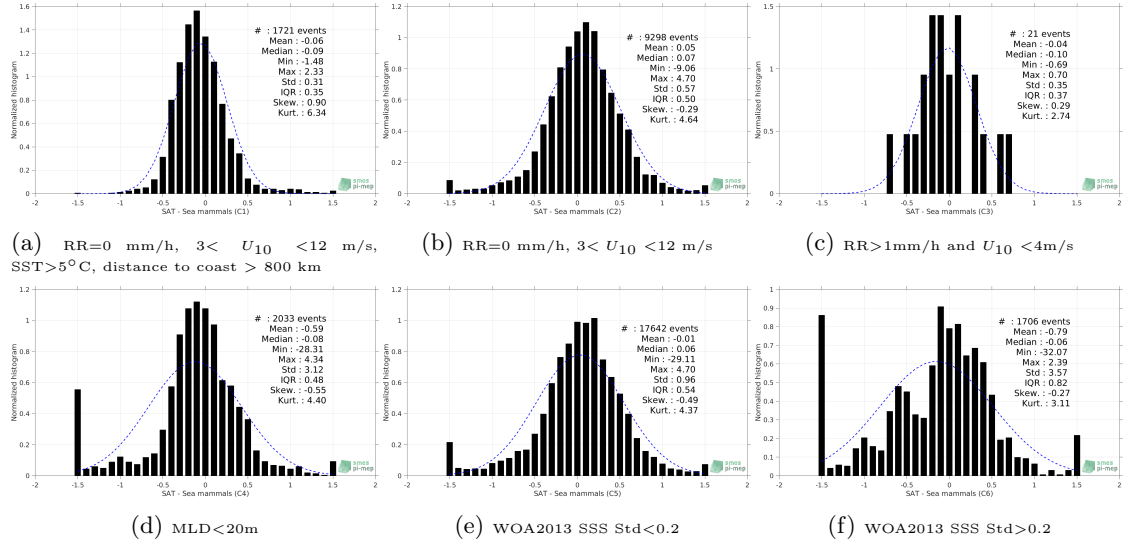
Figure 13: Normalized histogram of \Delta SSS (SMAP-L3-JPL-V4.3-MONTHLY-60KM - Sea mammals) for 6 different subdatasets corresponding to: RR=0 mm/h, 3 < U_{10} < 12 m/s, SST>5°C, distance to coast > 800 km (a), RR=0 mm/h, 3 < U_{10} < 12 m/s (b), RR>1mm/h and U_{10} < 4 m/s (c), MLD<20m (d), WOA2013 SSS Std<0.2 (e), WOA2013 SSS Std>0.2 (f).
