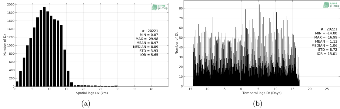
Figure 5: Histograms of the spatial (a) and temporal (b) lags between the time of the Sea mammals measurements and the date of the corresponding SMAP-L3-JPL-V4.3-MONTHLY-60KM SSS product.
