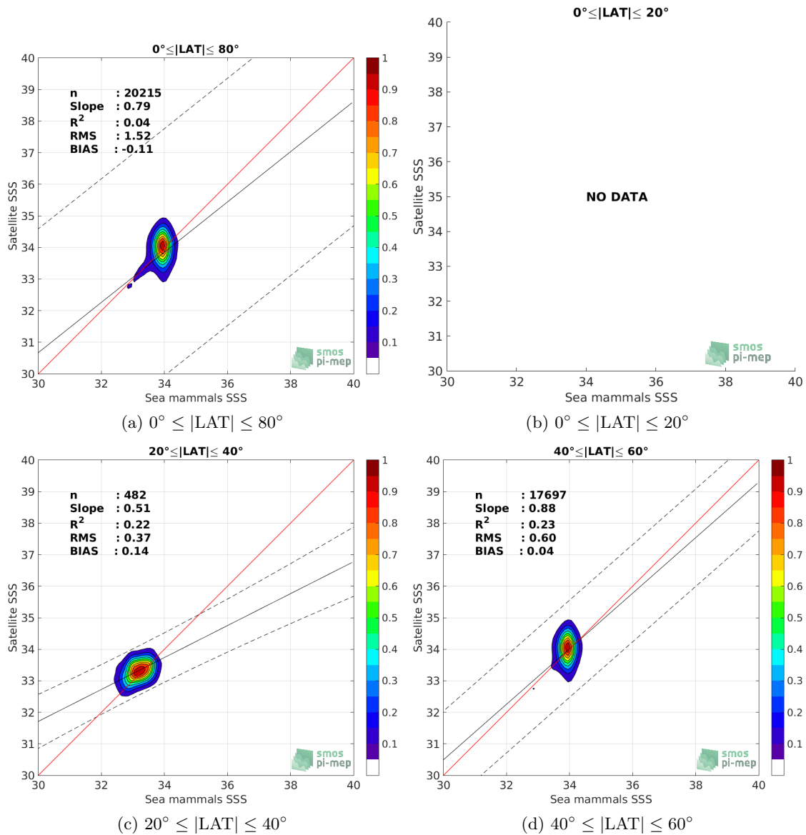
Figure 9: Contour maps of the concentration of SMAP-L3-JPL-V4.3-MONTHLY-60KM SSS (y-axis) versus Sea mammals SSS (x-axis) at match-up pairs for different latitude bands. For each plot, the red line shows x=y . The black thin and dashed lines indicate a linear fit through the data cloud and the \pm 95\% confidence levels, respectively. The number match-up pairs n , the slope and R^2 coefficient of the linear fit, the root mean square (RMS) and the mean bias between satellite and in situ data are indicated for each latitude band in each plots.
