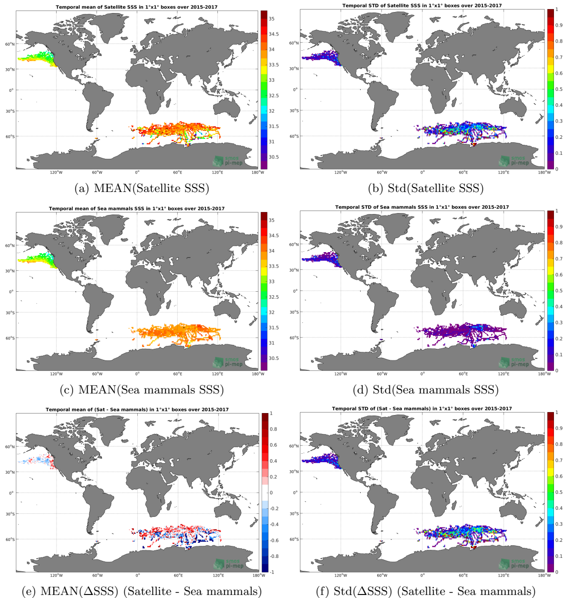
Figure 6: Temporal mean (left) and Std (right) of SSS from SMAP-L3-JPL-V4.3-MONTHLY-60KM (top), Sea mammals (middle), and of \Delta SSS (Satellite - Sea mammals). Only match-up pairs are used to generate these maps.
