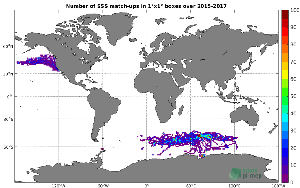
Figure 4: Number of SSS match-ups between Sea mammals SSS and the SMAP-L3-JPL-V4.3-MONTHLY-60KM SSS product for the Global Ocean Pi-MEP region over 1°x1° boxes and for the full satellite product period.
