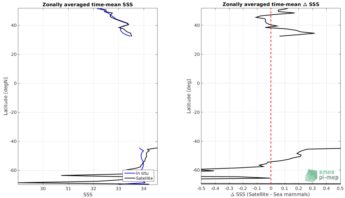
Figure 8: Left panel: Zonal mean SSS from SMAP-L3-JPL-V4.3-MONTHLY-60KM satellite product (black) and from Sea mammals (blue). Right panel: Zonal mean of \Delta SSS (Satellite - Sea mammals) for all the collected Pi-MEP match-up pairs estimated over the full satellite product period.
