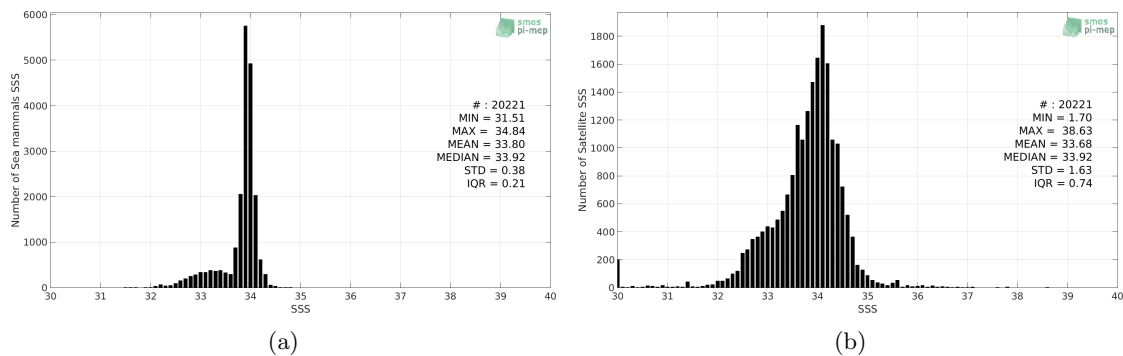
Figure 2: Histograms of SSS from Sea mammals (a) and SMAP-L3-JPL-V4.3-MONTHLY-60KM (b) considering all match-up pairs per bins of 0.1 over the Global Ocean Pi-MEP region and for the full satellite product period.
