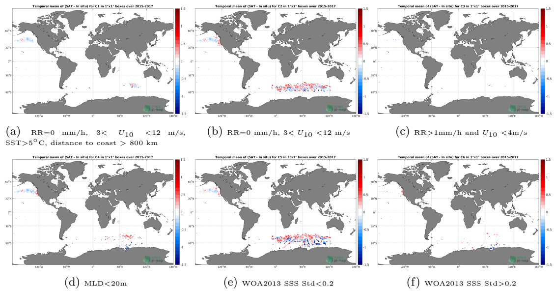
Figure 12: Temporal mean gridded over spatial boxes of size 1^\circ \times 1^\circ of \Delta SSS (SMAP-L3-JPL-V4.3-MONTHLY-60KM - Sea mammals) for 6 different subdatasets corresponding to:RR=0 mm/h, 3 < U_{10} < 12 m/s, SST >5^\circ C, distance to coast > 800 km (a), RR=0 mm/h, 3 < U_{10} < 12 m/s (b), RR >1 mm/h and U_{10} < 4 m/s (c),MLD <20 m (d),WOA2013 SSS Std <0.2 (e),WOA2013 SSS Std >0.2 (f).
