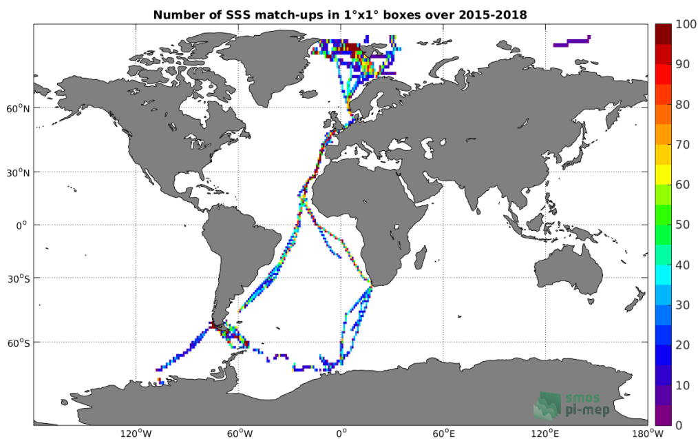
Figure 4: Number of SSS match-ups between TSG-POLARSTERN SSS and the SMAP-L3-JPL-V4.2-8DAY-RUNNING-60KM SSS product for the Global Ocean Pi-MEP region over 1°x1° boxes and for the full satellite product period.
