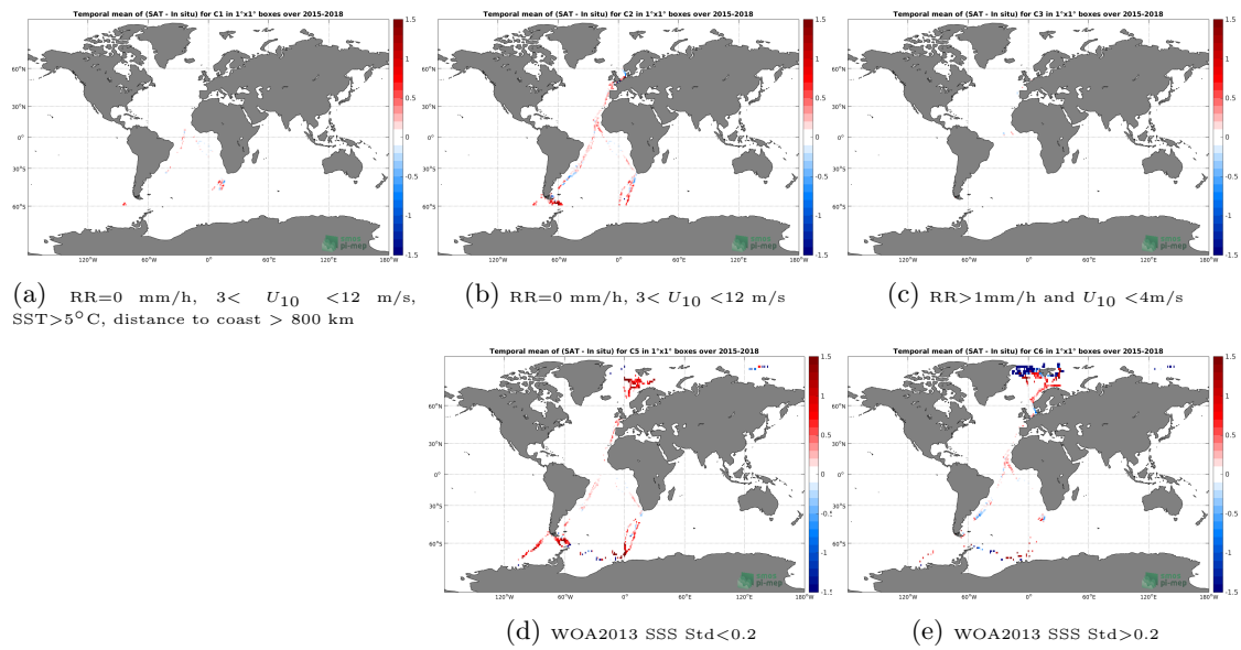
Figure 12: Temporal mean gridded over spatial boxes of size 1^\circ \times 1^\circ of \Delta SSS (SMAP-L3-JPL-V4.2-8DAY-RUNNING-60KM - TSG-POLARSTERN) for 5 different subdatasets corresponding to:RR=0 mm/h, 3 < U_{10} < 12 m/s, SST >5^\circ C, distance to coast > 800 km (a), RR=0 mm/h, 3 < U_{10} < 12 m/s (b), RR >1 mm/h and U_{10} < 4 m/s (c), WOA2013 SSS Std <0.2 (d), WOA2013 SSS Std >0.2 (e).
