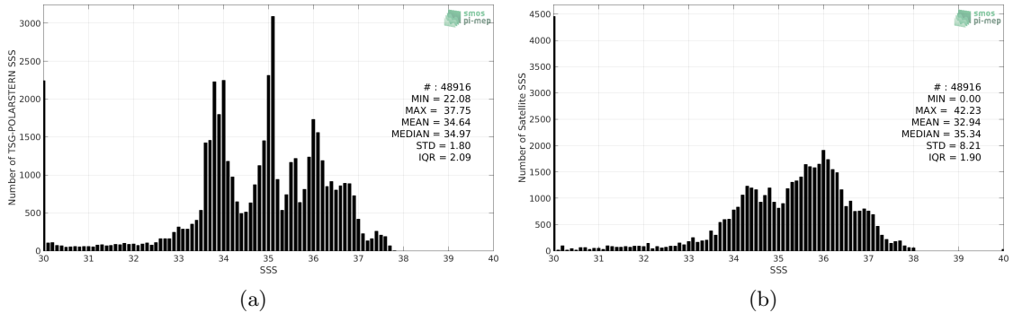
Figure 2: Histograms of SSS from TSG-POLARSTERN (a) and SMAP-L3-JPL-V4.2-8DAY-RUNNING-60KM (b) considering all match-up pairs per bins of 0.1 over the Global Ocean Pi-MEP region and for the full satellite product period.
