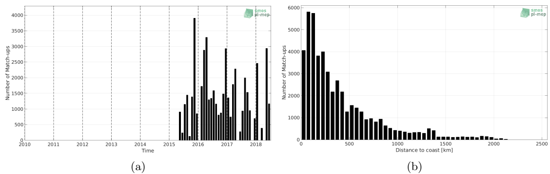
Figure 1: Number of match-ups between TSG-POLARSTERN and SMAP-L3-JPL-V4.2-8DAY-RUNNING-60KM SSS as a function of time (a) and as function of the distance to coast (b) over the Global Ocean Pi-MEP region and for the full satellite product period.
