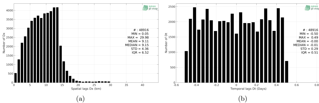
Figure 5: Histograms of the spatial (a) and temporal (b) lags between the time of the TSG-POLARSTERN measurements and the date of the corresponding SMAP-L3-JPL-V4.2-8DAY-RUNNING-60KM SSS product.
