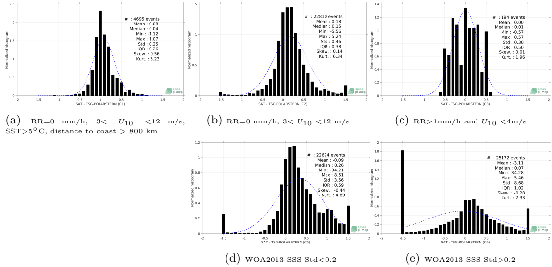
Figure 13: Normalized histogram of \Delta SSS (SMAP-L3-JPL-V4.2-8DAY-RUNNING-60KM - TSG-POLARSTERN) for 5 different subdatasets corresponding to: RR=0 mm/h, 3 < U_{10} < 12 m/s, SST>5°C, distance to coast > 800 km (a), RR=0 mm/h, 3 < U_{10} < 12 m/s (b), RR>1mm/h and U_{10} < 4 m/s (c), WOA2013 SSS Std<0.2 (d), WOA2013 SSS Std>0.2 (e).
