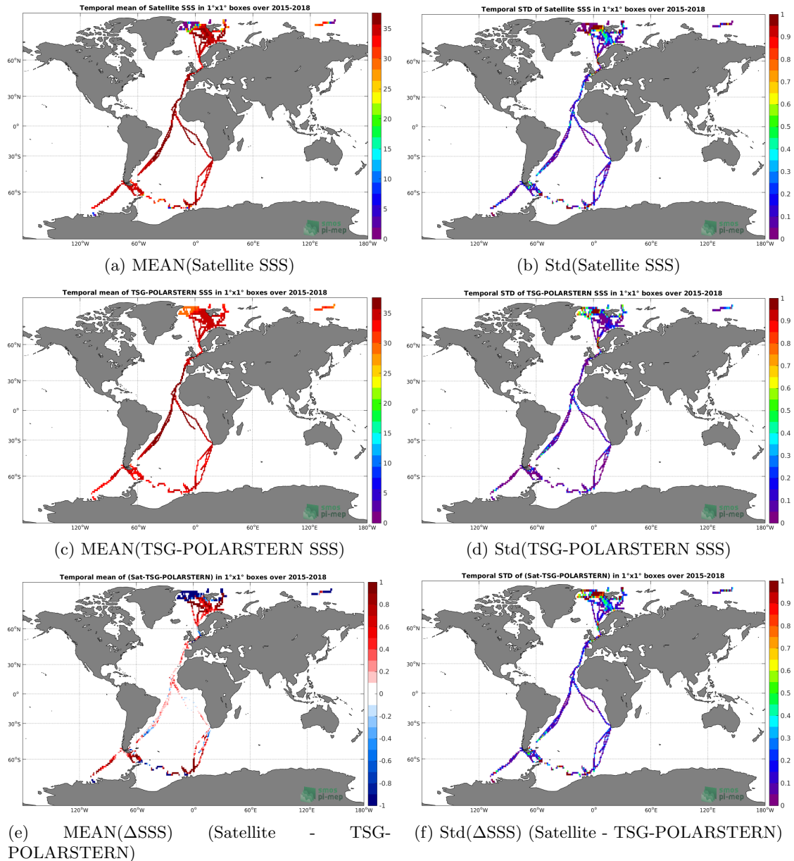
Figure 6: Temporal mean (left) and Std (right) of SSS from SMAP-L3-JPL-V4.2-8DAY-RUNNING-60KM (top), TSG-POLARSTERN (middle), and of \Delta SSS (Satellite - TSG-POLARSTERN). Only match-up pairs are used to generate these maps.
