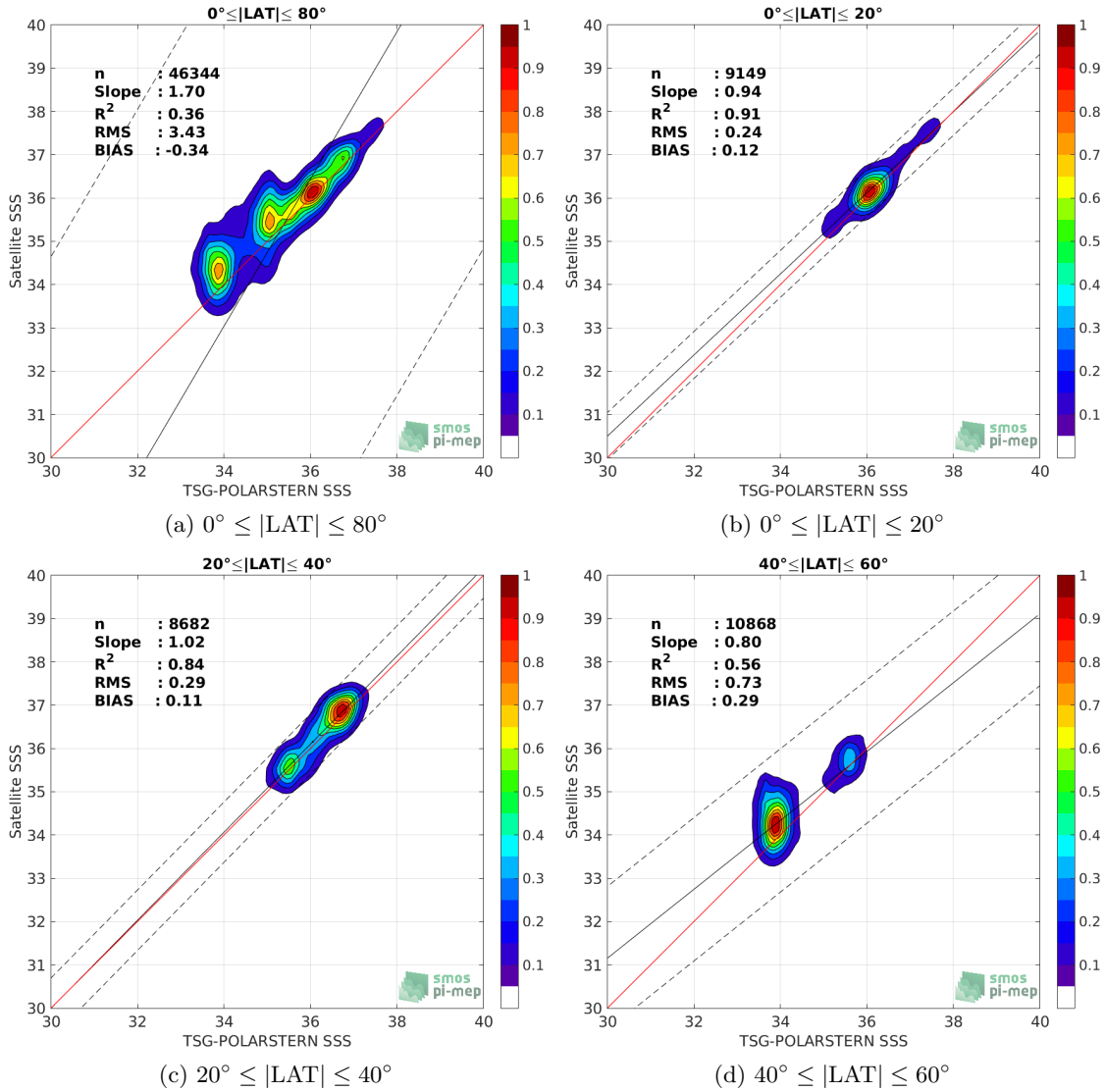
Figure 9: Contour maps of the concentration of SMAP-L3-JPL-V4.2-8DAY-RUNNING-60KM SSS (y-axis) versus TSG-POLARSTERN SSS (x-axis) at match-up pairs for different latitude bands. For each plot, the red line shows x=y . The black thin and dashed lines indicate a linear fit through the data cloud and the \pm 95\% confidence levels, respectively. The number match-up pairs n , the slope and R^2 coefficient of the linear fit, the root mean square (RMS) and the mean bias between satellite and in situ data are indicated for each latitude band in each plots.
