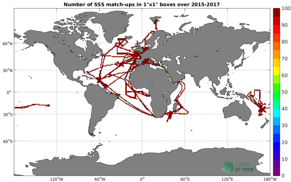
Figure 4: Number of SSS match-ups between TSG-GOSUD-Research-vessel SSS and the SMAP-L3-JPL-V4.2-8DAY-RUNNING-60KM SSS product for the Global Ocean Pi-MEP region over 1°x1° boxes and for the full satellite product period.
