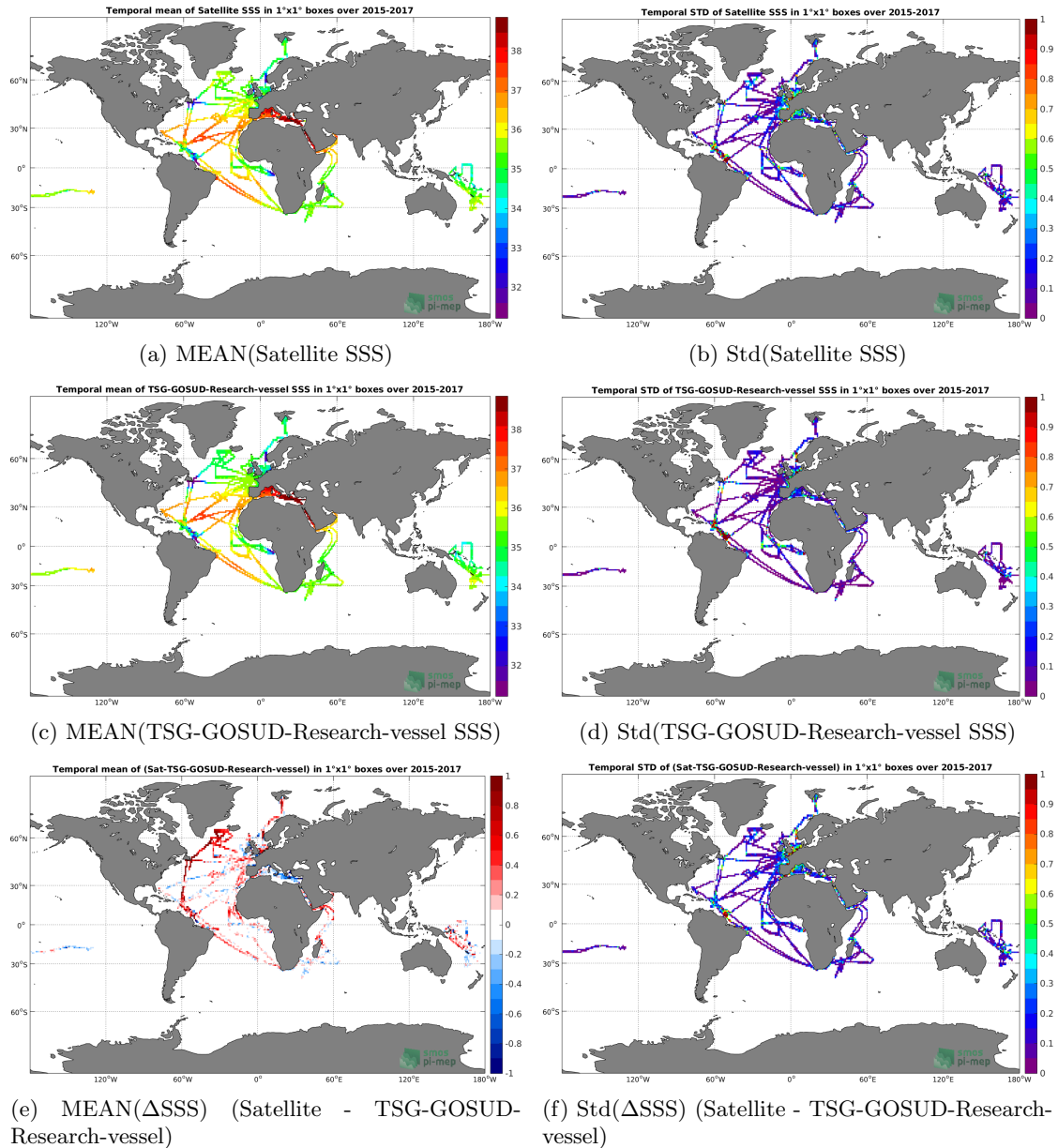
Figure 6: Temporal mean (left) and Std (right) of SSS from SMAP-L3-JPL-V4.2-8DAY-RUNNING-60KM (top), TSG-GOSUD-Research-vessel (middle), and of \Delta SSS (Satellite - TSG-GOSUD-Research-vessel). Only match-up pairs are used to generate these maps.
