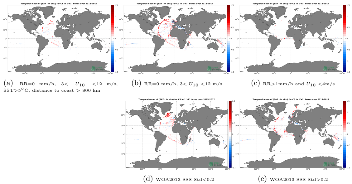
Figure 12: Temporal mean gridded over spatial boxes of size 1^\circ \times 1^\circ of \Delta SSS (SMAP-L3-JPL-V4.2-8DAY-RUNNING-60KM - TSG-GOSUD-Research-vessel) for 5 different subdatasets corresponding to: RR=0 mm/h, 3 < U_{10} < 12 m/s, SST > 5^\circ\text{C} , distance to coast > 800 km (a), RR=0 mm/h, 3 < U_{10} < 12 m/s (b), RR > 1 mm/h and U_{10} < 4 m/s (c), WOA2013 SSS Std < 0.2 (d), WOA2013 SSS Std > 0.2 (e).
