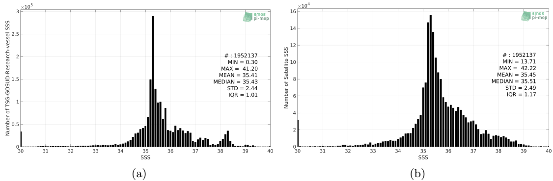
Figure 2: Histograms of SSS from TSG-GOSUD-Research-vessel (a) and SMAP-L3-JPL-V4.2-8DAY-RUNNING-60KM (b) considering all match-up pairs per bins of 0.1 over the Global Ocean Pi-MEP region and for the full satellite product period.
