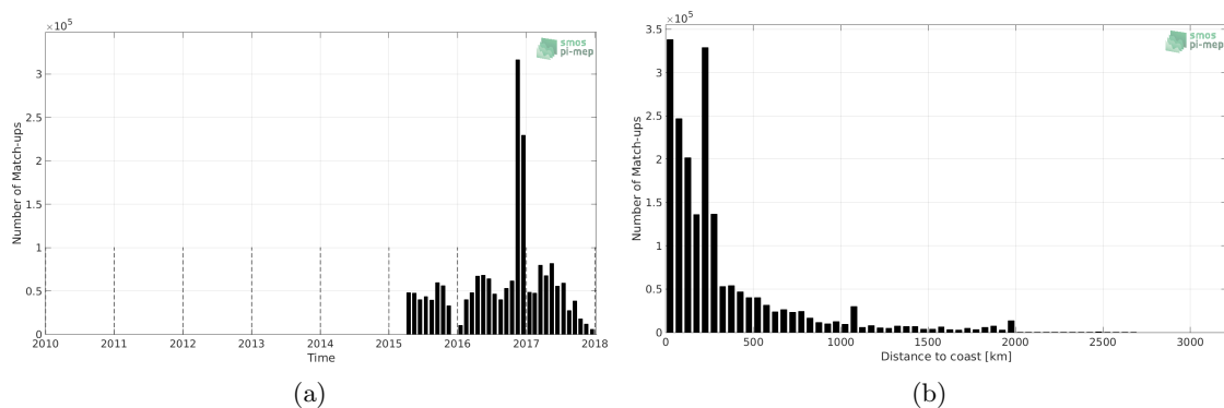
Figure 1: Number of match-ups between TSG-GOSUD-Research-vessel and SMAP-L3-JPL-V4.2-8DAY-RUNNING-60KM SSS as a function of time (a) and as function of the distance to coast (b) over the Global Ocean Pi-MEP region and for the full satellite product period.
