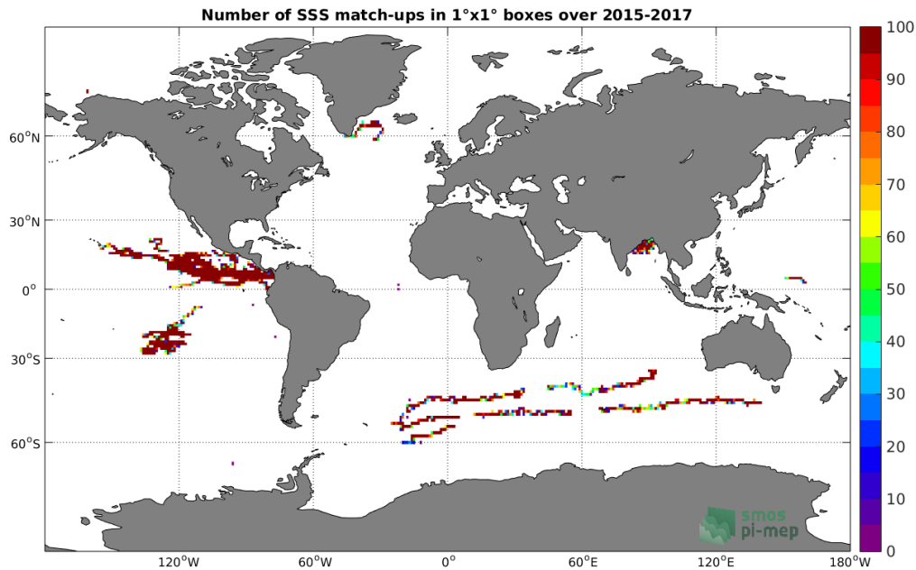
Figure 3: Number of SSS match-ups between Surface drifters SSS and the SMAP-L3-JPL-V4.2-8DAY-RUNNING-60KM SSS product for the Global Ocean Pi-MEP region over 1^{\circ} \times 1^{\circ} boxes and for the full satellite product period.
