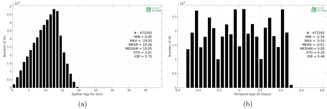
Figure 4: Histograms of the spatial (a) and temporal (b) lags between the time of the Surface drifters measurements and the date of the corresponding SMAP-L3-JPL-V4.2-8DAY-RUNNING-60KM SSS product.
