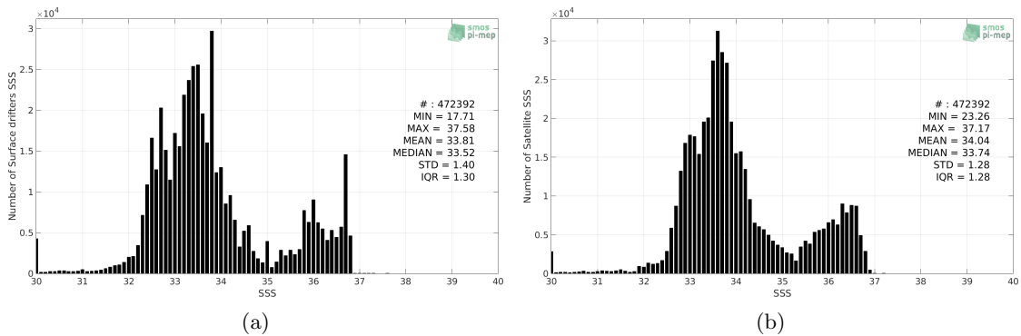
Figure 2: Histograms of SSS from Surface drifters (a) and SMAP-L3-JPL-V4.2-8DAY-RUNNING-60KM (b) considering all match-up pairs per bins of 0.1 over the Global Ocean Pi-MEP region and for the full satellite product period.
