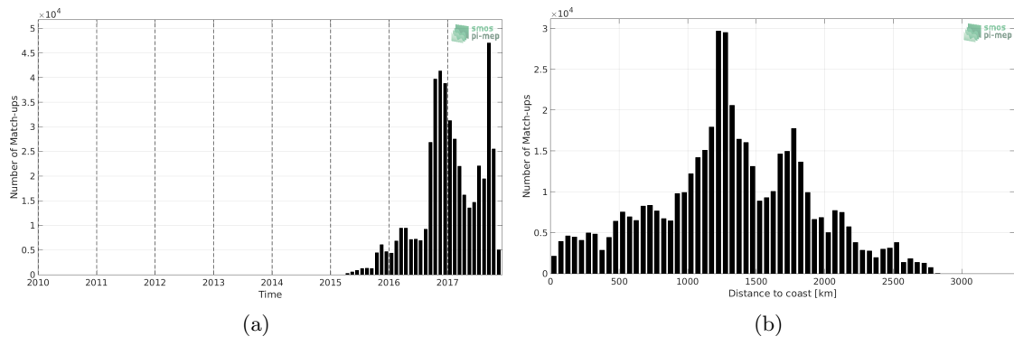
Figure 1: Number of match-ups between Surface drifters and SMAP-L3-JPL-V4.2-8DAY-RUNNING-60KM SSS as a function of time (a) and as function of the distance to coast (b) over the Global Ocean Pi-MEP region and for the full satellite product period.
