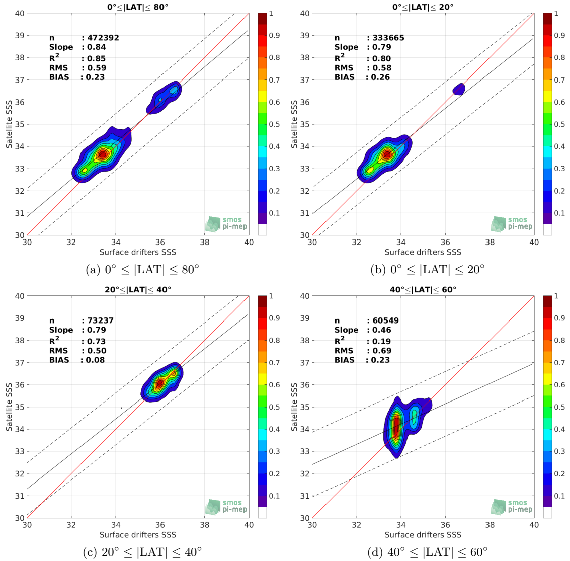
Figure 8: Contour maps of the concentration of SMAP-L3-JPL-V4.2-8DAY-RUNNING-60KM SSS (y-axis) versus Surface drifters SSS (x-axis) at match-up pairs for different latitude bands. For each plot, the red line shows x=y . The black thin and dashed lines indicate a linear fit through the data cloud and the \pm 95\% confidence levels, respectively. The number match-up pairs n , the slope and R^2 coefficient of the linear fit, the root mean square (RMS) and the mean bias between satellite and in situ data are indicated for each latitude band in each plots.
