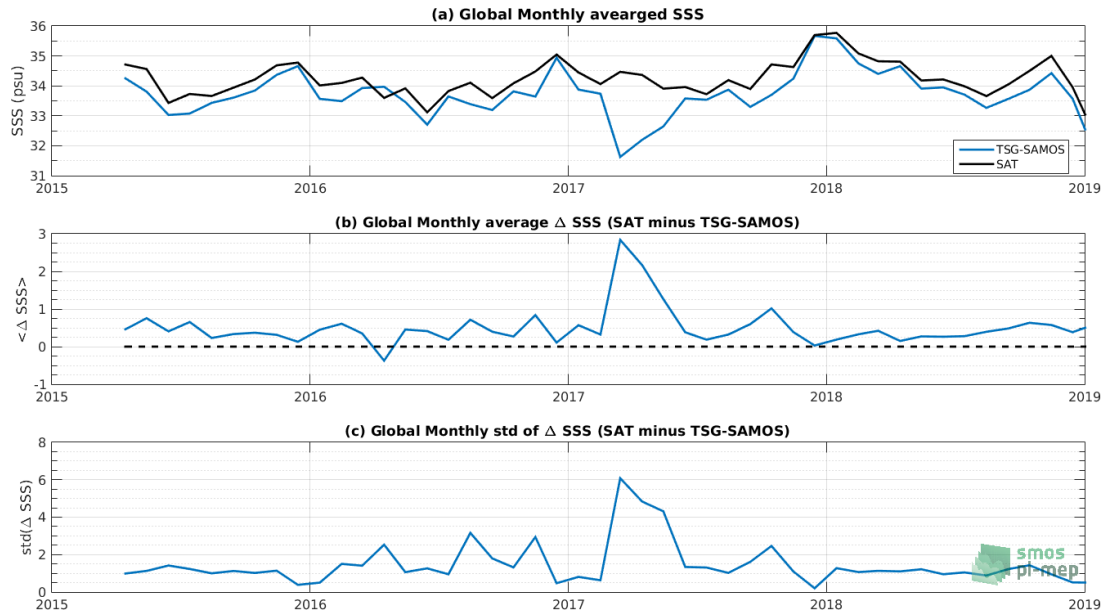
Figure 7: Time series of the monthly averaged mean SSS (top), mean \Delta SSS (Satellite - TSG-SAMOS) and Std of \Delta SSS (Satellite - TSG-SAMOS) over the Global Ocean Pi-MEP region considering all match-ups collected by the Pi-MEP platform.
