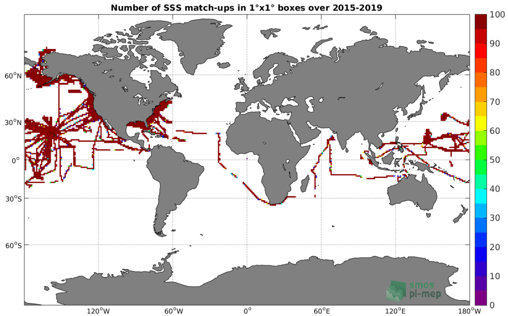
Figure 4: Number of SSS match-ups between TSG-SAMOS SSS and the SMAP-L3-JPL-V4.2-MONTHLY-60KM SSS product for the Global Ocean Pi-MEP region over 1^\circ \times 1^\circ boxes and for the full satellite product period.
