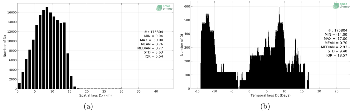
Figure 5: Histograms of the spatial (a) and temporal (b) lags between the time of the TSG-LEGOS-Survostral measurements and the date of the corresponding SMAP-L3-JPL-V4.2-MONTHLY-60KM SSS product.
