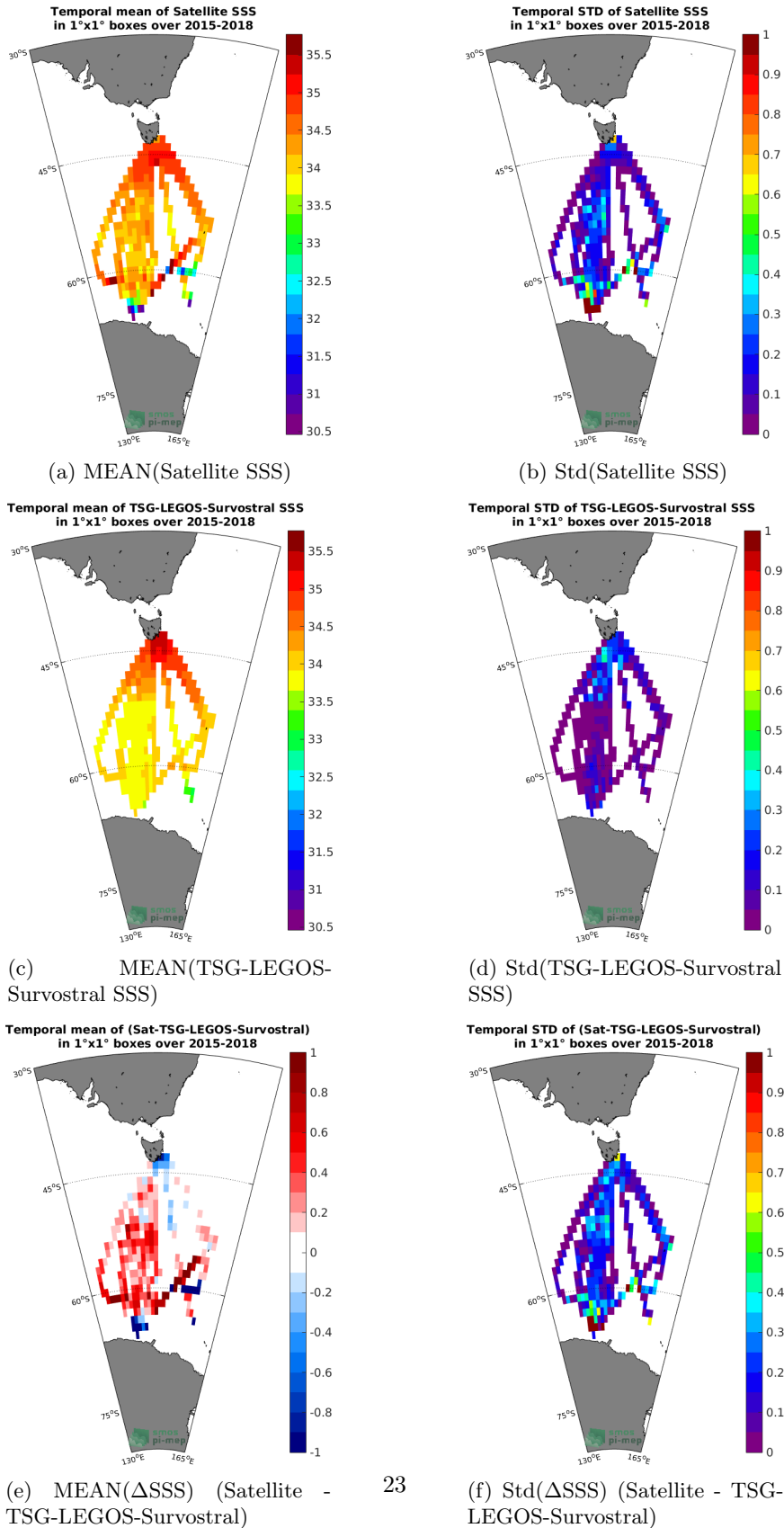
Figure 6: Temporal mean (left) and Std (right) of SSS from SMAP-L3-JPL-V4.2-MONTHLY-60KM (top), TSG-LEGOS-Survostral (middle), and of \Delta SSS (Satellite - TSG-LEGOS-Survostral). Only match-up pairs are used to generate these maps.
