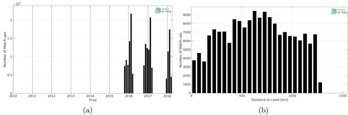
Figure 1: Number of match-ups between TSG-LEGOS-Survostral and SMAP-L3-JPL-V4.2-MONTHLY-60KM SSS as a function of time (a) and as function of the distance to coast (b) over the Global Ocean Pi-MEP region and for the full satellite product period.
