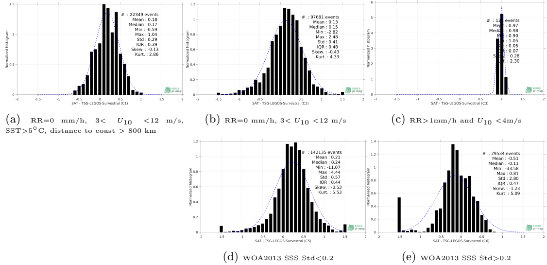
Figure 13: Normalized histogram of \Delta\text{SSS} (SMAP-L3-JPL-V4.2-MONTHLY-60KM - TSG-LEGOS-Survostral) for 5 different subdatasets corresponding to: RR=0 mm/h, 3 < U_{10} < 12 m/s, SST > 5^{\circ}\text{C} , distance to coast > 800 km (a), RR=0 mm/h, 3 < U_{10} < 12 m/s (b), RR > 1\text{mm/h} and U_{10} < 4\text{m/s} (c), WOA2013 SSS Std < 0.2 (d), WOA2013 SSS Std > 0.2 (e).
