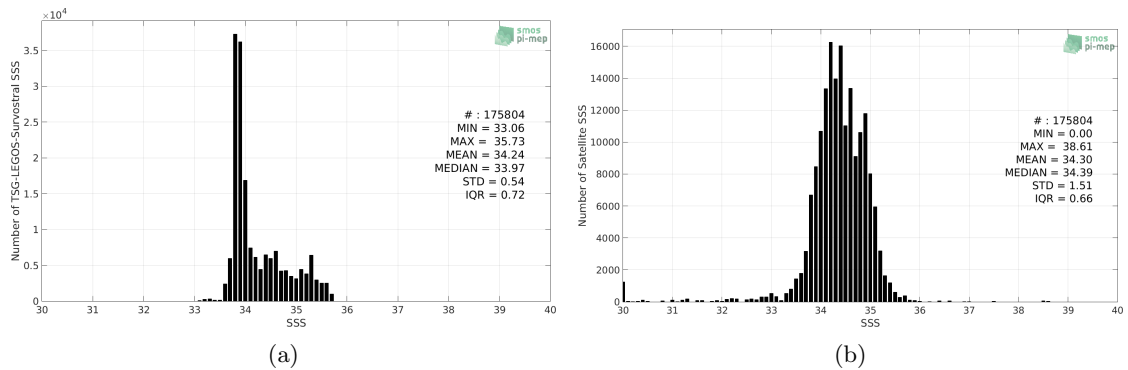
Figure 2: Histograms of SSS from TSG-LEGOS-Survostral (a) and SMAP-L3-JPL-V4.2-MONTHLY-60KM (b) considering all match-up pairs per bins of 0.1 over the Global Ocean Pi-MEP region and for the full satellite product period.
