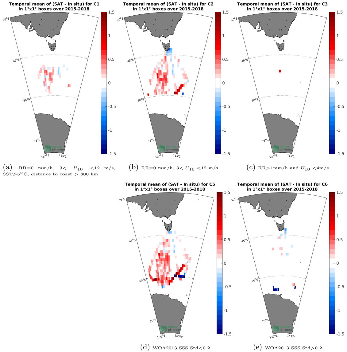
Figure 12: Temporal mean gridded over spatial boxes of size 1°x1° of \Delta SSS (SMAP-L3-JPL-V4.2-MONTHLY-60KM - TSG-LEGOS-Survostral) for 5 different subdatasets corresponding to:RR=0 mm/h, 3 < U_{10} < 12 m/s, SST>5°C, distance to coast > 800 km (a), RR=0 mm/h, 3 < U_{10} < 12 m/s (b), RR>1mm/h and U_{10} < 4 m/s (c), WOA2013 SSS Std<0.2 (d), WOA2013 SSS Std>0.2 (e).
