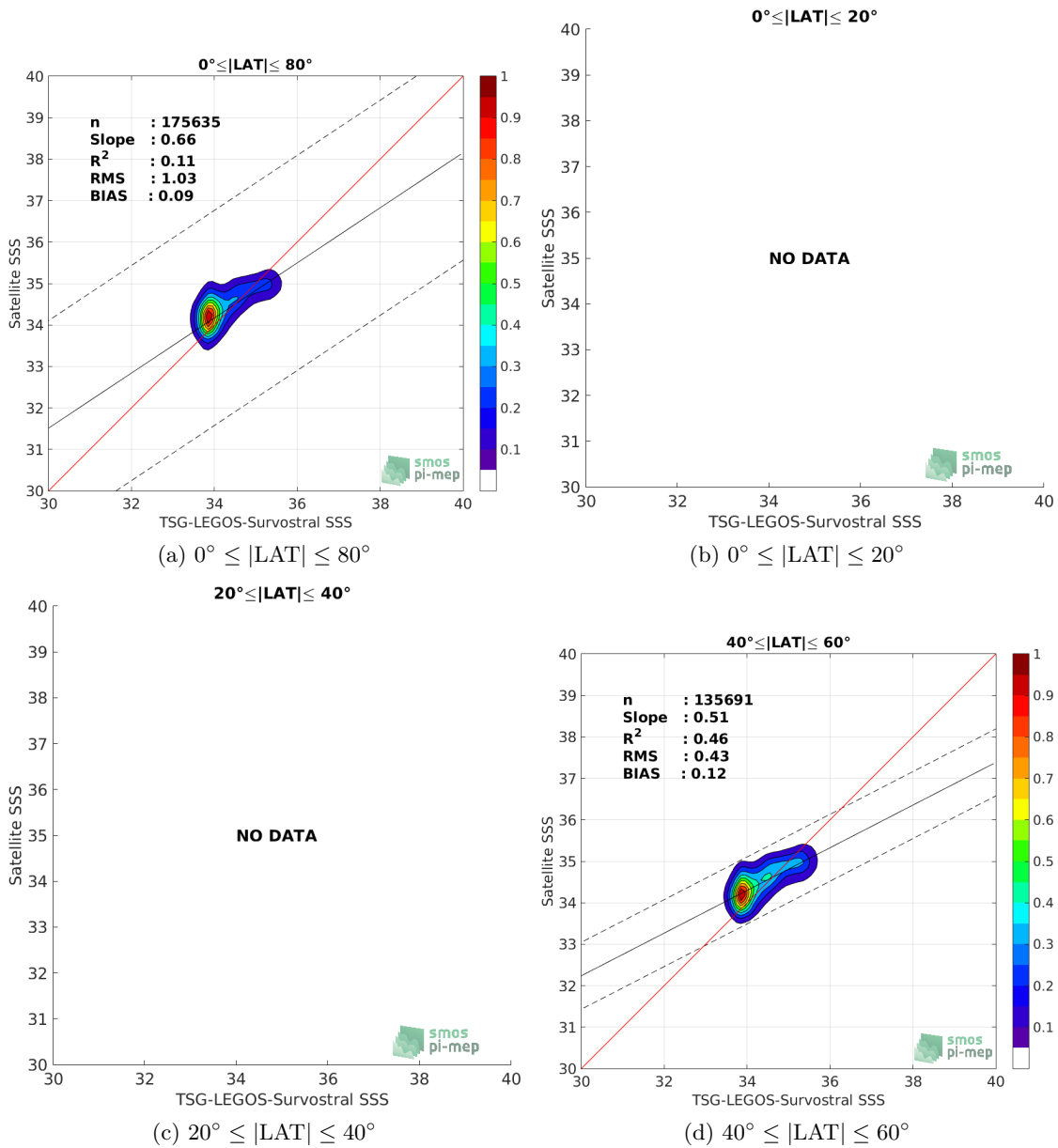
Figure 9: Contour maps of the concentration of SMAP-L3-JPL-V4.2-MONTHLY-60KM SSS (y-axis) versus TSG-LEGOS-Survostral SSS (x-axis) at match-up pairs for different latitude bands. For each plot, the red line shows x=y . The black thin and dashed lines indicate a linear fit through the data cloud and the \pm 95\% confidence levels, respectively. The number match-up pairs n , the slope and R^2 coefficient of the linear fit, the root mean square (RMS) and the mean bias between satellite and in situ data are indicated for each latitude band in each plots.
