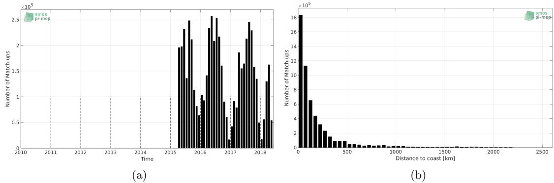
Figure 1: Number of match-ups between TSG-SAMOS and SMAP-L3-JPL-V4-8DAY-RUNNING-60KM SSS as a function of time (a) and as function of the distance to coast (b) over the Global Ocean Pi-MEP region and for the full satellite product period.
