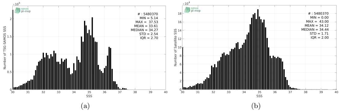
Figure 2: Histograms of SSS from TSG-SAMOS (a) and SMAP-L3-JPL-V4-8DAY-RUNNING-60KM (b) considering all match-up pairs per bins of 0.1 over the Global Ocean Pi-MEP region and for the full satellite product period.
