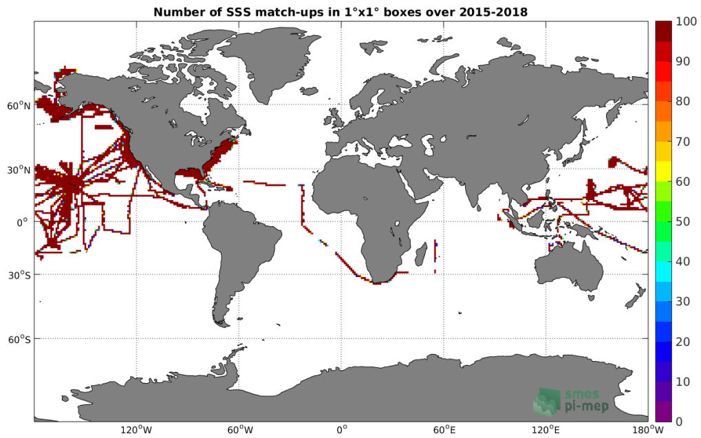
Figure 4: Number of SSS match-ups between TSG-SAMOS SSS and the SMAP-L3-JPL-V4-8DAY-RUNNING-60KM SSS product for the Global Ocean Pi-MEP region over 1°x1° boxes and for the full satellite product period.
