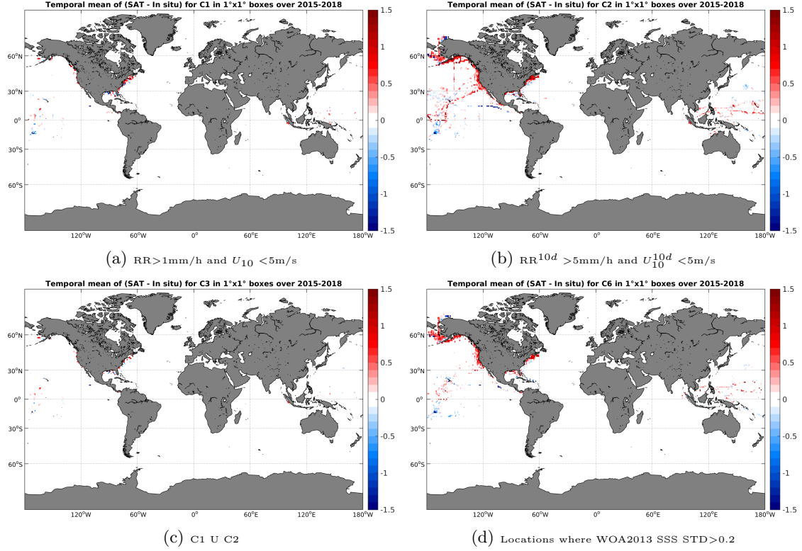
Figure 12: Temporal mean gridded over spatial boxes of size 1^\circ \times 1^\circ of \Delta SSS (SMAP-L3-JPL-V4-8DAY-RUNNING-60KM - TSG-SAMOS) for 4 different subdatasets corresponding to: RR > 1mm/h and U_{10} < 5 m/s (a), RR^{10d} > 5 mm/h and U_{10}^{10d} < 5 m/s (b), C1 U C2 (c), Locations where WOA2013 SSS STD > 0.2 (d).
