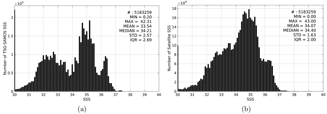
Figure 2: Histograms of SSS from TSG-SAMOS (a) and SMAP-L3-JPL-V4-8DAY-RUNNING-60KM (b) considering all match-up pairs per bins of 0.1 over the Global Ocean Pi-MEP region and for the full satellite product period.
