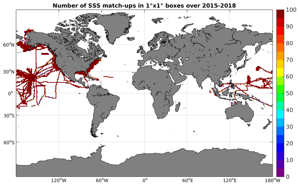
Figure 4: Number of SSS match-ups between TSG-SAMOS SSS and the SMAP-L3-JPL-V4-8DAY-RUNNING-60KM SSS product for the Global Ocean Pi-MEP region over 1^\circ \times 1^\circ boxes and for the full satellite product period.
