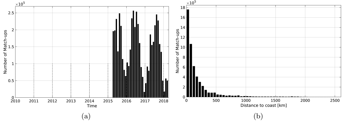
Figure 1: Number of match-ups between TSG-SAMOS and SMAP-L3-JPL-V4-8DAY-RUNNING-60KM SSS as a function of time (a) and as function of the distance to coast (b) over the Global Ocean Pi-MEP region and for the full satellite product period.
