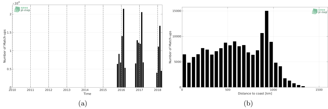
Figure 1: Number of match-ups between TSG-LEGOS-Survostral and SMAP-L3-JPL-V4-8DAY-RUNNING-60KM SSS as a function of time (a) and as function of the distance to coast (b) over the Global Ocean Pi-MEP region and for the full satellite product period.
