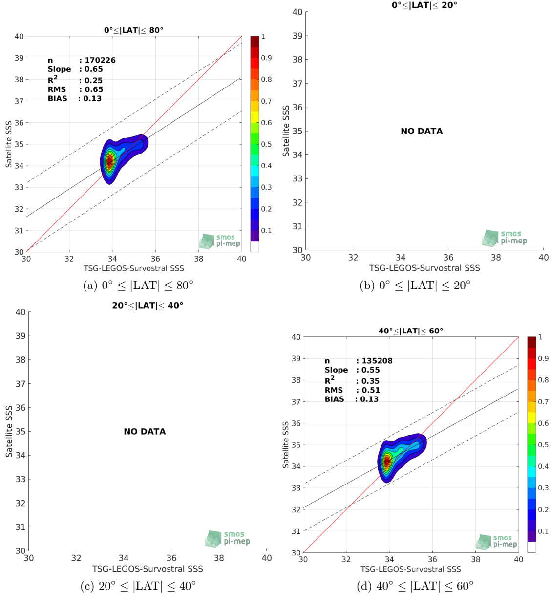
Figure 9: Contour maps of the concentration of SMAP-L3-JPL-V4-8DAY-RUNNING-60KM SSS (y-axis) versus TSG-LEGOS-Survostral SSS (x-axis) at match-up pairs for different latitude bands. For each plot, the red line shows x=y . The black thin and dashed lines indicate a linear fit through the data cloud and the \pm 95\% confidence levels, respectively. The number match-up pairs n , the slope and R^2 coefficient of the linear fit, the root mean square (RMS) and the mean bias between satellite and in situ data are indicated for each latitude band in each plots.
