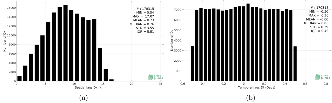
Figure 5: Histograms of the spatial (a) and temporal (b) lags between the time of the TSG-LEGOS-Survostral measurements and the date of the corresponding SMAP-L3-JPL-V4-8DAY-RUNNING-60KM SSS product.
