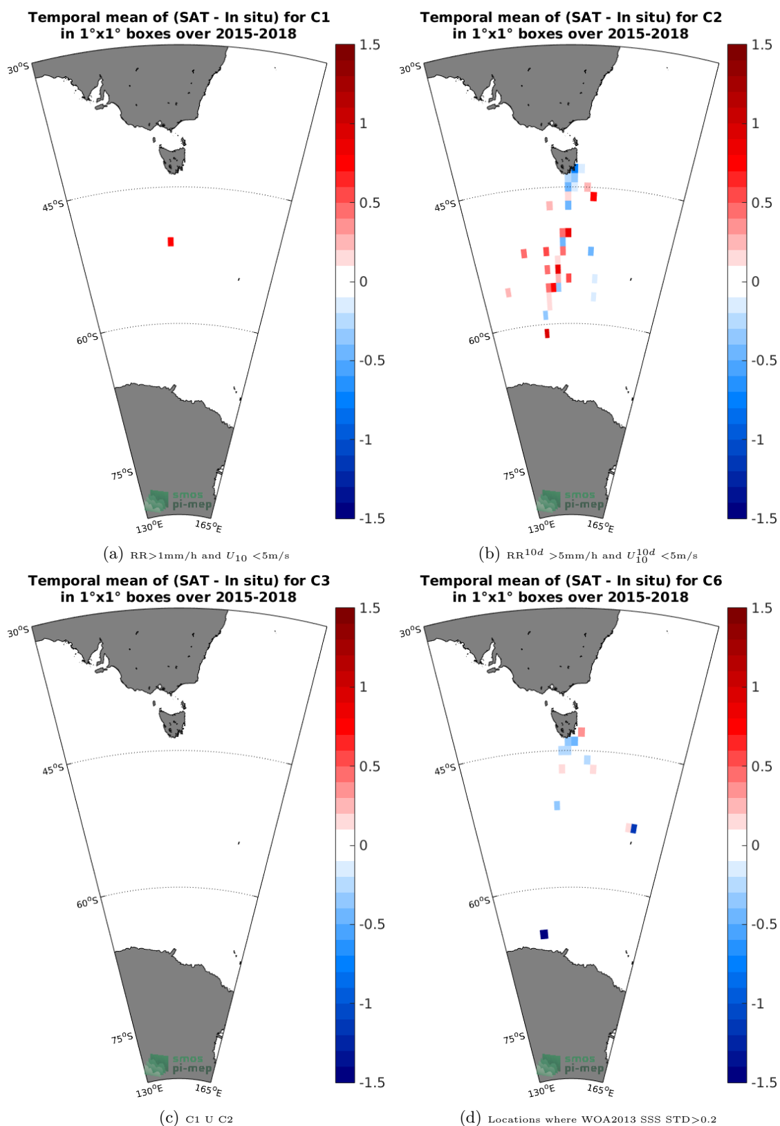
Figure 12: Temporal mean gridded over spatial boxes of size 1°x1° of \Delta\text{SSS} (SMAP-L3-JPL-V4-8DAY-RUNNING-60KM - TSG-LEGOS-Survostral) for 4 different subdatasets corresponding to: RR > 1\text{mm/h} and U_{10} < 5\text{m/s} (a), RR^{10d} > 5\text{mm/h} and U_{10}^{10d} < 5\text{m/s} (b), C1 U C2 (c), Locations where WOA2013 SSS STD > 0.2 (d).
