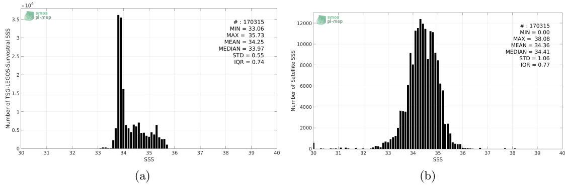
Figure 2: Histograms of SSS from TSG-LEGOS-Survostral (a) and SMAP-L3-JPL-V4-8DAY-RUNNING-60KM (b) considering all match-up pairs per bins of 0.1 over the Global Ocean Pi-MEP region and for the full satellite product period.
