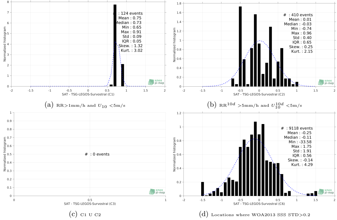
Figure 13: Normalized histogram of \Delta\text{SSS} (SMAP-L3-JPL-V4-8DAY-RUNNING-60KM - TSG-LEGOS-Survostral) for 6 different subdatasets corresponding to: RR > 1\text{mm/h} and U_{10} < 5\text{m/s} (a), RR^{10d} > 5\text{mm/h} and U_{10}^{10d} < 5\text{m/s} (b), C1 \cup C2 (c), Locations where WOA2013 SSS STD > 0.2 (d).
