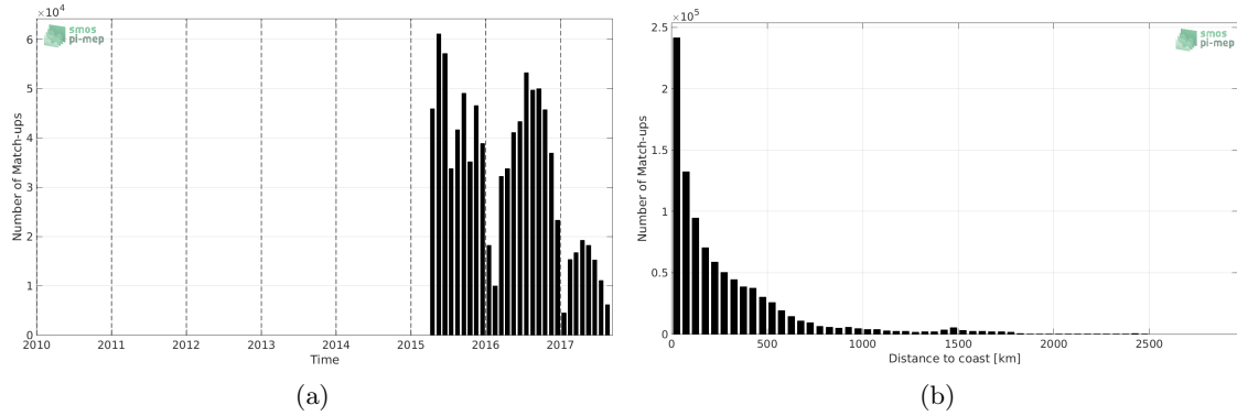
Figure 1: Number of match-ups between TSG-LEGOS-DM and SMAP-L3-JPL-V4-8DAY-RUNNING-60KM SSS as a function of time (a) and as function of the distance to coast (b) over the Global Ocean Pi-MEP region and for the full satellite product period.
