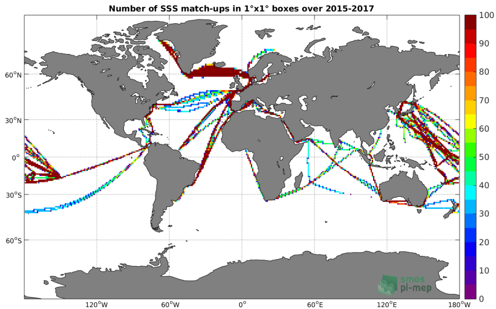
Figure 4: Number of SSS match-ups between TSG-LEGOS-DM SSS and the SMAP-L3-JPL-V4-8DAY-RUNNING-60KM SSS product for the Global Ocean Pi-MEP region over 1^\circ \times 1^\circ boxes and for the full satellite product period.
