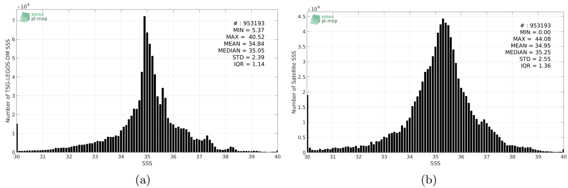
Figure 2: Histograms of SSS from TSG-LEGOS-DM (a) and SMAP-L3-JPL-V4-8DAY-RUNNING-60KM (b) considering all match-up pairs per bins of 0.1 over the Global Ocean Pi-MEP region and for the full satellite product period.
