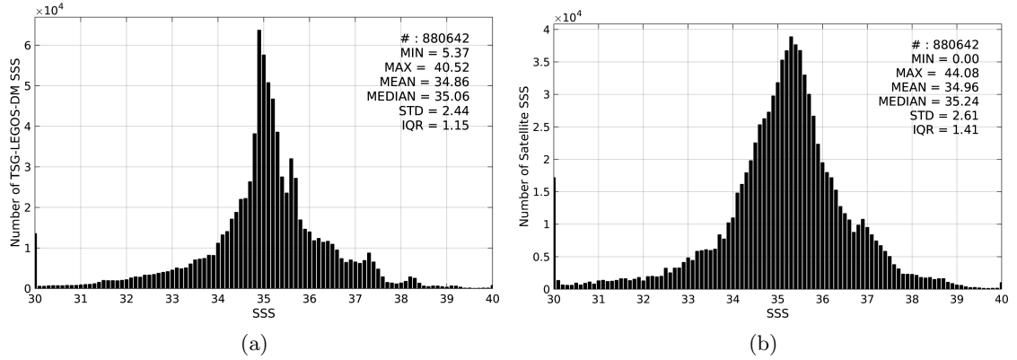
Figure 2: Histograms of SSS from TSG-LEGOS-DM (a) and SMAP-L3-JPL-V4-8DAY-RUNNING-60KM (b) considering all match-up pairs per bins of 0.1 over the Global Ocean Pi-MEP region and for the full satellite product period.
