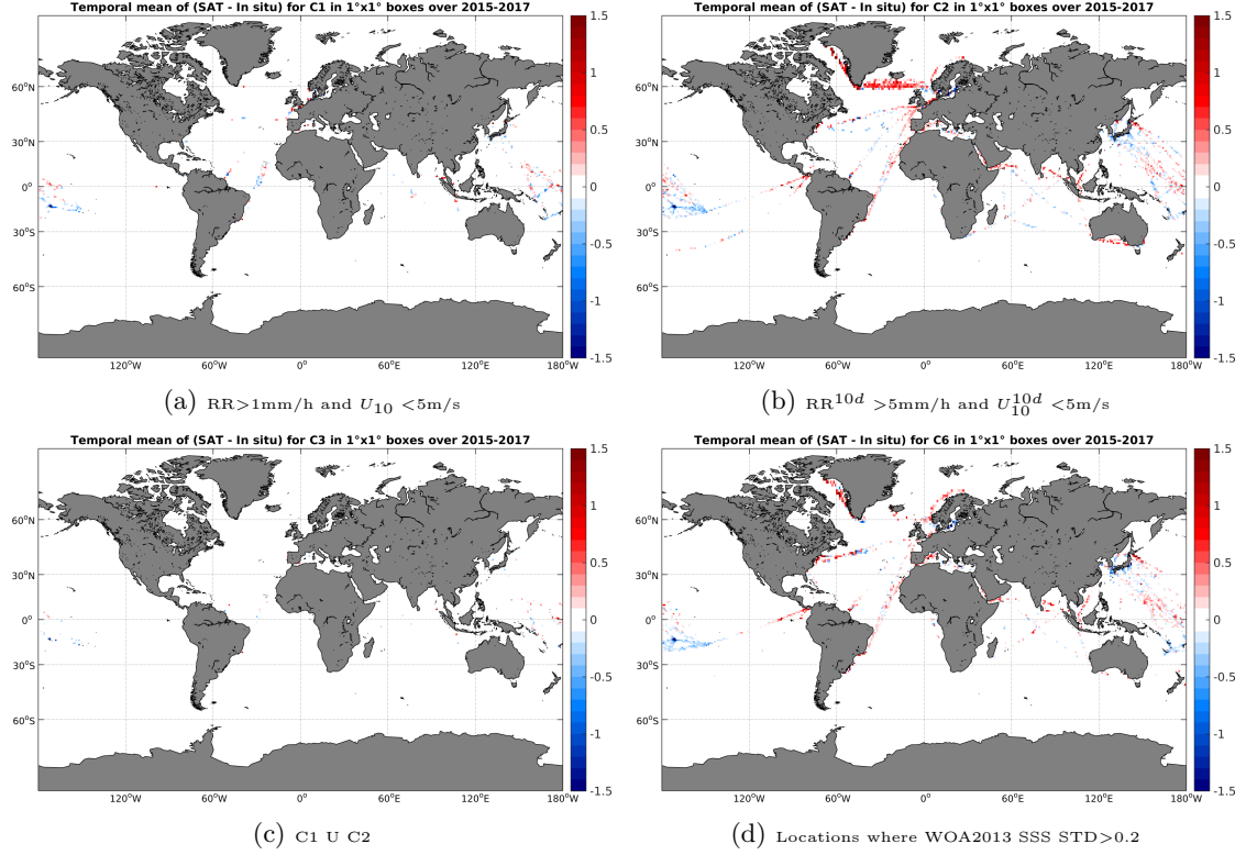
Figure 12: Temporal mean gridded over spatial boxes of size 1^\circ \times 1^\circ of \Delta SSS (SMAP-L3-JPL-V4-8DAY-RUNNING-60KM - TSG-LEGOS-DM) for 4 different subdatasets corresponding to: RR > 1\text{mm/h} and U_{10} < 5\text{m/s} (a), RR^{10d} > 5\text{mm/h} and U_{10}^{10d} < 5\text{m/s} (b), C1 U C2 (c), Locations where WOA2013 SSS STD > 0.2 (d).
