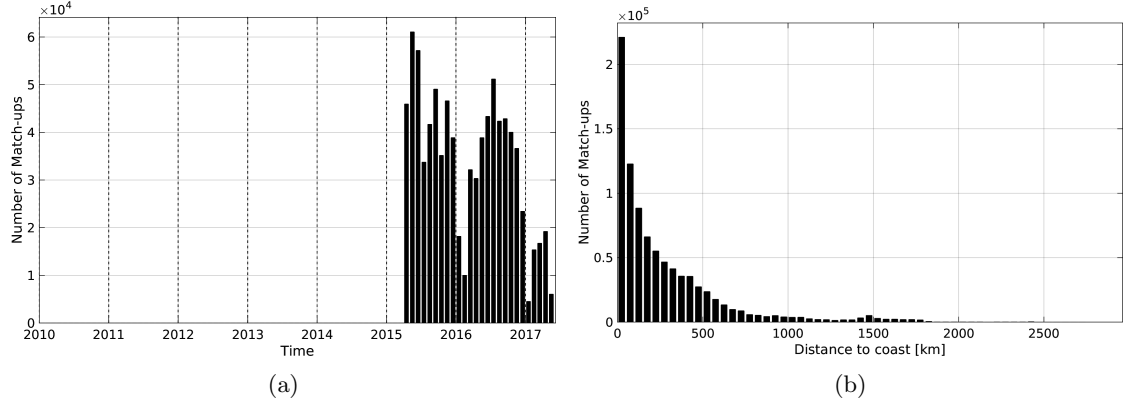
Figure 1: Number of match-ups between TSG-LEGOS-DM and SMAP-L3-JPL-V4-8DAY-RUNNING-60KM SSS as a function of time (a) and as function of the distance to coast (b) over the Global Ocean Pi-MEP region and for the full satellite product period.
