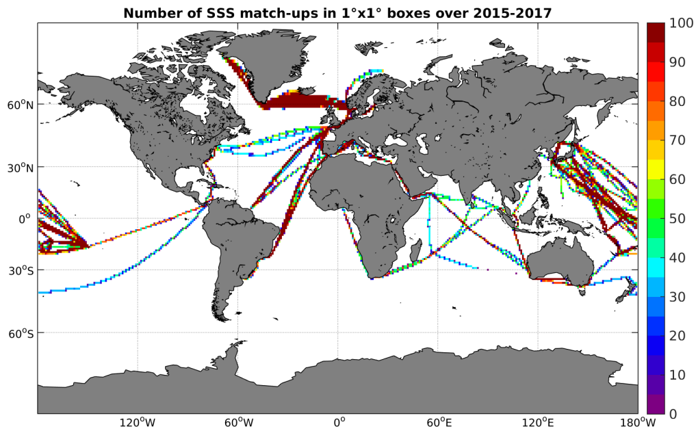
Figure 4: Number of SSS match-ups between TSG-LEGOS-DM SSS and the SMAP-L3-JPL-V4-8DAY-RUNNING-60KM SSS product for the Global Ocean Pi-MEP region over 1^\circ \times 1^\circ boxes and for the full satellite product period.
