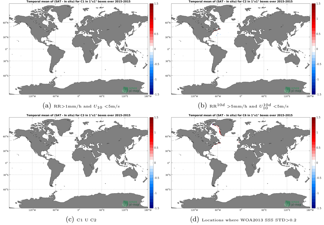
Figure 12: Temporal mean gridded over spatial boxes of size 1^\circ \times 1^\circ of \Delta SSS (SMAP-L3-JPL-V4-8DAY-RUNNING-60KM - TSG-GOSUD-Sailing-ship) for 4 different subdatasets corresponding to: RR > 1\text{mm/h} and U_{10} < 5\text{m/s} (a), RR^{10d} > 5\text{mm/h} and U_{10}^{10d} < 5\text{m/s} (b), C1 U C2 (c), Locations where WOA2013 SSS STD > 0.2 (d).
