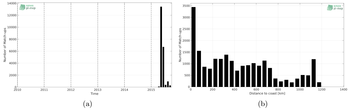
Figure 1: Number of match-ups between TSG-GOSUD-Sailing-ship and SMAP-L3-JPL-V4-8DAY-RUNNING-60KM SSS as a function of time (a) and as function of the distance to coast (b) over the Global Ocean Pi-MEP region and for the full satellite product period.
