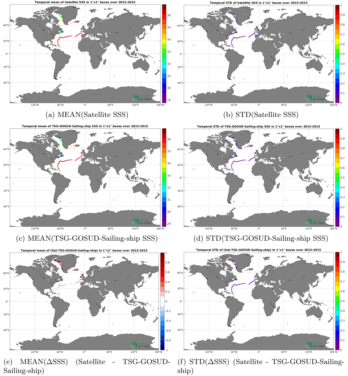
Figure 6: Temporal mean (left) and STD (right) of SSS from SMAP-L3-JPL-V4-8DAY-RUNNING-60KM (top), TSG-GOSUD-Sailing-ship (middle), and of \Delta SSS (Satellite - TSG-GOSUD-Sailing-ship). Only match-up pairs are used to generate these maps.
