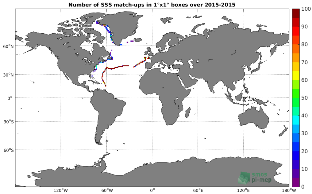
Figure 4: Number of SSS match-ups between TSG-GOSUD-Sailing-ship SSS and the SMAP-L3-JPL-V4-8DAY-RUNNING-60KM SSS product for the Global Ocean Pi-MEP region over 1^\circ \times 1^\circ boxes and for the full satellite product period.
