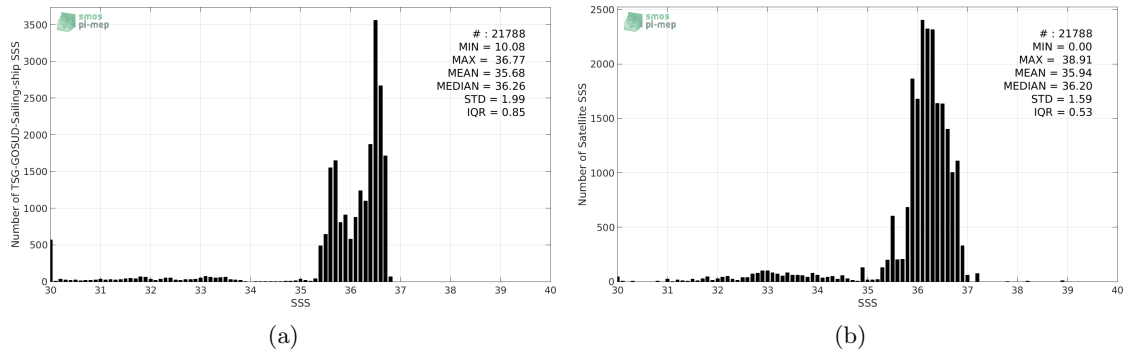
Figure 2: Histograms of SSS from TSG-GOSUD-Sailing-ship (a) and SMAP-L3-JPL-V4-8DAY-RUNNING-60KM (b) considering all match-up pairs per bins of 0.1 over the Global Ocean Pi-MEP region and for the full satellite product period.
