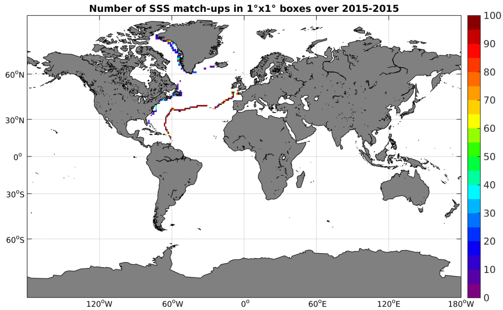
Figure 4: Number of SSS match-ups between TSG-GOSUD-Sailing-ship SSS and the SMAP-L3-JPL-V4-8DAY-RUNNING-60KM SSS product for the Global Ocean Pi-MEP region over 1^\circ \times 1^\circ boxes and for the full satellite product period.
