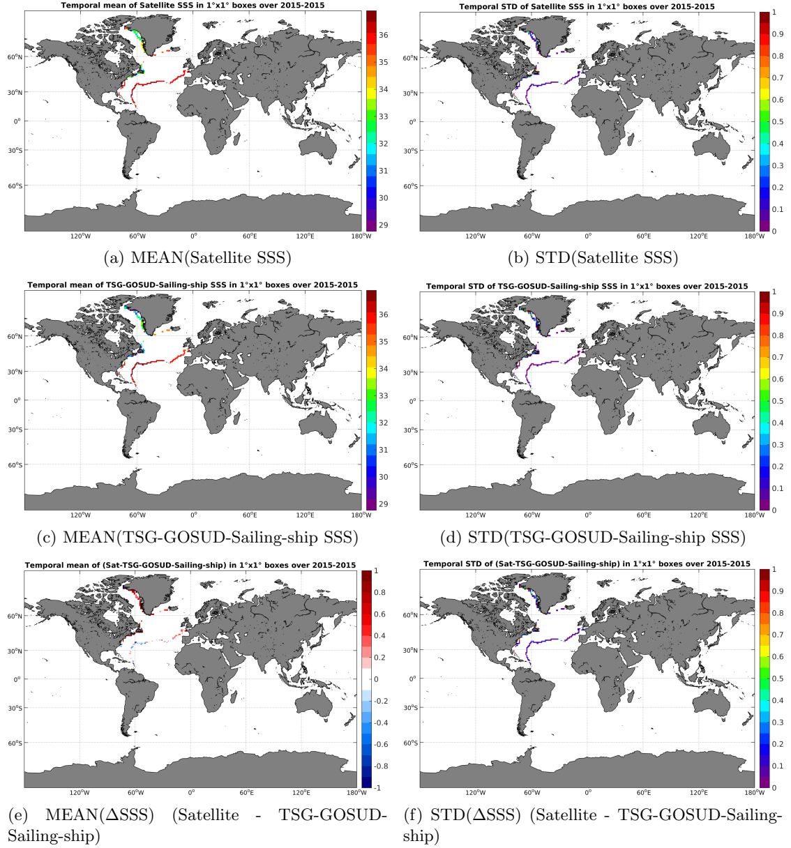
Figure 6: Temporal mean (left) and STD (right) of SSS from SMAP-L3-JPL-V4-8DAY-RUNNING-60KM (top), TSG-GOSUD-Sailing-ship (middle), and of \Delta SSS (Satellite - TSG-GOSUD-Sailing-ship). Only match-up pairs are used to generate these maps.
