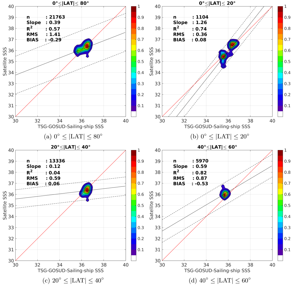
Figure 9: Contour maps of the concentration of SMAP-L3-JPL-V4-8DAY-RUNNING-60KM SSS (y-axis) versus TSG-GOSUD-Sailing-ship SSS (x-axis) at match-up pairs for different latitude bands. For each plot, the red line shows x=y . The black thin and dashed lines indicate a linear fit through the data cloud and the \pm 95\% confidence levels, respectively. The number match-up pairs n , the slope and R^2 coefficient of the linear fit, the root mean square (RMS) and the mean bias between satellite and in situ data are indicated for each latitude band in each plots.
