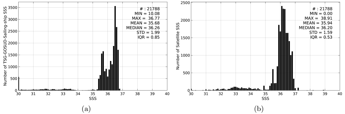
Figure 2: Histograms of SSS from TSG-GOSUD-Sailing-ship (a) and SMAP-L3-JPL-V4-8DAY-RUNNING-60KM (b) considering all match-up pairs per bins of 0.1 over the Global Ocean Pi-MEP region and for the full satellite product period.
