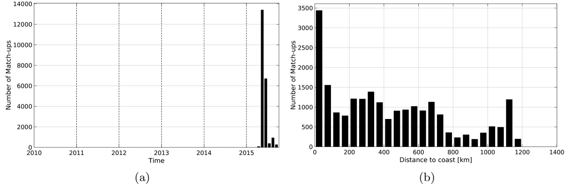
Figure 1: Number of match-ups between TSG-GOSUD-Sailing-ship and SMAP-L3-JPL-V4-8DAY-RUNNING-60KM SSS as a function of time (a) and as function of the distance to coast (b) over the Global Ocean Pi-MEP region and for the full satellite product period.
