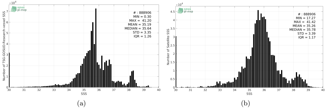
Figure 2: Histograms of SSS from TSG-GOSUD-Research-vessel (a) and SMAP-L3-JPL-V4-8DAY-RUNNING-60KM (b) considering all match-up pairs per bins of 0.1 over the Global Ocean Pi-MEP region and for the full satellite product period.
