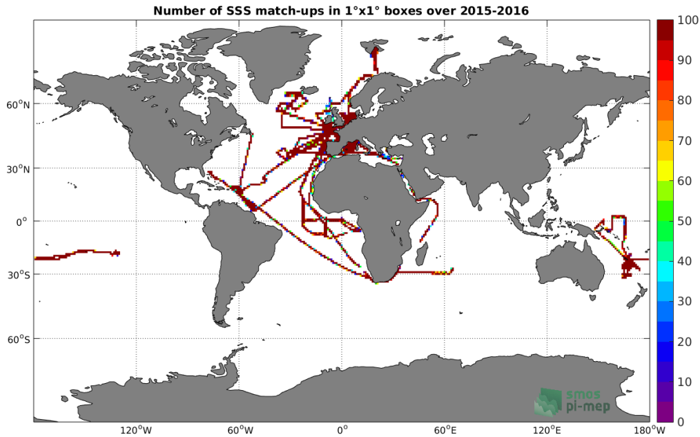
Figure 4: Number of SSS match-ups between TSG-GOSUD-Research-vessel SSS and the SMAP-L3-JPL-V4-8DAY-RUNNING-60KM SSS product for the Global Ocean Pi-MEP region over 1°x1° boxes and for the full satellite product period.
