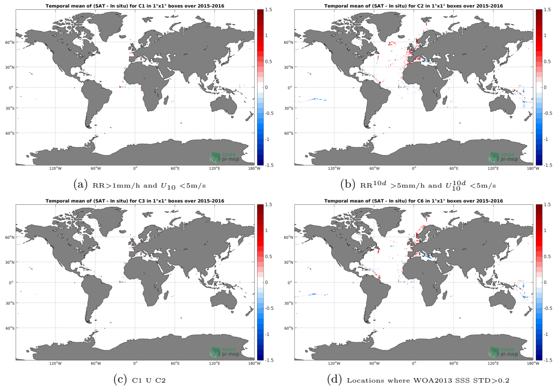
Figure 12: Temporal mean gridded over spatial boxes of size 1^\circ \times 1^\circ of \Delta SSS (SMAP-L3-JPL-V4-8DAY-RUNNING-60KM - TSG-GOSUD-Research-vessel) for 4 different subdatasets corresponding to: RR > 1mm/h and U_{10} < 5\text{m/s} (a), RR^{10d} > 5\text{mm/h} and U_{10}^{10d} < 5\text{m/s} (b), C1 U C2 (c), Locations where WOA2013 SSS STD > 0.2 (d).
