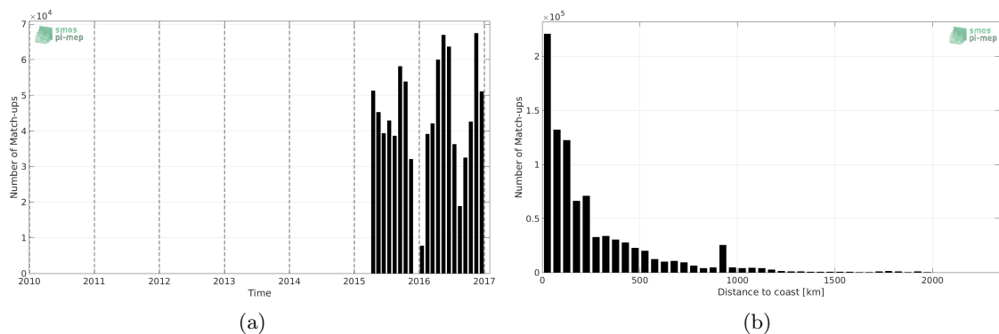
Figure 1: Number of match-ups between TSG-GOSUD-Research-vessel and SMAP-L3-JPL-V4-8DAY-RUNNING-60KM SSS as a function of time (a) and as function of the distance to coast (b) over the Global Ocean Pi-MEP region and for the full satellite product period.
