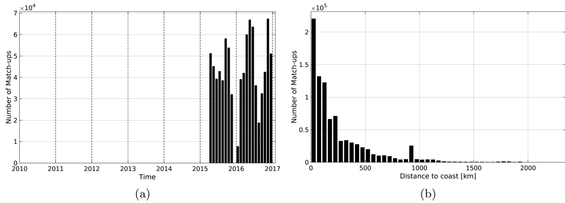
Figure 1: Number of match-ups between TSG-GOSUD-Research-vessel and SMAP-L3-JPL-V4-8DAY-RUNNING-60KM SSS as a function of time (a) and as function of the distance to coast (b) over the Global Ocean Pi-MEP region and for the full satellite product period.
