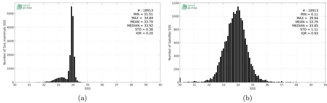
Figure 2: Histograms of SSS from Sea mammals (a) and SMAP-L3-JPL-V4-8DAY-RUNNING-60KM (b) considering all match-up pairs per bins of 0.1 over the Global Ocean Pi-MEP region and for the full satellite product period.
