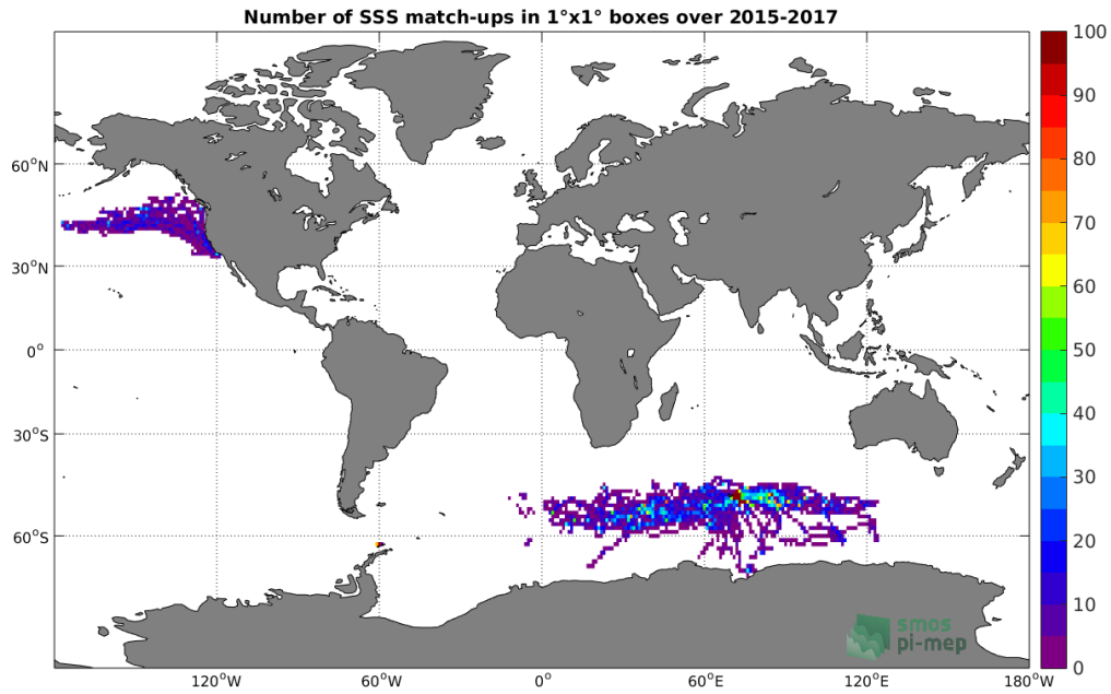
Figure 4: Number of SSS match-ups between Sea mammals SSS and the SMAP-L3-JPL-V4-8DAY-RUNNING-60KM SSS product for the Global Ocean Pi-MEP region over 1^\circ \times 1^\circ boxes and for the full satellite product period.
