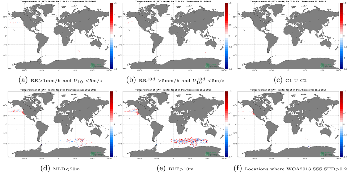
Figure 12: Temporal mean gridded over spatial boxes of size 1^\circ \times 1^\circ of \Delta\text{SSS} (SMAP-L3-JPL-V4-8DAY-RUNNING-60KM - Sea mammals) for 6 different subdatasets corresponding to: RR > 1\text{mm/h} and U_{10} < 5\text{m/s} (a), RR^{10d} > 5\text{mm/h} and U_{10}^{10d} < 5\text{m/s} (b), C1 U C2 (c), MLD < 20\text{m} (d), BLT > 10\text{m} (e), Locations where WOA2013 SSS STD > 0.2 (f).
