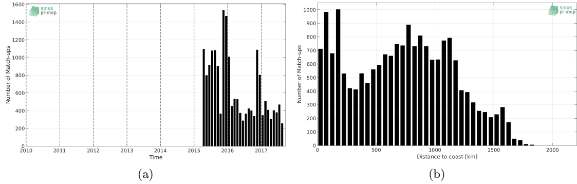
Figure 1: Number of match-ups between Sea mammals and SMAP-L3-JPL-V4-8DAY-RUNNING-60KM SSS as a function of time (a) and as function of the distance to coast (b) over the Global Ocean Pi-MEP region and for the full satellite product period.
