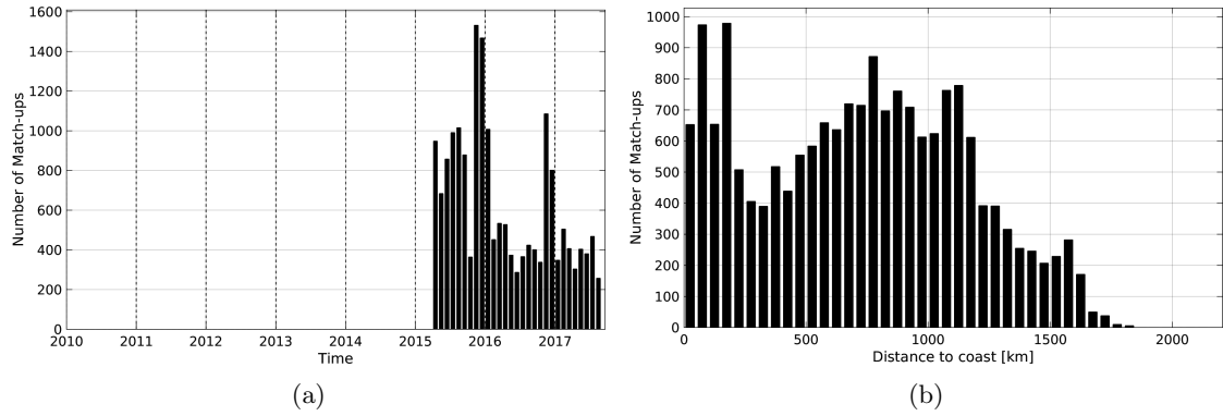
Figure 1: Number of match-ups between Sea mammals and SMAP-L3-JPL-V4-8DAY-RUNNING-60KM SSS as a function of time (a) and as function of the distance to coast (b) over the Global Ocean Pi-MEP region and for the full satellite product period.
