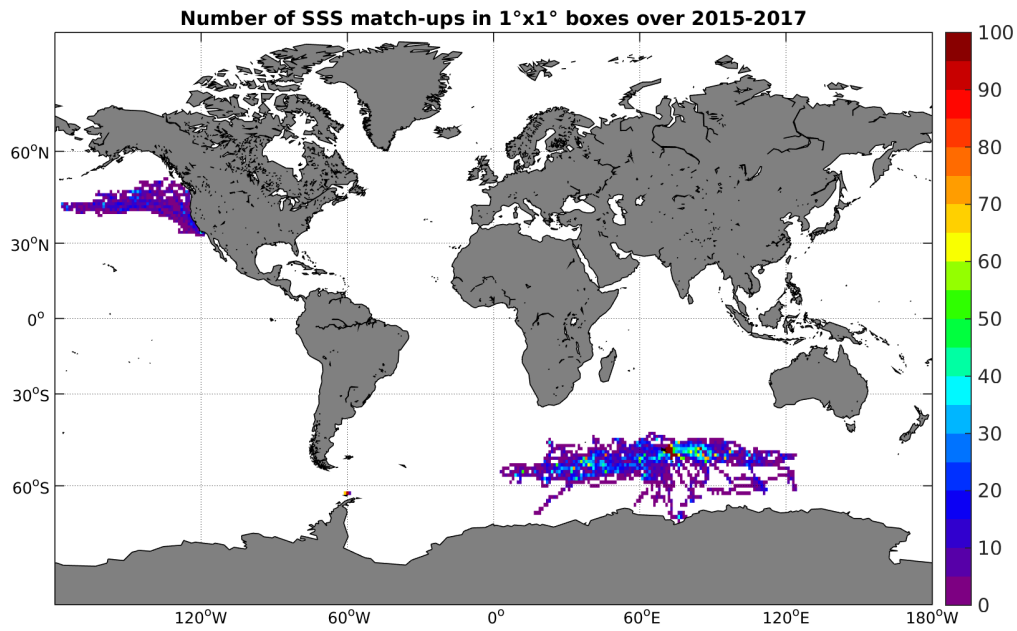
Figure 4: Number of SSS match-ups between Sea mammals SSS and the SMAP-L3-JPL-V4-8DAY-RUNNING-60KM SSS product for the Global Ocean Pi-MEP region over 1^\circ \times 1^\circ boxes and for the full satellite product period.
