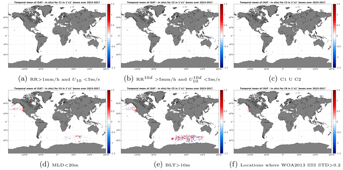
Figure 12: Temporal mean gridded over spatial boxes of size 1^\circ \times 1^\circ of \Delta SSS (SMAP-L3-JPL-V4-8DAY-RUNNING-60KM - Sea mammals) for 6 different subdatasets corresponding to: RR > 1\text{mm/h} and U_{10} < 5\text{m/s} (a), RR^{10d} > 5\text{mm/h} and U_{10}^{10d} < 5\text{m/s} (b), C1 U C2 (c), MLD < 20\text{m} (d), BLT > 10\text{m} (e), Locations where WOA2013 SSS STD > 0.2 (f).
