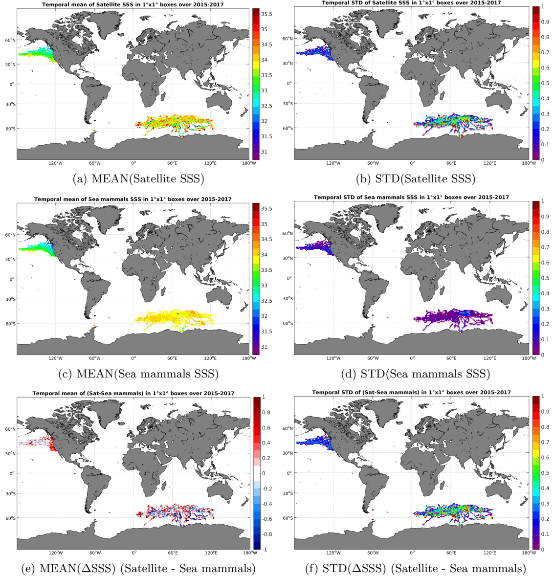
Figure 6: Temporal mean (left) and STD (right) of SSS from SMAP-L3-JPL-V4-8DAY-RUNNING-60KM (top), Sea mammals (middle), and of \Delta SSS (Satellite - Sea mammals). Only match-up pairs are used to generate these maps.
