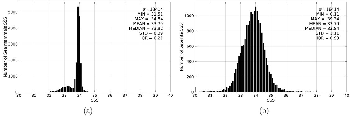
Figure 2: Histograms of SSS from Sea mammals (a) and SMAP-L3-JPL-V4-8DAY-RUNNING-60KM (b) considering all match-up pairs per bins of 0.1 over the Global Ocean Pi-MEP region and for the full satellite product period.
