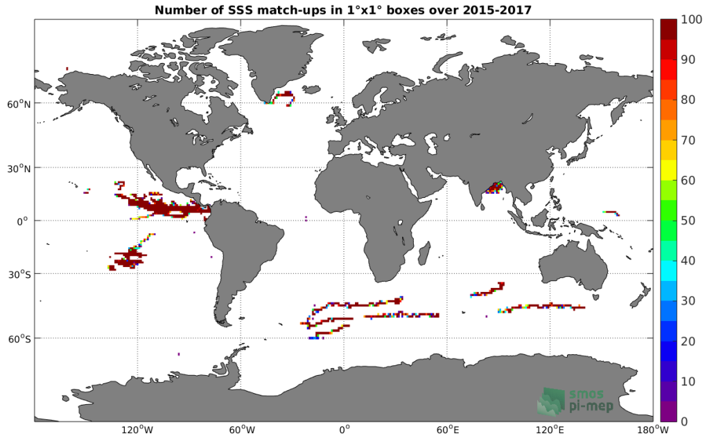
Figure 3: Number of SSS match-ups between Surface drifters SSS and the SMAP-L3-JPL-V4-8DAY-RUNNING-60KM SSS product for the Global Ocean Pi-MEP region over 1°x1° boxes and for the full satellite product period.
