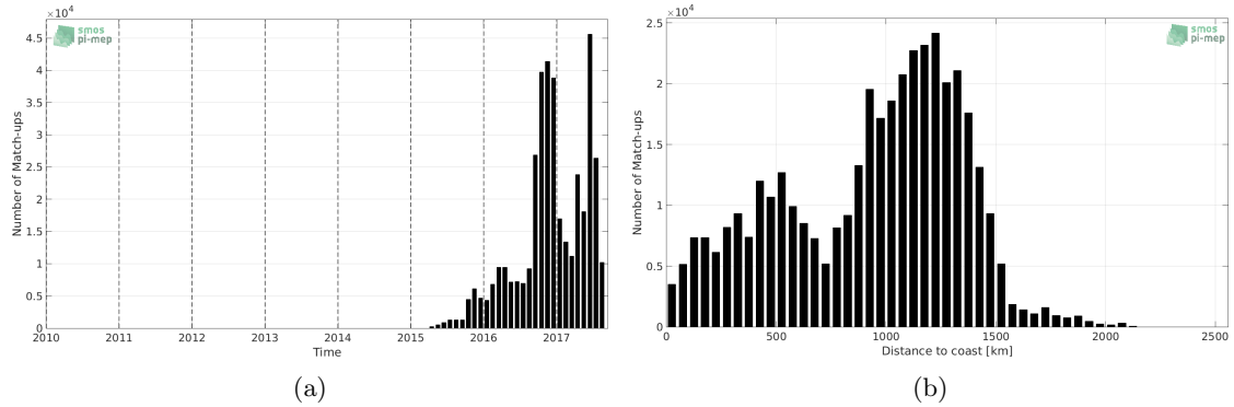
Figure 1: Number of match-ups between Surface drifters and SMAP-L3-JPL-V4-8DAY-RUNNING-60KM SSS as a function of time (a) and as function of the distance to coast (b) over the Global Ocean Pi-MEP region and for the full satellite product period.
