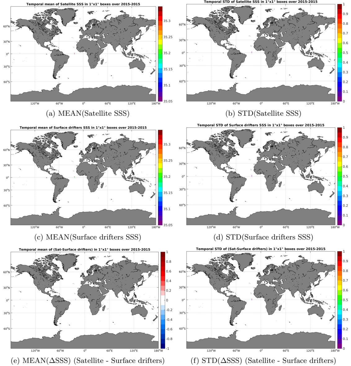
Figure 5: Temporal mean (left) and STD (right) of SSS from SMAP-L3-JPL-V4-8DAY-RUNNING-60KM (top), Surface drifters (middle), and of \Delta SSS (Satellite - Surface drifters). Only match-up pairs are used to generate these maps.
