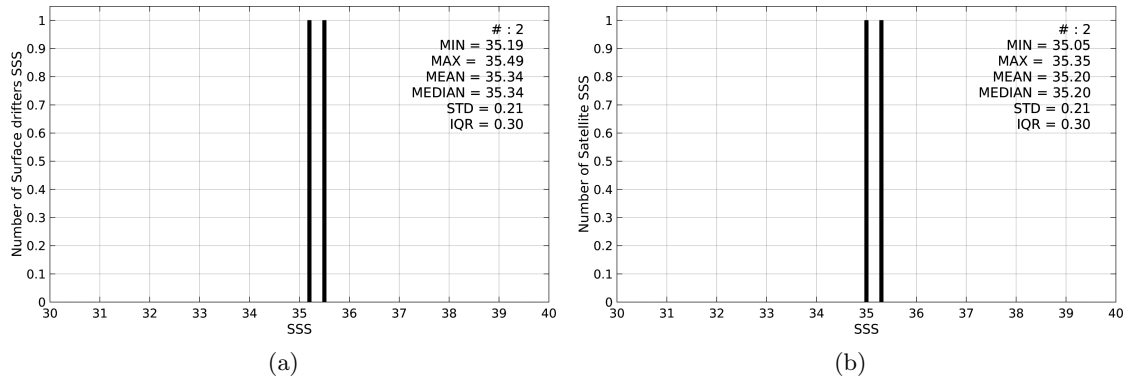
Figure 2: Histograms of SSS from Surface drifters (a) and SMAP-L3-JPL-V4-8DAY-RUNNING-60KM (b) considering all match-up pairs per bins of 0.1 over the Global Ocean Pi-MEP region and for the full satellite product period.
