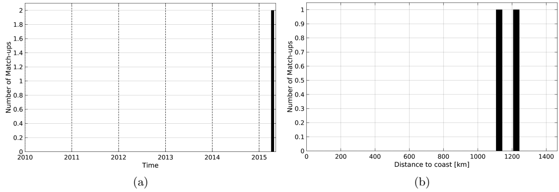
Figure 1: Number of match-ups between Surface drifters and SMAP-L3-JPL-V4-8DAY-RUNNING-60KM SSS as a function of time (a) and as function of the distance to coast (b) over the Global Ocean Pi-MEP region and for the full satellite product period.
