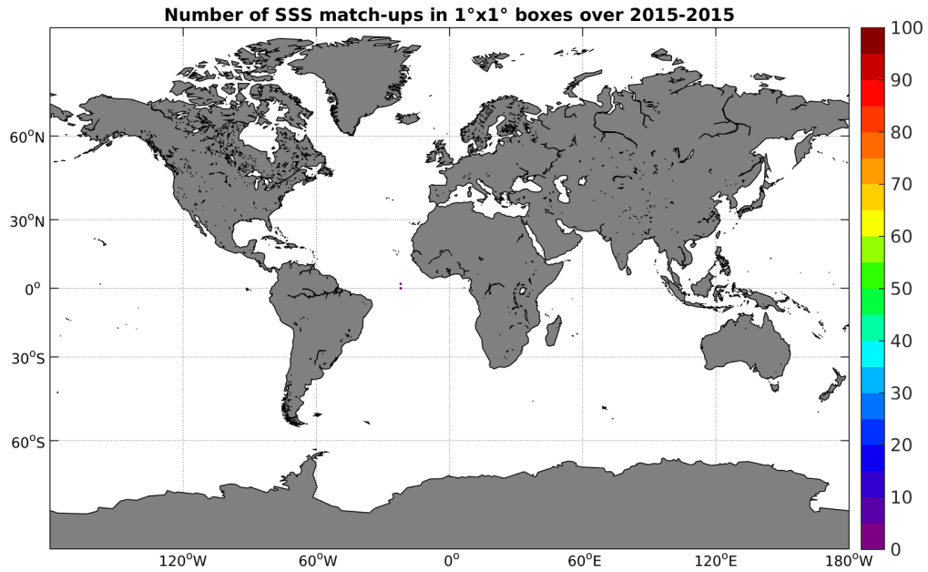
Figure 3: Number of SSS match-ups between Surface drifters SSS and the SMAP-L3-JPL-V4-8DAY-RUNNING-60KM SSS product for the Global Ocean Pi-MEP region over 1°x1° boxes and for the full satellite product period.
