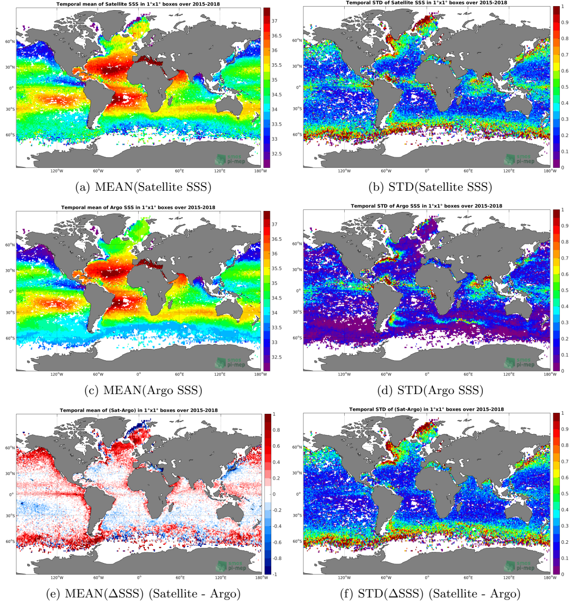
Figure 6: Temporal mean (left) and STD (right) of SSS from SMAP-L3-JPL-V4-8DAY-RUNNING-60KM (top), Argo (middle), and of \Delta SSS (Satellite - Argo). Only match-up pairs are used to generate these maps.
