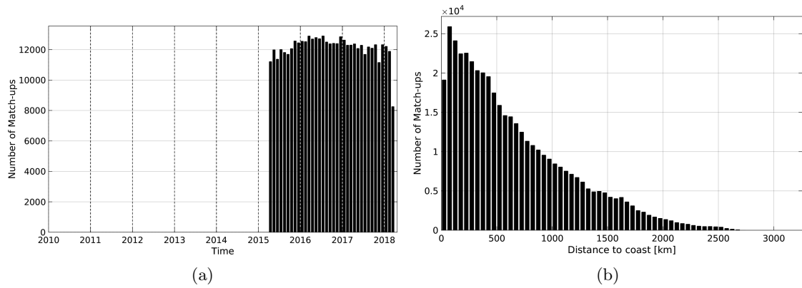
Figure 1: Number of match-ups between Argo and SMAP-L3-JPL-V4-8DAY-RUNNING-60KM SSS as a function of time (a) and as function of the distance to coast (b) over the Global Ocean Pi-MEP region and for the full satellite product period.
