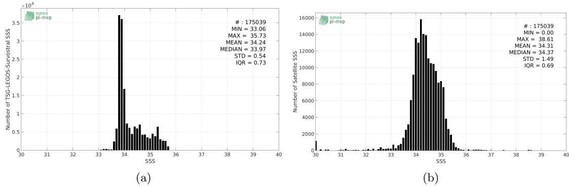
Figure 2: Histograms of SSS from TSG-LEGOS-Survostral (a) and SMAP-L3-JPL-V4-MONTHLY-60KM (b) considering all match-up pairs per bins of 0.1 over the Global Ocean Pi-MEP region and for the full satellite product period.
