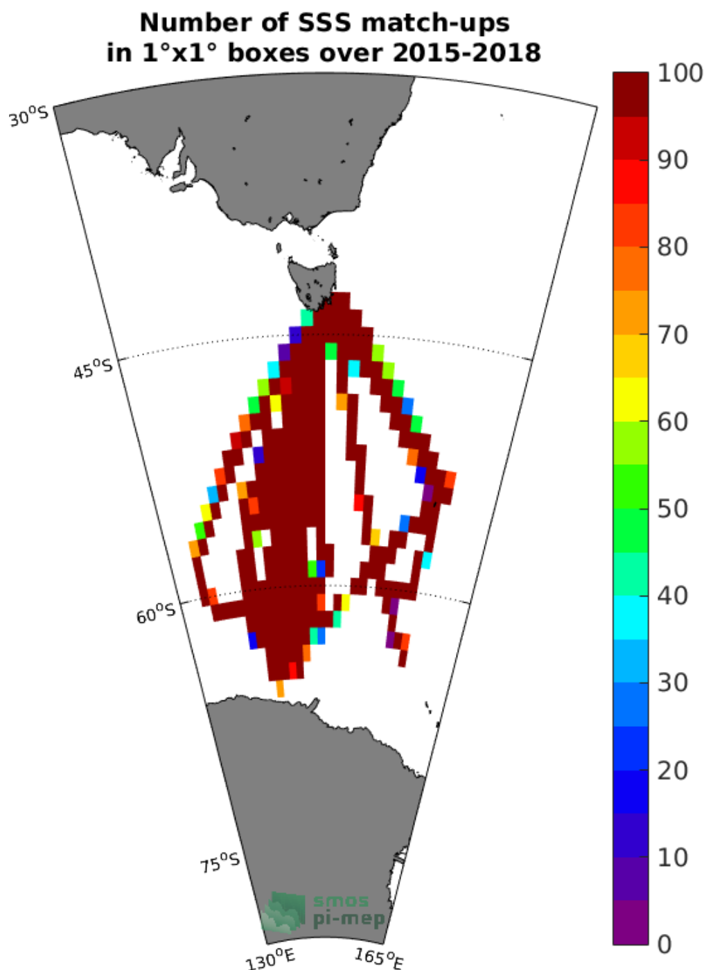
Figure 4: Number of SSS match-ups between TSG-LEGOS-Survostral SSS and the SMAP-L3-JPL-V4-MONTHLY-60KM SSS product for the Global Ocean Pi-MEP region over 1°x1° boxes and for the full satellite product period.
