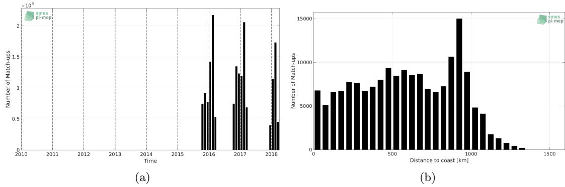
Figure 1: Number of match-ups between TSG-LEGOS-Survostral and SMAP-L3-JPL-V4-MONTHLY-60KM SSS as a function of time (a) and as function of the distance to coast (b) over the Global Ocean Pi-MEP region and for the full satellite product period.
