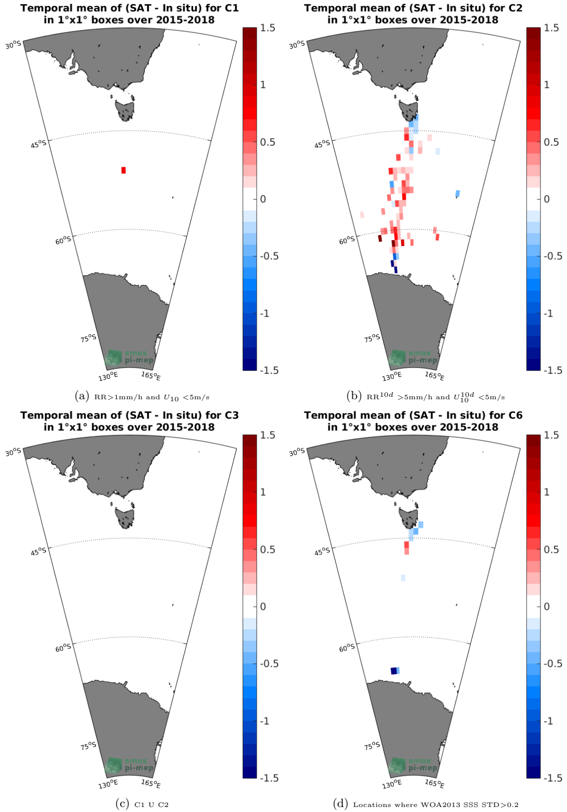
Figure 12: Temporal mean gridded over spatial boxes of size 1°x1° of \Delta\text{SSS} (SMAP-L3-JPL-V4-MONTHLY-60KM - TSG-LEGOS-Survostral) for 4 different subdatasets corresponding to: RR > 1\text{mm/h} and U_{10} < 5\text{m/s} (a), RR^{10d} > 5\text{mm/h} and U_{10}^{10d} < 5\text{m/s} (b), C1 U C2 (c), Locations where WOA2013 SSS STD > 0.2 (d).
