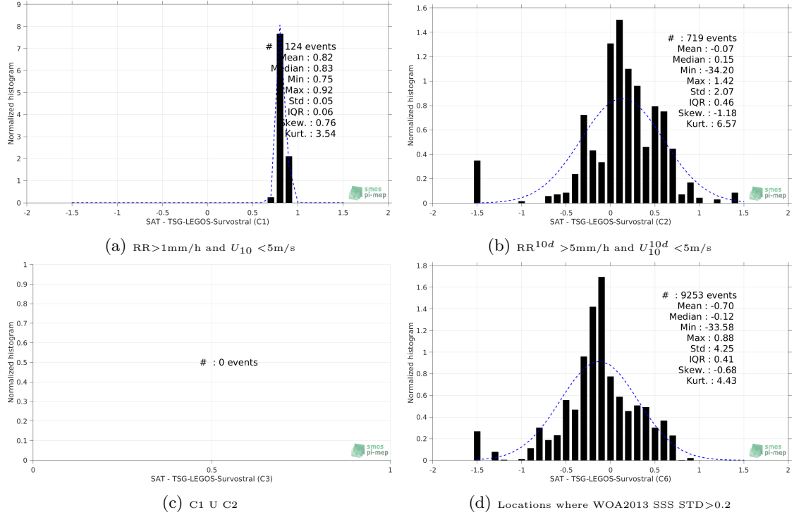
Figure 13: Normalized histogram of \Delta\text{SSS} (SMAP-L3-JPL-V4-MONTHLY-60KM - TSG-LEGOS-Survostral) for 6 different subdatasets corresponding to: RR > 1\text{mm/h} and U_{10} < 5\text{m/s} (a), RR^{10d} > 5\text{mm/h} and U_{10}^{10d} < 5\text{m/s} (b), C1 \cup C2 (c), Locations where WOA2013 SSS STD > 0.2 (d).
