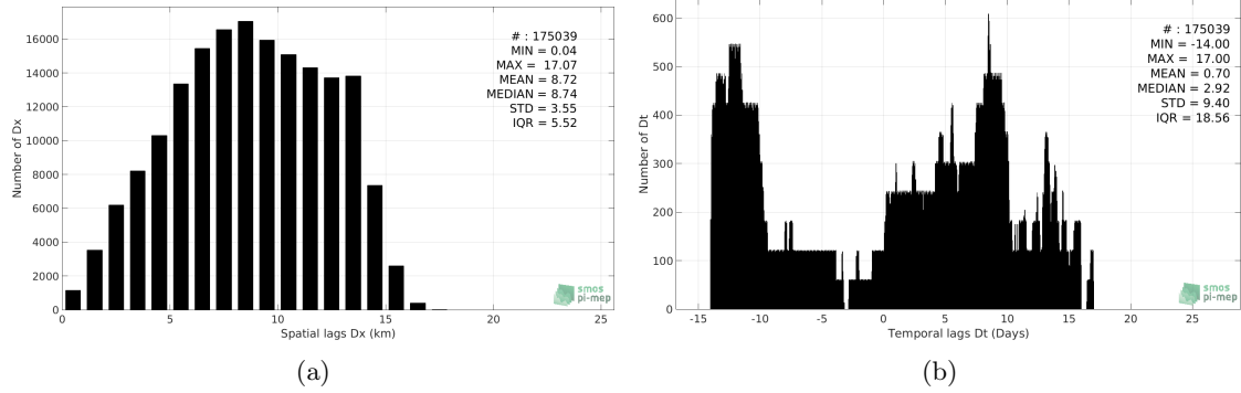
Figure 5: Histograms of the spatial (a) and temporal (b) lags between the time of the TSG-LEGOS-Survostral measurements and the date of the corresponding SMAP-L3-JPL-V4-MONTHLY-60KM SSS product.
