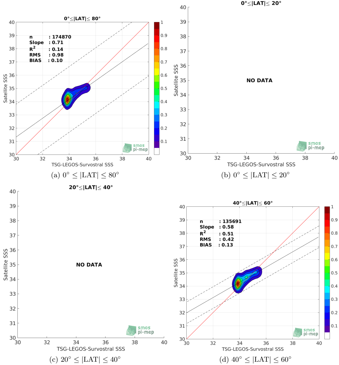
Figure 9: Contour maps of the concentration of SMAP-L3-JPL-V4-MONTHLY-60KM SSS (y-axis) versus TSG-LEGOS-Survostral SSS (x-axis) at match-up pairs for different latitude bands. For each plot, the red line shows x=y . The black thin and dashed lines indicate a linear fit through the data cloud and the \pm 95\% confidence levels, respectively. The number match-up pairs n , the slope and R^2 coefficient of the linear fit, the root mean square (RMS) and the mean bias between satellite and in situ data are indicated for each latitude band in each plots.
