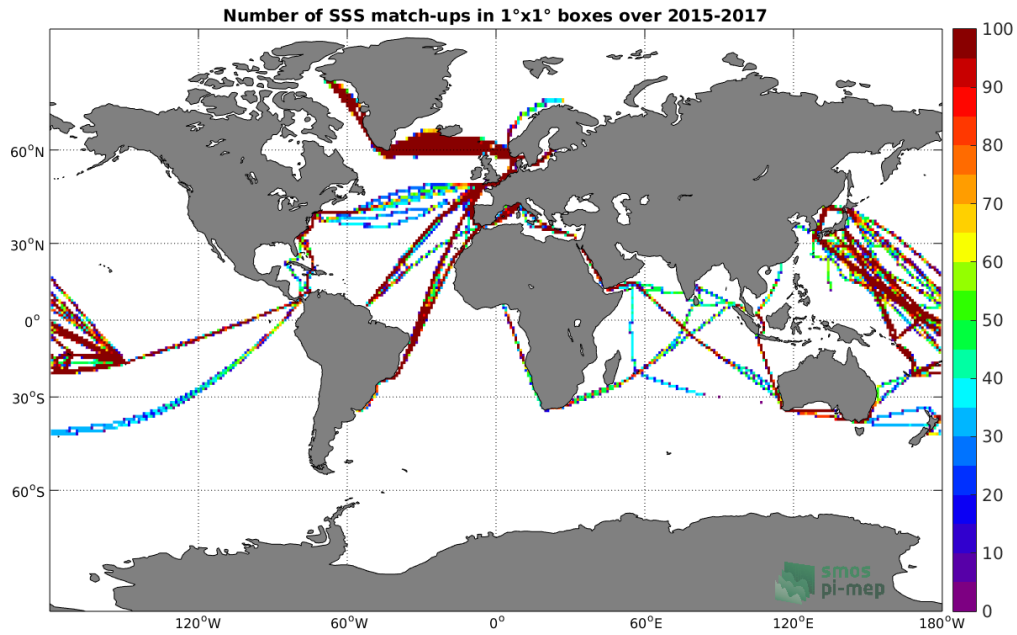
Figure 4: Number of SSS match-ups between TSG-LEGOS-DM SSS and the SMAP-L3-JPL-V4-MONTHLY-60KM SSS product for the Global Ocean Pi-MEP region over 1°x1° boxes and for the full satellite product period.
