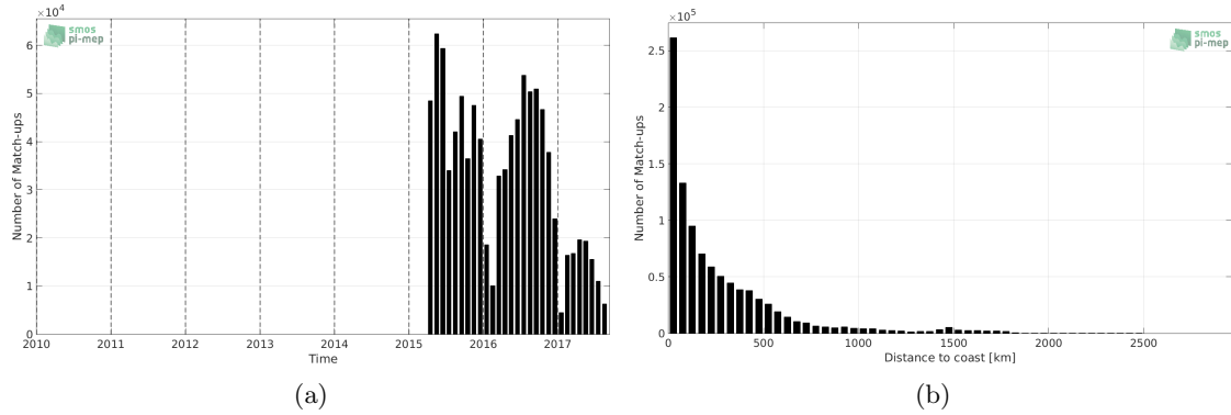
Figure 1: Number of match-ups between TSG-LEGOS-DM and SMAP-L3-JPL-V4-MONTHLY-60KM SSS as a function of time (a) and as function of the distance to coast (b) over the Global Ocean Pi-MEP region and for the full satellite product period.
