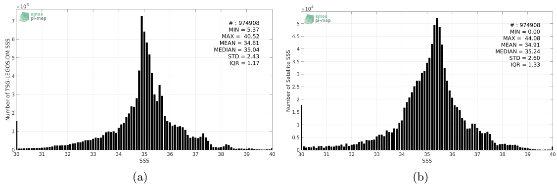
Figure 2: Histograms of SSS from TSG-LEGOS-DM (a) and SMAP-L3-JPL-V4-MONTHLY-60KM (b) considering all match-up pairs per bins of 0.1 over the Global Ocean Pi-MEP region and for the full satellite product period.
