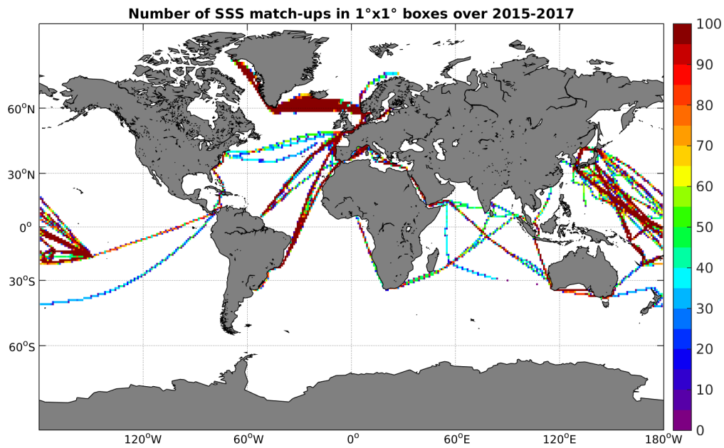
Figure 4: Number of SSS match-ups between TSG-LEGOS-DM SSS and the SMAP-L3-JPL-V4-MONTHLY-60KM SSS product for the Global Ocean Pi-MEP region over 1°x1° boxes and for the full satellite product period.
