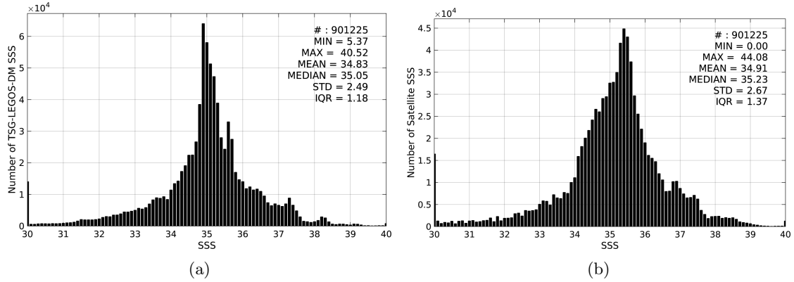
Figure 2: Histograms of SSS from TSG-LEGOS-DM (a) and SMAP-L3-JPL-V4-MONTHLY-60KM (b) considering all match-up pairs per bins of 0.1 over the Global Ocean Pi-MEP region and for the full satellite product period.
