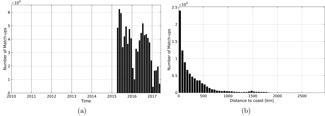
Figure 1: Number of match-ups between TSG-LEGOS-DM and SMAP-L3-JPL-V4-MONTHLY-60KM SSS as a function of time (a) and as function of the distance to coast (b) over the Global Ocean Pi-MEP region and for the full satellite product period.
