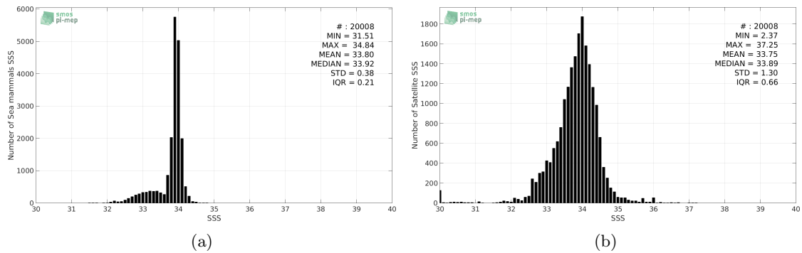
Figure 2: Histograms of SSS from Sea mammals (a) and SMAP-L3-JPL-V4-MONTHLY-60KM (b) considering all match-up pairs per bins of 0.1 over the Global Ocean Pi-MEP region and for the full satellite product period.
