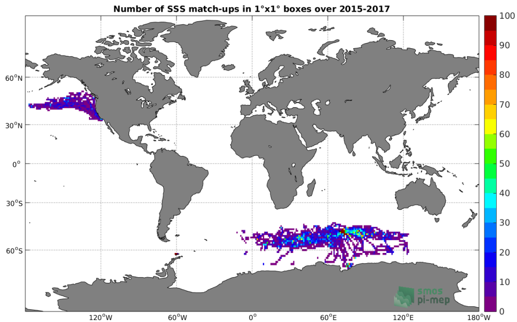
Figure 4: Number of SSS match-ups between Sea mammals SSS and the SMAP-L3-JPL-V4-MONTHLY-60KM SSS product for the Global Ocean Pi-MEP region over 1^\circ \times 1^\circ boxes and for the full satellite product period.
