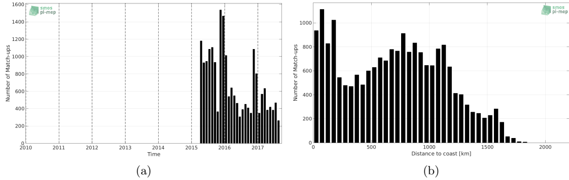
Figure 1: Number of match-ups between Sea mammals and SMAP-L3-JPL-V4-MONTHLY-60KM SSS as a function of time (a) and as function of the distance to coast (b) over the Global Ocean Pi-MEP region and for the full satellite product period.
