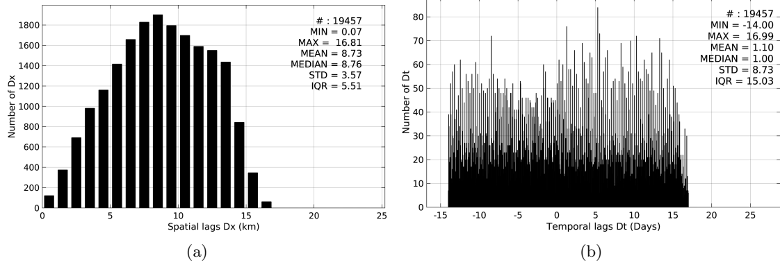
Figure 5: Histograms of the spatial (a) and temporal (b) lags between the time of the Sea mammals measurements and the date of the corresponding SMAP-L3-JPL-V4-MONTHLY-60KM SSS product.
