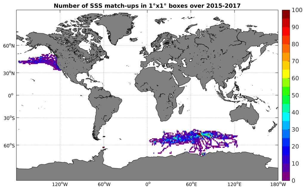
Figure 4: Number of SSS match-ups between Sea mammals SSS and the SMAP-L3-JPL-V4-MONTHLY-60KM SSS product for the Global Ocean Pi-MEP region over 1^\circ \times 1^\circ boxes and for the full satellite product period.
