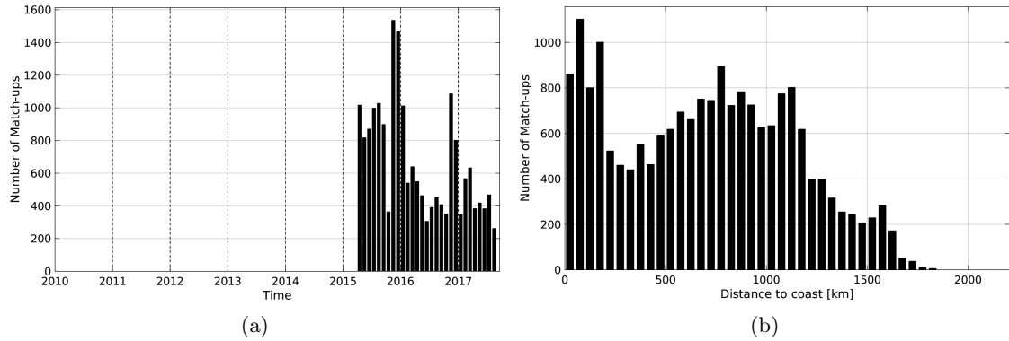
Figure 1: Number of match-ups between Sea mammals and SMAP-L3-JPL-V4-MONTHLY-60KM SSS as a function of time (a) and as function of the distance to coast (b) over the Global Ocean Pi-MEP region and for the full satellite product period.
