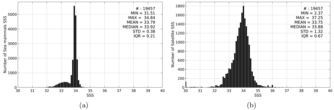
Figure 2: Histograms of SSS from Sea mammals (a) and SMAP-L3-JPL-V4-MONTHLY-60KM (b) considering all match-up pairs per bins of 0.1 over the Global Ocean Pi-MEP region and for the full satellite product period.
