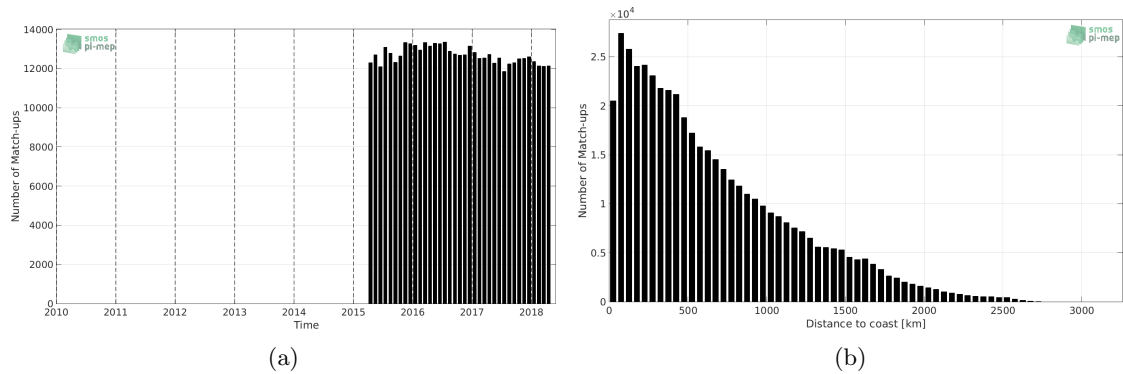
Figure 1: Number of match-ups between Argo and SMAP-L3-JPL-V4-MONTHLY-60KM SSS as a function of time (a) and as function of the distance to coast (b) over the Global Ocean Pi-MEP region and for the full satellite product period.
