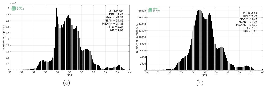
Figure 2: Histograms of SSS from Argo (a) and SMAP-L3-JPL-V4-MONTHLY-60KM (b) considering all match-up pairs per bins of 0.1 over the Global Ocean Pi-MEP region and for the full satellite product period.
