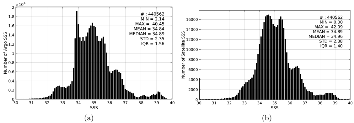
Figure 2: Histograms of SSS from Argo (a) and SMAP-L3-JPL-V4-MONTHLY-60KM (b) considering all match-up pairs per bins of 0.1 over the Global Ocean Pi-MEP region and for the full satellite product period.
