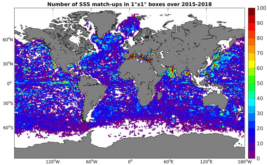
Figure 4: Number of SSS match-ups between Argo SSS and the SMAP-L3-JPL-V4-MONTHLY-60KM SSS product for the Global Ocean Pi-MEP region over 1^\circ \times 1^\circ boxes and for the full satellite product period.
