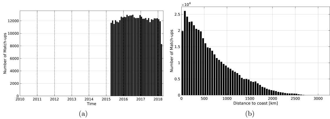
Figure 1: Number of match-ups between Argo and SMAP-L3-JPL-V4-MONTHLY-60KM SSS as a function of time (a) and as function of the distance to coast (b) over the Global Ocean Pi-MEP region and for the full satellite product period.
