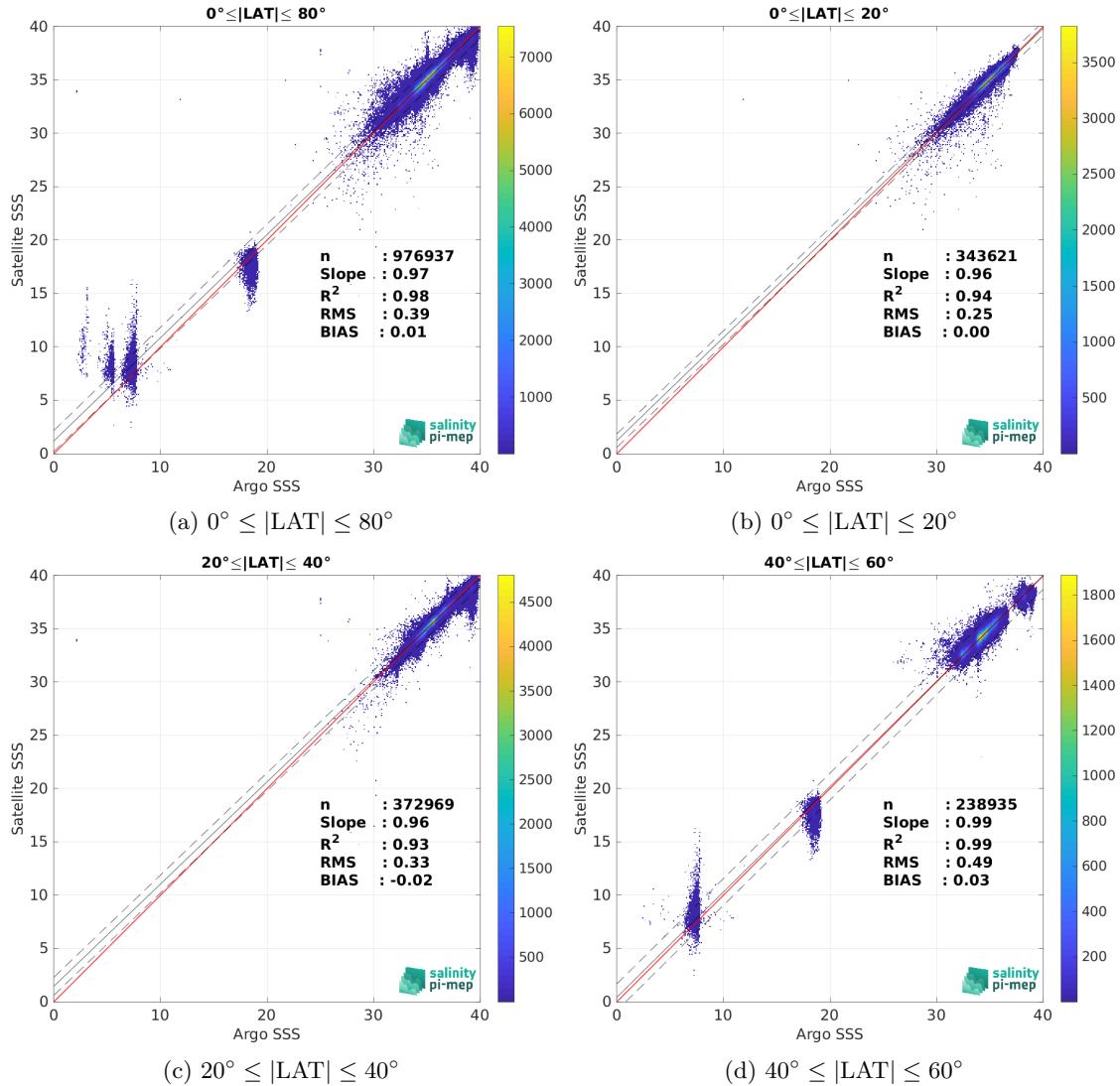
Figure 9: Contour maps of the concentration of SMAP SSS L2-AVERAGED v5 (RSS) SSS (y-axis) versus Argo SSS (x-axis) at match-up pairs for different latitude bands. For each plot, the red line shows x=y . The black thin and dashed lines indicate a linear fit through the data cloud and the \pm 95\% confidence levels, respectively. The number match-up pairs n , the slope and R^2 coefficient of the linear fit, the root mean square (RMS) and the mean bias between satellite and in situ data are indicated for each latitude band in each plots.
