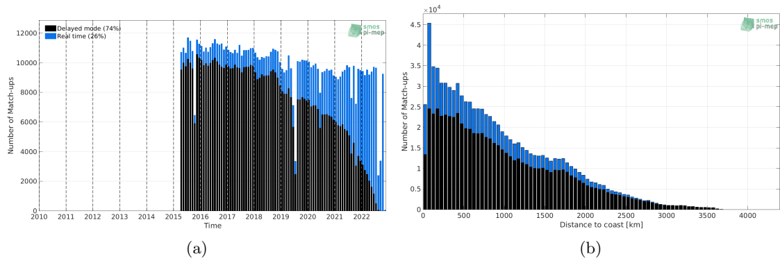
Figure 1: Number of match-ups between Argo and SMAP SSS L2-AVERAGED v5 (RSS) SSS as a function of time (a) and as function of the distance to coast (b) over the Global Ocean Pi-MEP region and for the full satellite product period.
