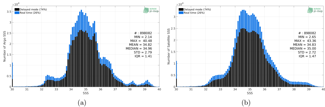
Figure 2: Histograms of SSS from Argo (a) and SMAP SSS L2-AVERAGED v5 (RSS) (b) considering all match-up pairs per bins of 0.1 over the Global Ocean Pi-MEP region and for the full satellite product period.
