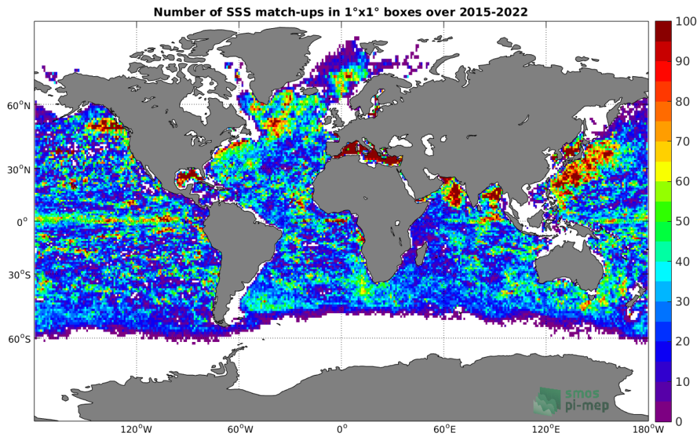
Figure 4: Number of SSS match-ups between Argo SSS and the SMAP SSS L2-AVERAGED v5 (RSS) SSS product for the Global Ocean Pi-MEP region over 1^\circ \times 1^\circ boxes and for the full satellite product period.
