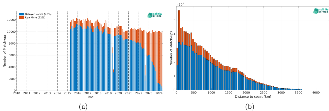
Figure 2: Number of match-ups between Argo and SMAP SSS L2-AVERAGED v5.0 (JPL) SSS as a function of time (a) and as function of the distance to coast (b) over the Global Ocean Pi-MEP region and for the full satellite product period.
