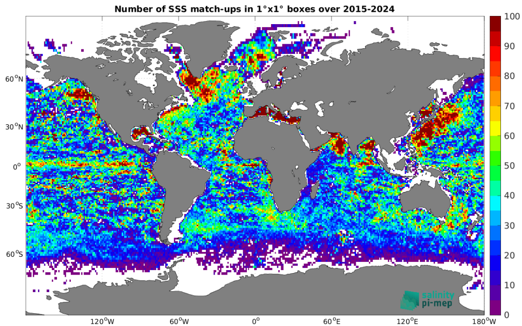
Figure 5: Number of SSS match-ups between Argo SSS and the SMAP SSS L2-AVERAGED v5.0 (JPL) SSS product for the Global Ocean Pi-MEP region over 1^\circ \times 1^\circ boxes and for the full satellite product period.
