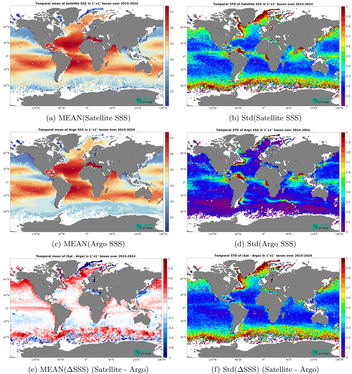
Figure 7: Temporal mean (left) and Std (right) of SSS from SMAP SSS L2-AVERAGED v5.0 (JPL) (top), Argo (middle), and of \Delta SSS (Satellite - Argo). Only match-up pairs are used to generate these maps.
