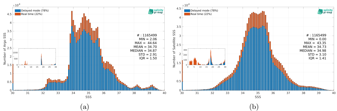
Figure 3: Histograms of SSS from Argo (a) and SMAP SSS L2-AVERAGED v5.0 (JPL) (b) considering all match-up pairs per bins of 0.1 over the Global Ocean Pi-MEP region and for the full satellite product period.
