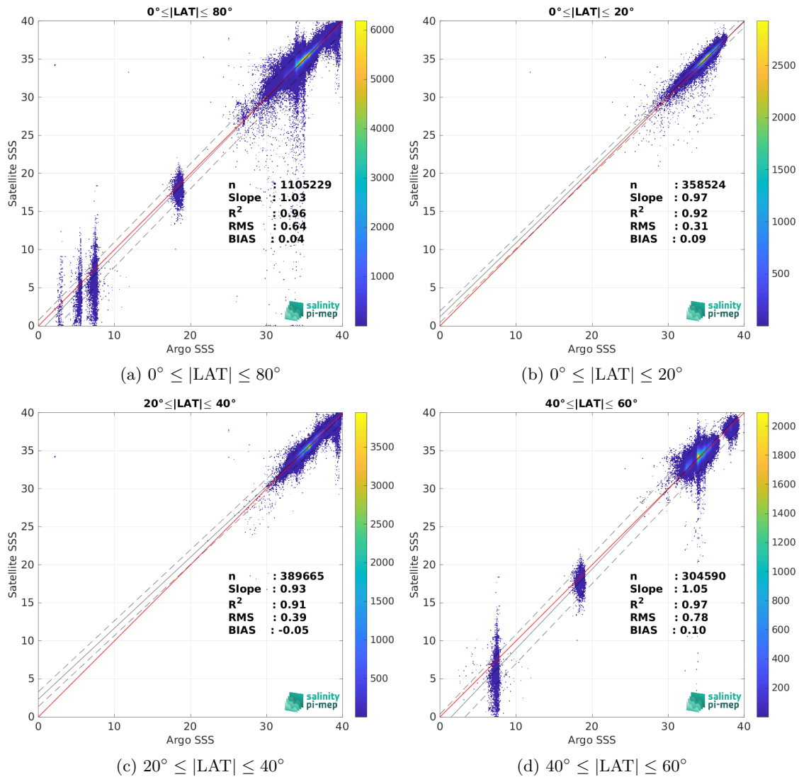
Figure 9: Contour maps of the concentration of SMAP SSS L2-AVERAGED v5.0 (JPL) SSS (y-axis) versus Argo SSS (x-axis) at match-up pairs for different latitude bands. For each plot, the red line shows x=y . The black thin and dashed lines indicate a linear fit through the data cloud and the \pm 95\% confidence levels, respectively. The number match-up pairs n , the slope and R^2 coefficient of the linear fit, the root mean square (RMS) and the mean bias between satellite and in situ data are indicated for each latitude band in each plot.
