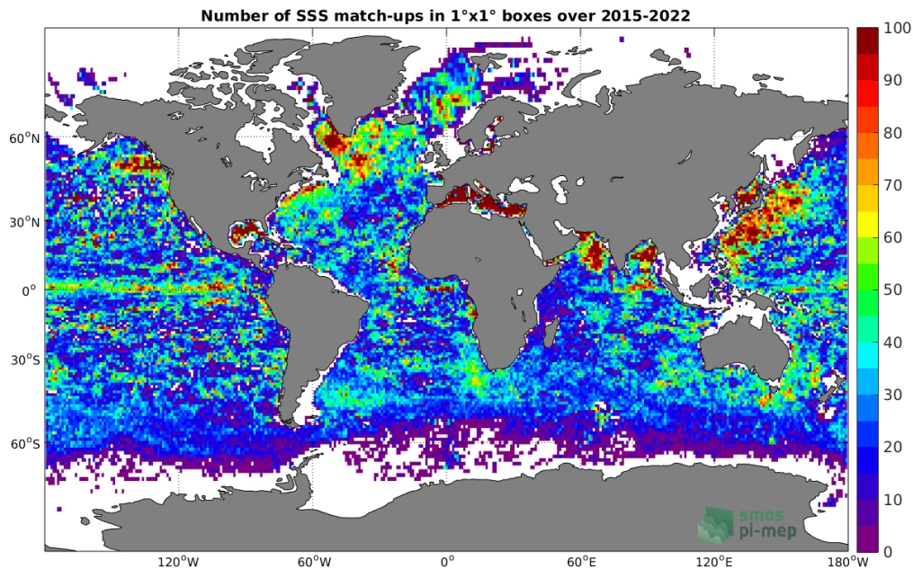
Figure 4: Number of SSS match-ups between Argo SSS and the SMAP SSS L2-AVERAGED v5.0 (JPL) SSS product for the Global Ocean Pi-MEP region over 1^\circ \times 1^\circ boxes and for the full satellite product period.
