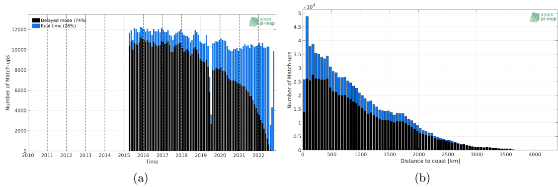
Figure 1: Number of match-ups between Argo and SMAP SSS L2-AVERAGED v5.0 (JPL) SSS as a function of time (a) and as function of the distance to coast (b) over the Global Ocean Pi-MEP region and for the full satellite product period.
