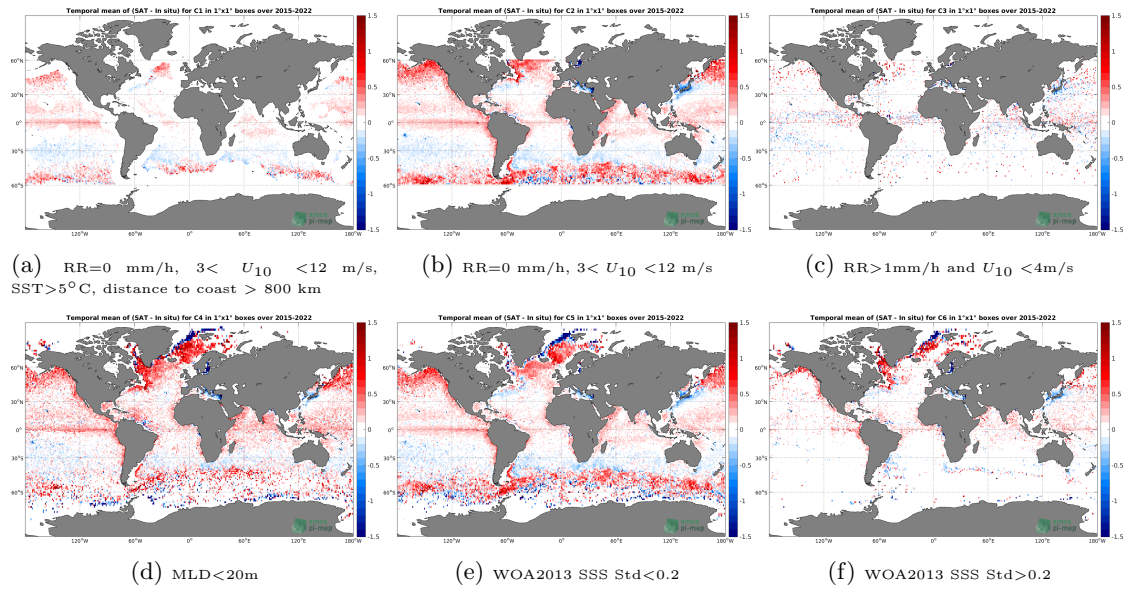
Figure 12: Temporal mean gridded over spatial boxes of size 1^\circ \times 1^\circ of \Delta SSS (SMAP SSS L2-AVERAGED v5.0 (JPL) - Argo) for 6 different subdatasets corresponding to:RR=0 mm/h, 3 < U_{10} < 12 m/s, SST > 5^\circ\text{C} , distance to coast > 800 km (a), RR=0 mm/h, 3 < U_{10} < 12 m/s (b), RR > 1 mm/h and U_{10} < 4 m/s (c),MLD < 20 m (d),WOA2013 SSS Std < 0.2 (e),WOA2013 SSS Std > 0.2 (f).
