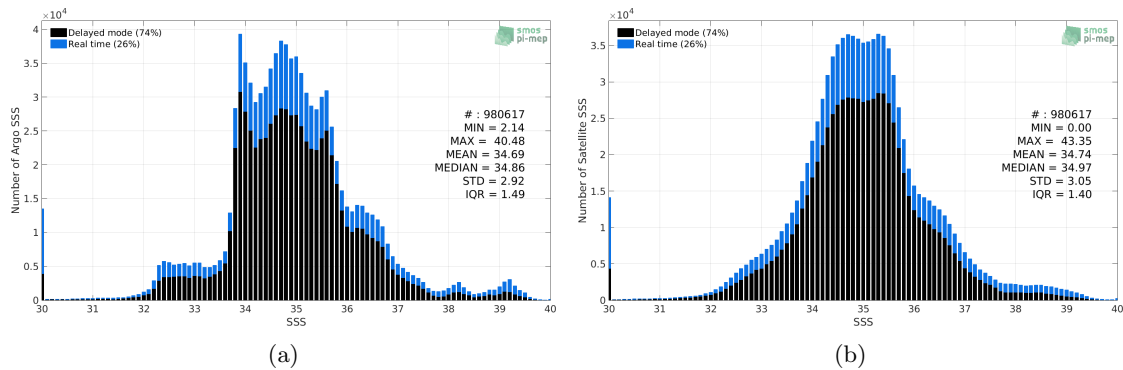
Figure 2: Histograms of SSS from Argo (a) and SMAP SSS L2-AVERAGED v5.0 (JPL) (b) considering all match-up pairs per bins of 0.1 over the Global Ocean Pi-MEP region and for the full satellite product period.
