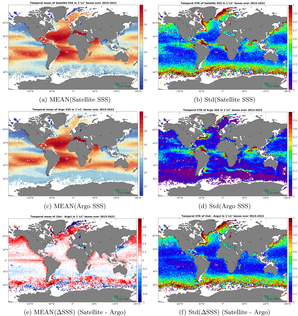
Figure 6: Temporal mean (left) and Std (right) of SSS from SMAP SSS L2-AVERAGED v5.0 (JPL) (top), Argo (middle), and of \Delta SSS (Satellite - Argo). Only match-up pairs are used to generate these maps.
