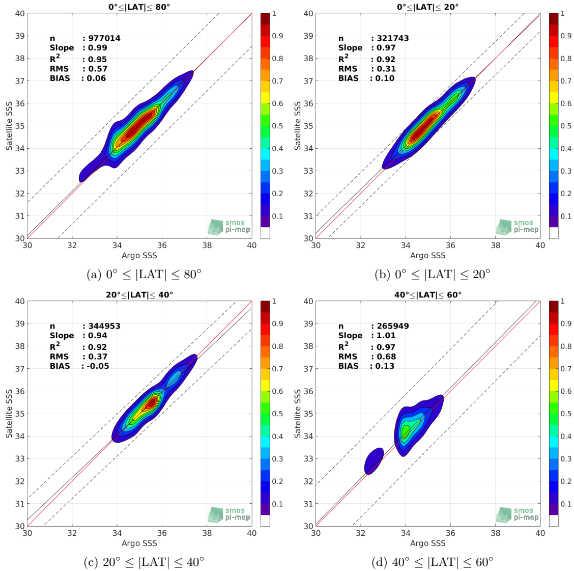
Figure 9: Contour maps of the concentration of SMAP SSS L2-AVERAGED v5.0 (JPL) SSS (y-axis) versus Argo SSS (x-axis) at match-up pairs for different latitude bands. For each plot, the red line shows x=y . The black thin and dashed lines indicate a linear fit through the data cloud and the \pm 95\% confidence levels, respectively. The number match-up pairs n , the slope and R^2 coefficient of the linear fit, the root mean square (RMS) and the mean bias between satellite and in situ data are indicated for each latitude band in each plots.
